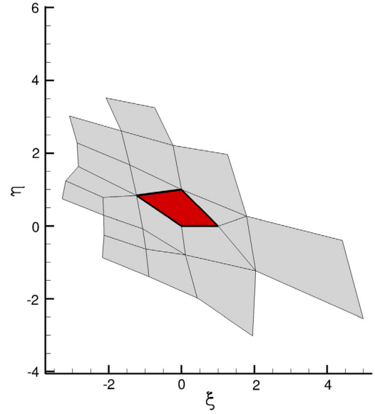
(b) Central stencil in reference space.
