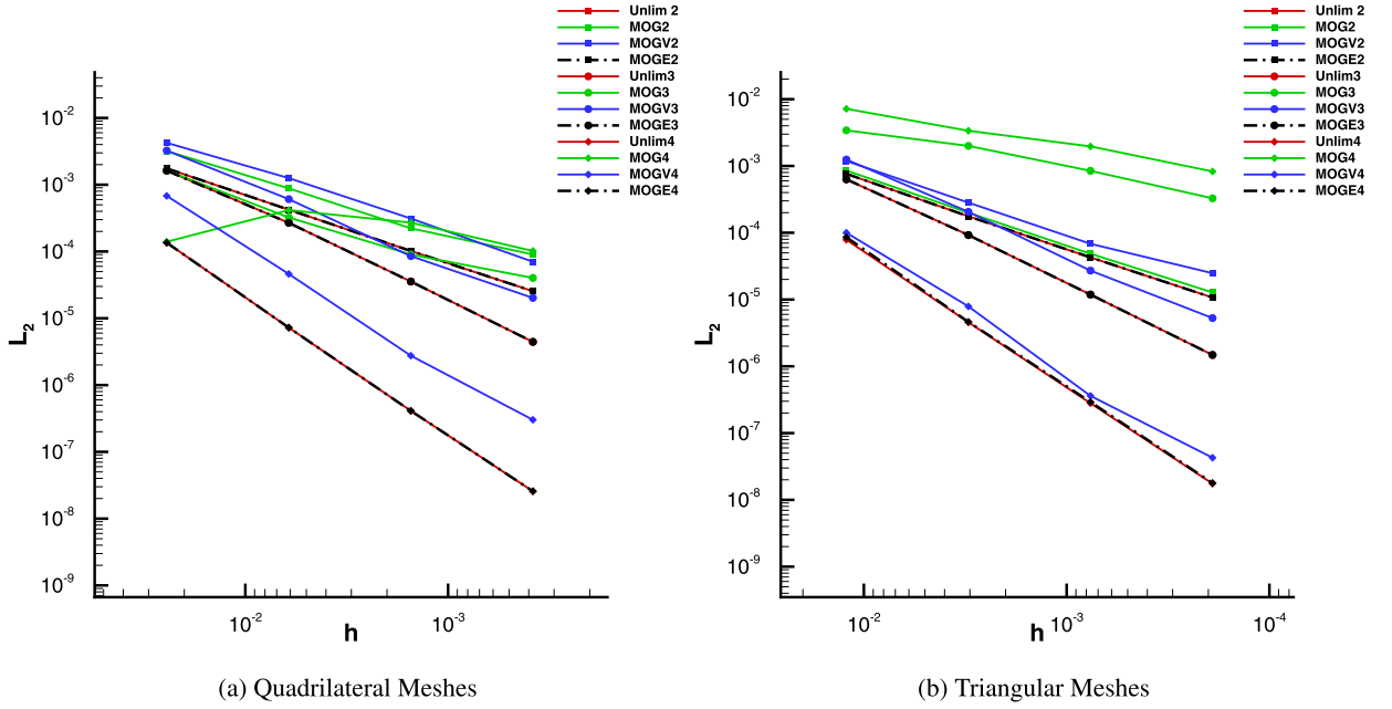
Fig. 8. L^2 convergence curves obtained with various numerical schemes on quadrilateral and triangular meshes for the 2D vortex evolution problem at t = 10 . (For interpretation of the colours in this figure, the reader is referred to the web version of this article.)
