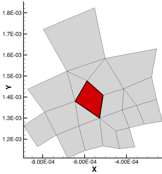
(a) Central stencil in physical space.
