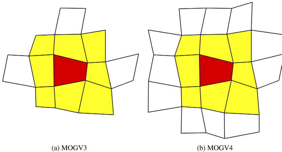
Fig. 6. Stencils for 3rd and 4th-order MOGV limiter, the \mathcal{M}_{\min} and \mathcal{M}_{\max} bounds are obtained from the yellow coloured elements and the considered cell in red colour. (For interpretation of the references to colour in this figure legend, the reader is referred to the web version of this article.)
