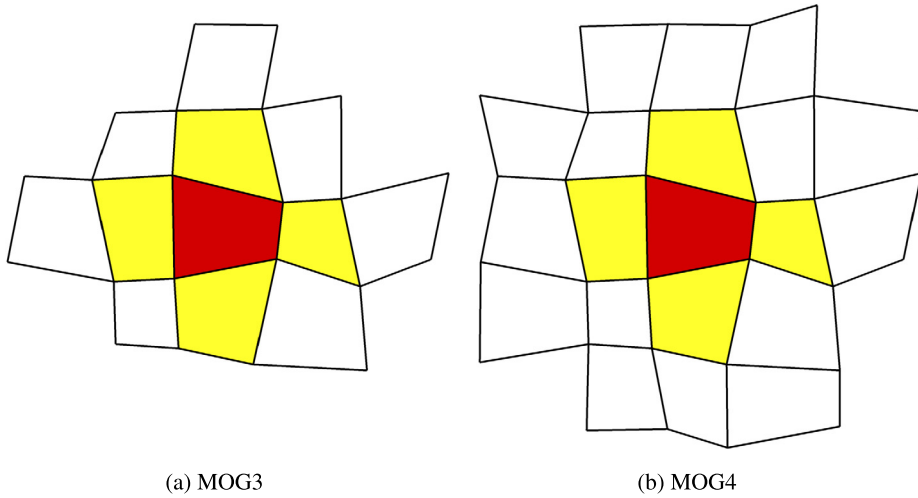
Fig. 5. Stencils for 3rd and 4th-order MOG limiter, the \mathcal{M}_{\min} and \mathcal{M}_{\max} bounds are obtained from the yellow coloured elements and the considered cell in red colour. (For interpretation of the references to colour in this figure legend, the reader is referred to the web version of this article.)
