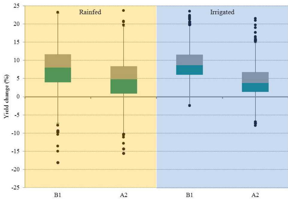
Figure 7 Projected yield changes (%) in rainfed (cv. Kilombero) and irrigated (cv. Puspa 33) rice for the 2050s, using three GCMs and two emission scenarios.
