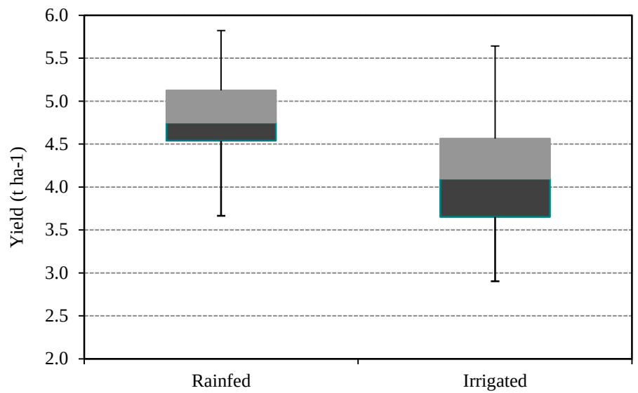
Figure 6 Simulated yield under the baseline (1961-1990) climatic conditions for rain-fed (cv. Kilombero) and irrigated rice (cv. Puspa 33) in the study area.
