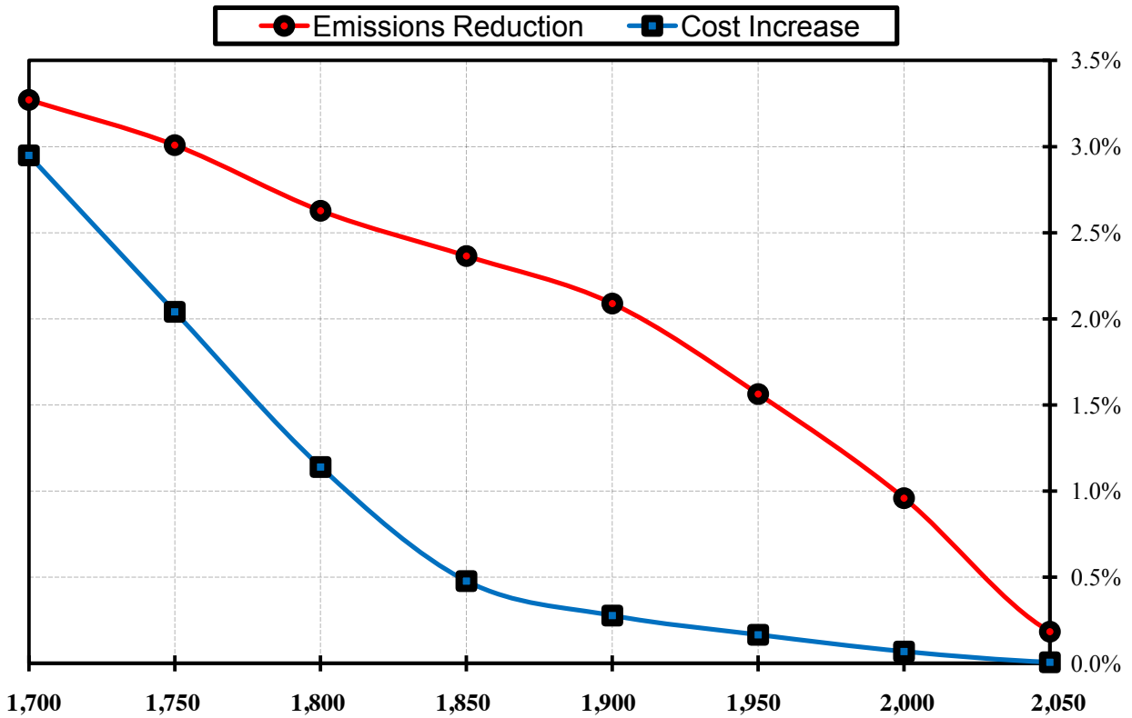
Figure 19. Total emissions reduction and cost increase under different emissions caps (with respect to the emissions unconstrained case, i.e., Case A).
