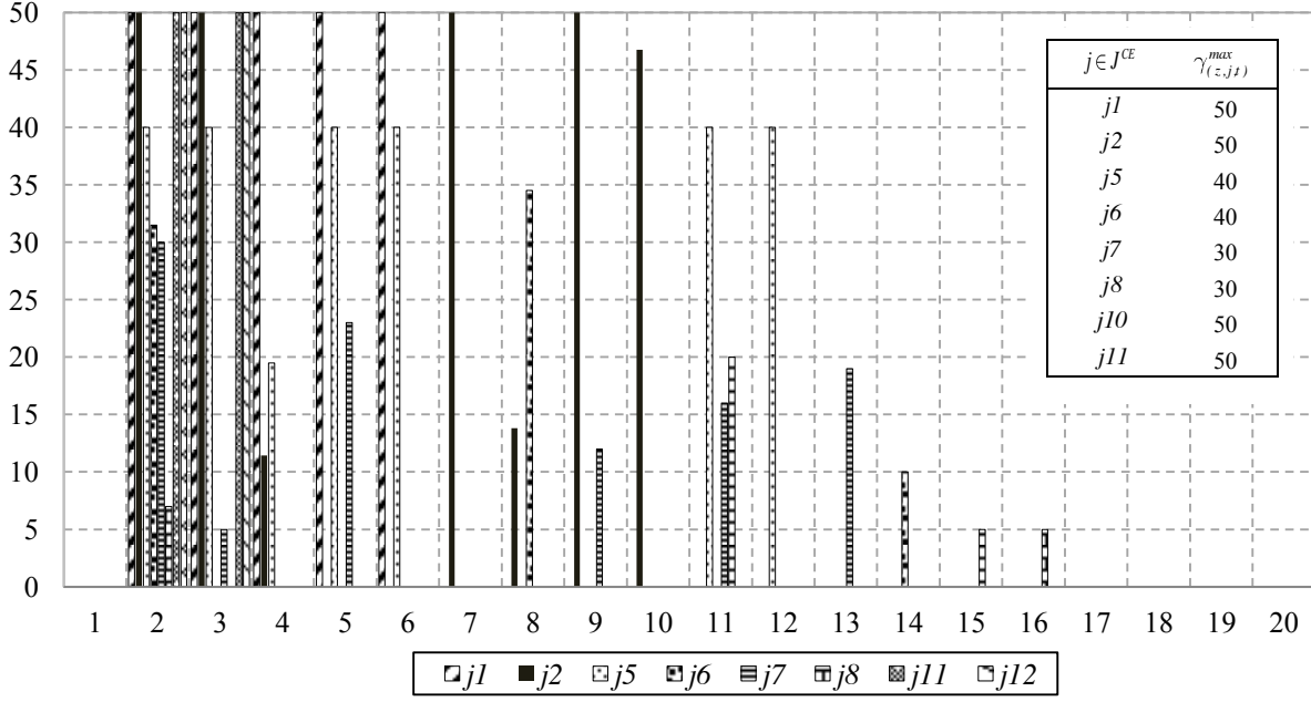
Figure 7. Case A: Capacity expansion for local exploitation and conversion technologies per time period.
