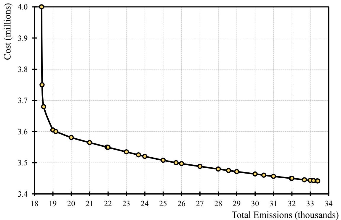
Figure 20. Multi-objective optimization: Pareto frontier for total emissions and cost.
