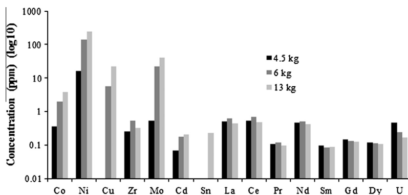
Fig. 6. Effect of bed inventory on increase of solid minor element concentrations for bed inventories of 4.5 kg, 6 kg and 13 kg \text{CaCO}_3 .
