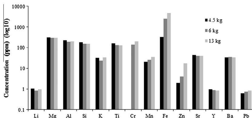
Fig. 4. Effect of bed inventory on increase of solid major elemental concentrations for bed inventories of 4.5 kg, 6 kg and 13 kg \text{CaCO}_3 .
