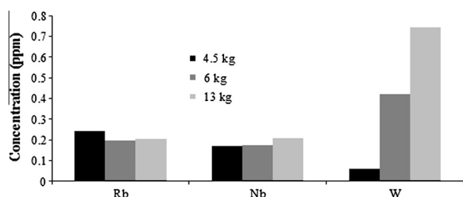
Fig. 7. Effect of bed inventory on increase of solid trace elemental concentrations, for bed inventories of 4.5 kg, 6 kg and 13 kg \text{CaCO}_3 .
