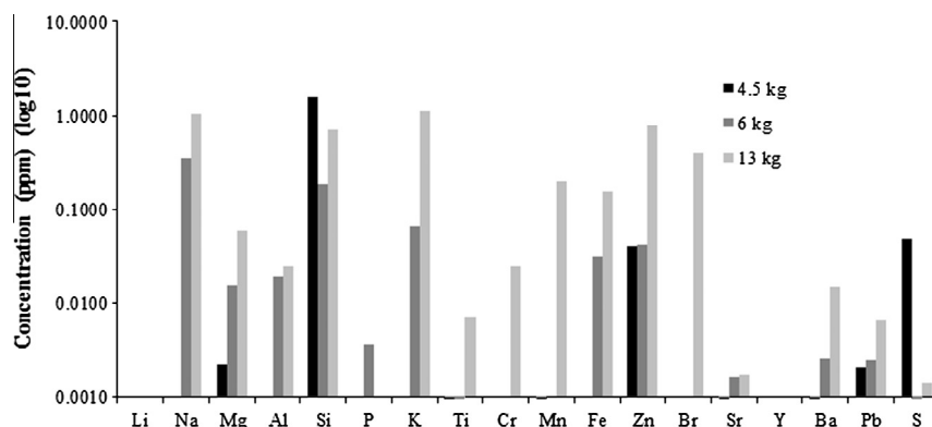
Fig. 5. Effect of bed inventory on increase of flue gas major elemental concentrations for bed inventories of 4.5 kg, 6 kg and 13 kg \text{CaCO}_3 .
