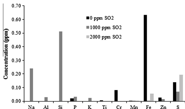
Fig. 10. Effect of \text{SO}_2 on increase of flue gas major elemental concentrations for \text{SO}_2 concentrations of 0 ppm, 1000 ppm and 2000 ppm, and bed inventory of 13 kg \text{CaCO}_3 .
