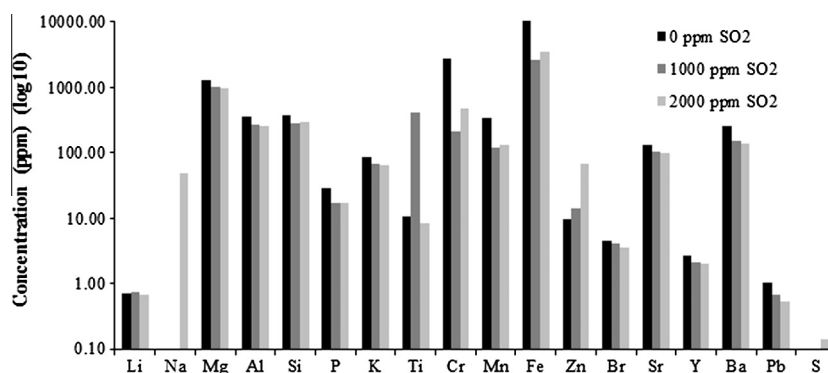
Fig. 9. Effect of \text{SO}_2 on (a) increase of solid major elemental concentrations for \text{SO}_2 concentrations of 0 ppm, 1000 ppm and 2000 ppm, and bed inventory of 13 kg \text{CaCO}_3 .
