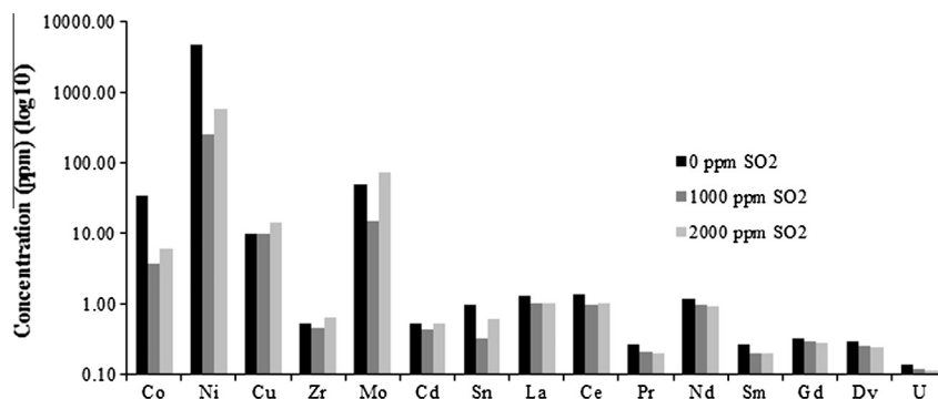
Fig. 11. Effect of \text{SO}_2 on (a) increase of solids minor elemental concentrations for \text{SO}_2 concentrations of 0 ppm, 1000 ppm and 2000 ppm, and bed inventory of 13 kg \text{CaCO}_3 .
