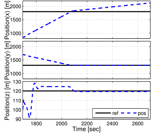
Fig. 12. Position tracking error of the first UAV after being disassembled in the integrated simulation
