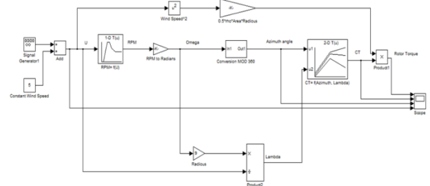
Figure 10. Rotor Simulink Model
