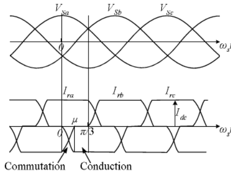
Figure 6. AC Voltage and Current waveforms
