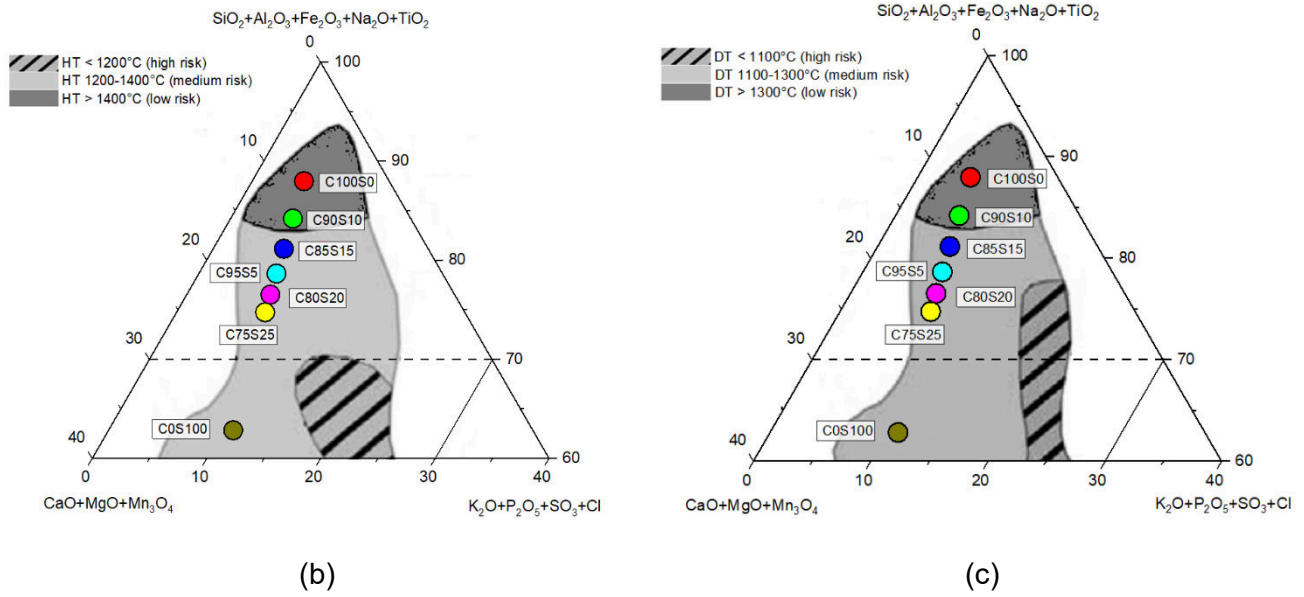
Fig. 2. Slagging risk estimation adopted from Vassilev et al. (Vassilev et al. 2014); (a) SCK diagram; (b) HT area; (c) DT area
