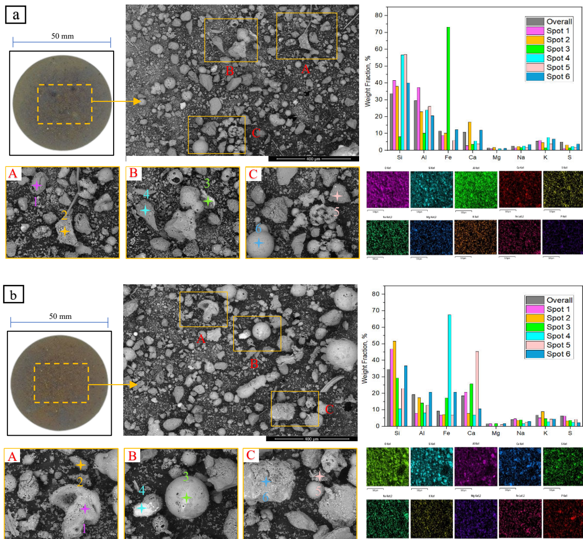
Fig. 8. BSE image with elements of C80S20 ash at the probe temperature of (a) 550 ^{\circ}\text{C} ; (b) 600 ^{\circ}\text{C}
