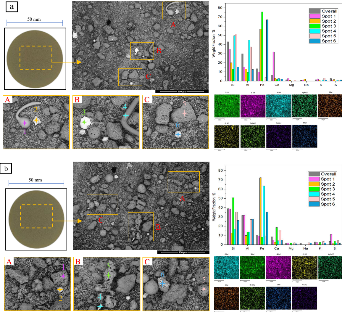
Fig. 4. BSE image with elements of C100S0 ash at the probe temperature of (a) 550 °C; (b) 600 °C
