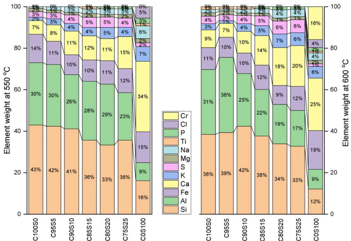
Fig. 11. Elemental composition comparison of ash deposits of tested samples
