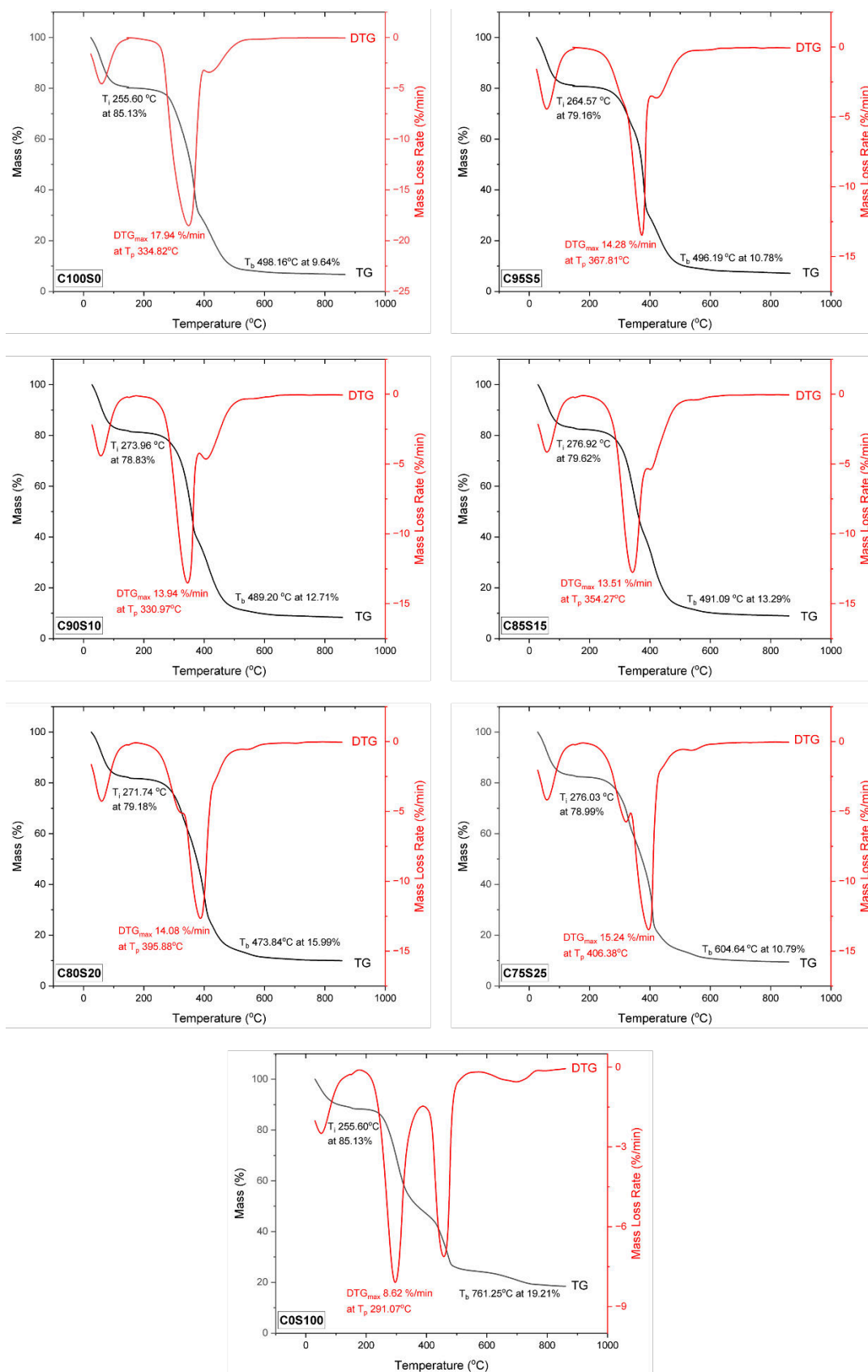
Fig. 2. TG and DTG curves of coal, SRF, and the blended
