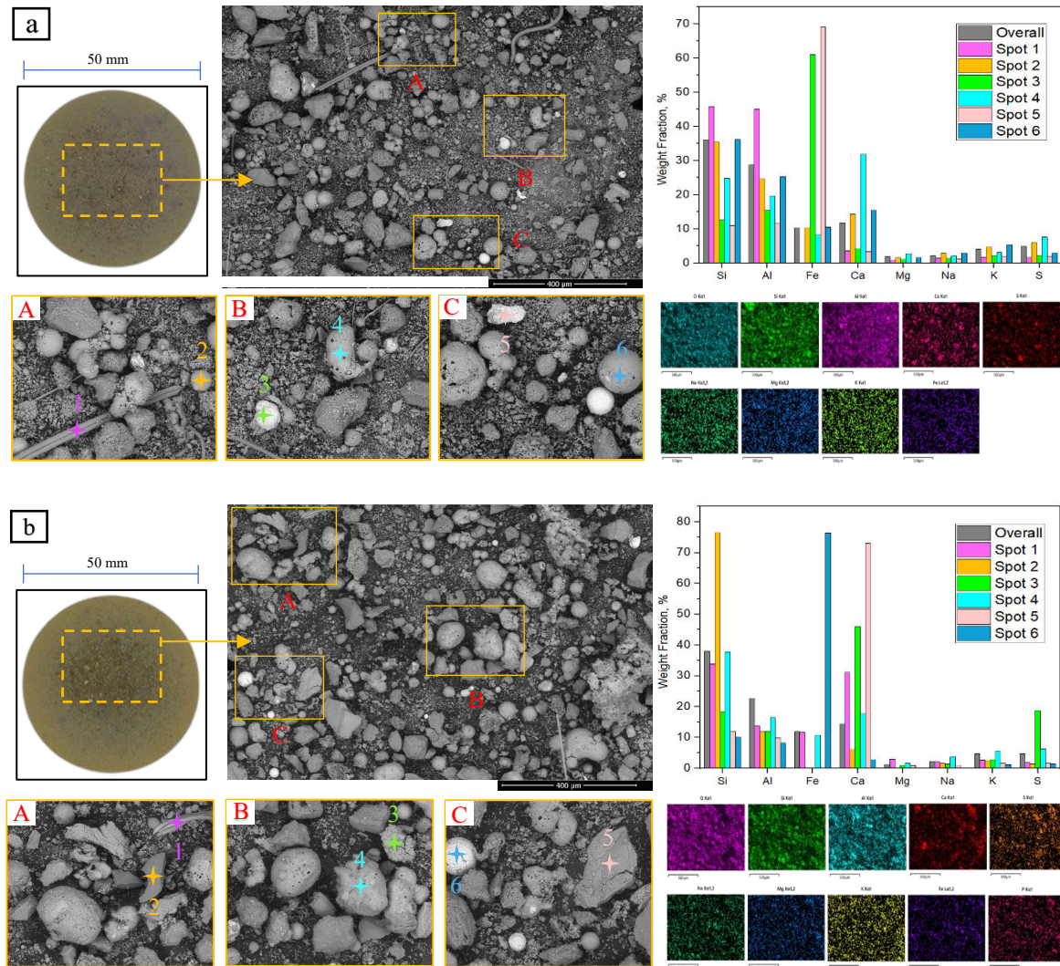
Fig. 7. BSE image with elements of C85S15 ash at a temperature of (a) 550 °C; (b) 600 °C
