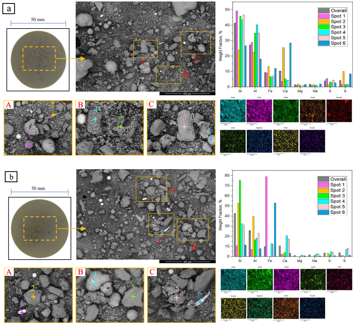
Fig. 6. BSE image with elements of C90S10 ash at the probe temperature of (a) 550 °C; (b) 600 °C
