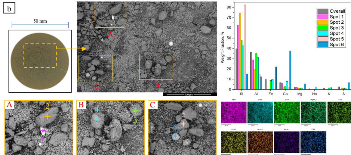
Fig. 5. BSE image with elements of C95S5 ash at the probe temperature of (a) 550 °C; (b) 600 °C
