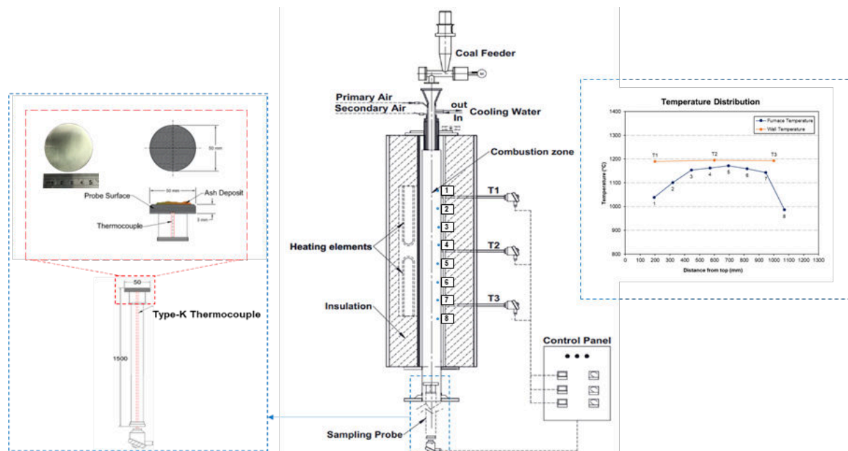
Fig. 1. Schematic diagram of laboratory-scale combustor (modified from (Karuana et al. 2024b))
