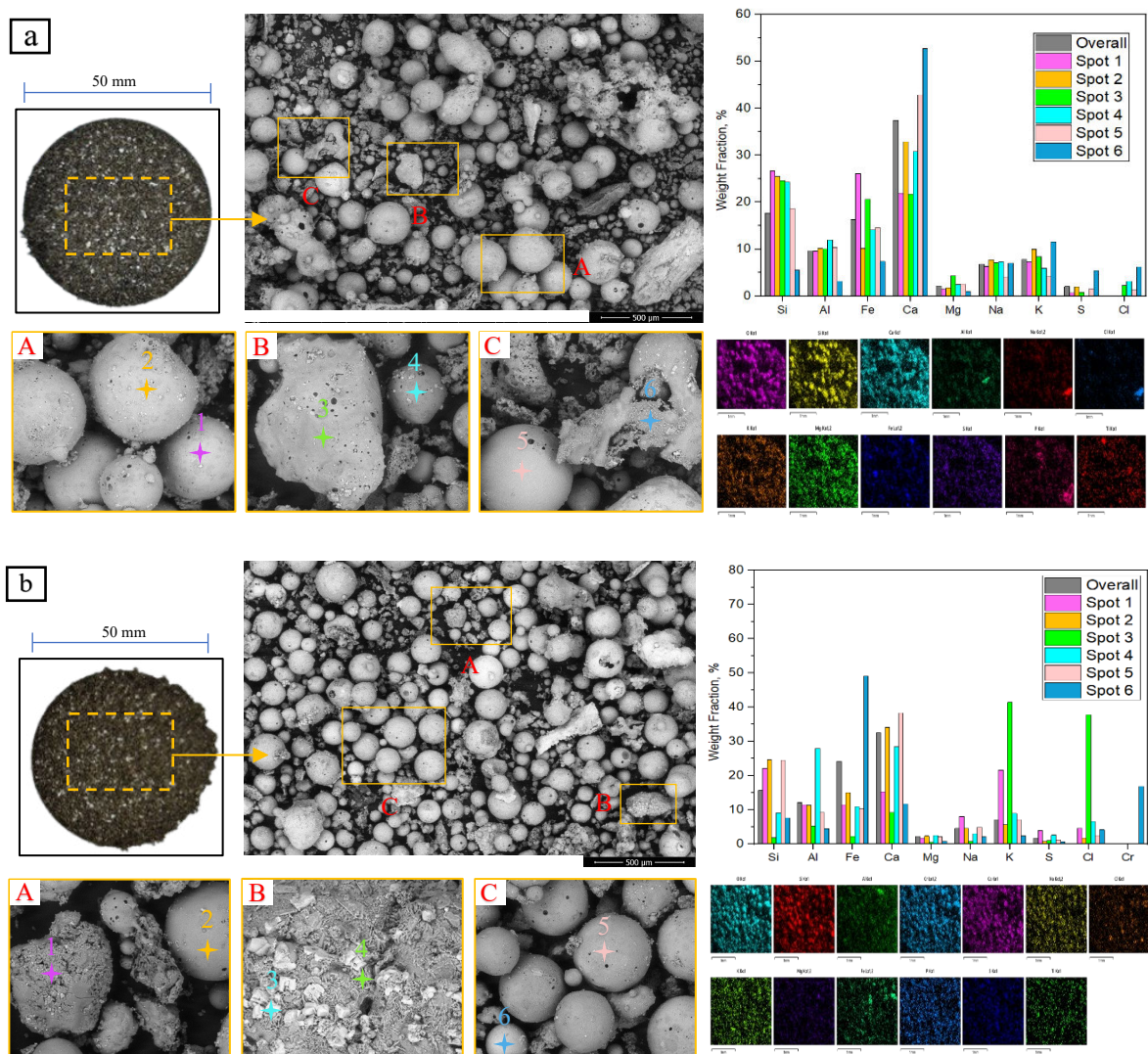
Fig. 10. BSE image with elements of C0S100 ash at a temperature of (a) 550 °C; (b) 600 °C
