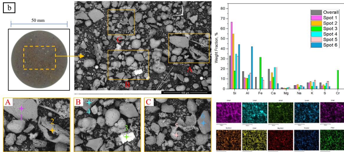
Fig. 9. BSE image with elements of C75S25 ash at a temperature of (a) 550 °C; (b) 600 °C
