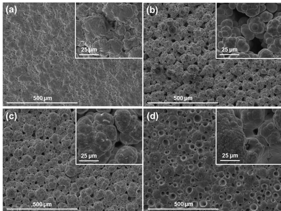
Fig. 4. SEM surface images with high magnification detail of Ni coatings produced with red brush and different current densities and CTAB concentrations: (a) 37 A/dm 2 and 3 g/l; (b) 75 A/dm 2 and 0.1 g/l; (c) 75 A/dm 2 and 0.5 g/l; (d) 75 A/dm 2 and 4 g/l.
