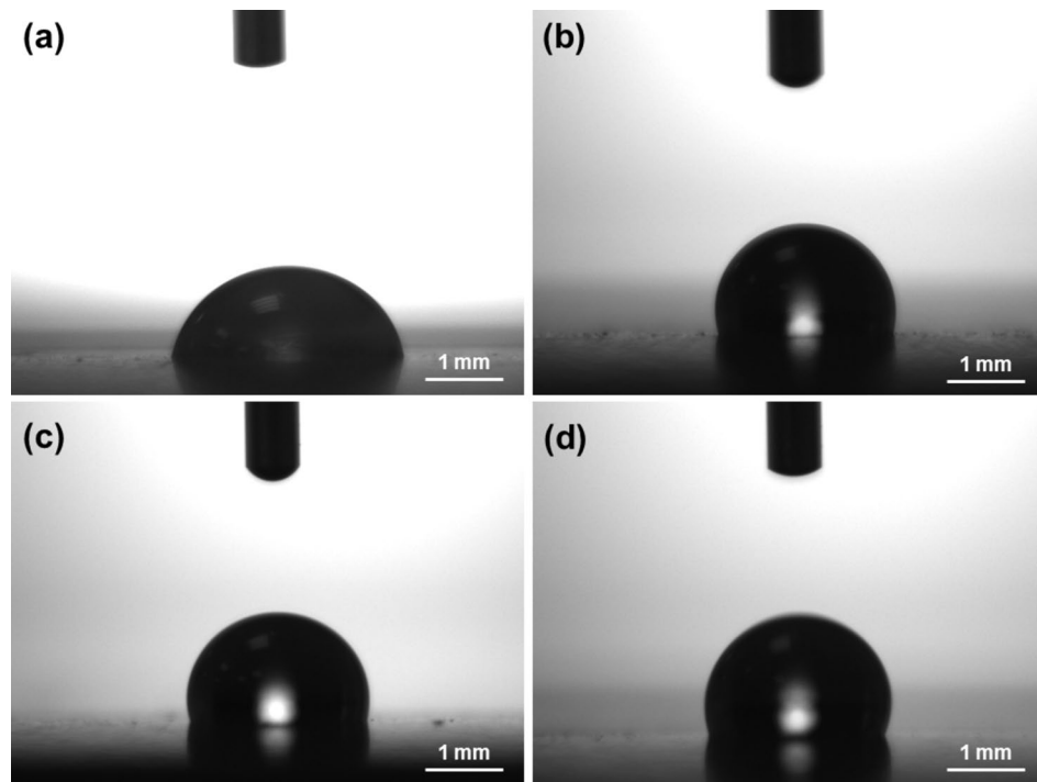
Fig. 8. Images taken during the measurement of the contact angle of a water droplet on the surface of different coatings: (a) Ni coating, (b) Ni/PTFE produced with IPA, (c) Ni/PTFE produced with ethanol, and (d) Ni/PTFE produced with ethanol interrupted at 5 A-min.
