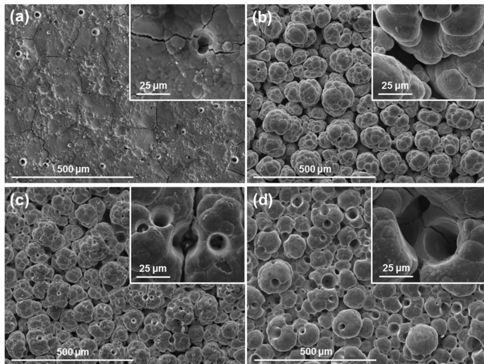
Fig. 3. SEM surface images with high magnification detail of Ni coatings produced with white brush and different current densities and CTAB concentrations of: (a) 37 A/dm 2 and 3 g/l; (b) 75 A/dm 2 and 0.1 g/l; (c) 75 A/dm 2 and 0.5 g/l; (d) 75 A/dm 2 and 4 g/l.
