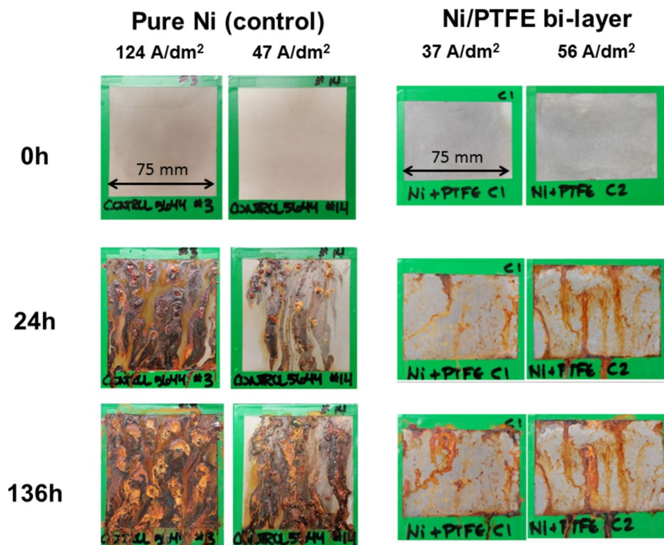
Fig. 9. Comparison of Ni and Ni/PTFE coating surfaces after salt spray testing for 136 h.
