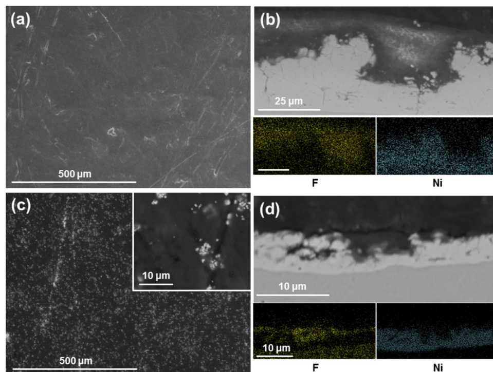
Fig. 6. SEM images and EDX mapping of Ni/PTFE coatings produced using ethanol as PTFE suspension agent, a current density of 37 A/dm 2 and white brush. (a) corresponds to a secondary electrons image of a thick coating surface, whereas (b) is a cross-section (BSE) of (a), together with EDX mapping of F (yellow) and Ni (blue). (c) is a thin coating surface (BSE), with (d) the cross-section (BSE) and EDX mapping of (c).
