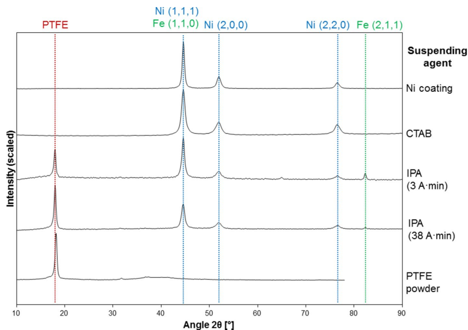
Fig. 7. XRD patterns of Ni and Ni/PTFE coatings corresponding, from top to bottom, to a pure Ni coating, a Ni coating produced from a PTFE suspension with CTAB, a Ni/PTFE coating produced with IPA at 3 A·min, a Ni/PTFE coating produced with IPA at 38 A·min, and as-received PTFE powder.
