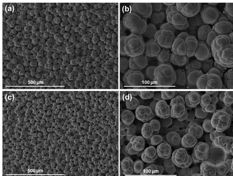
Fig. 1. SEM surface images of two pure nickel coatings deposited with a white brush material. (a,b) show two magnifications of a sample produced with a current density of 75 \text{ A/dm}^2 (c,d) correspond to a coating deposited at 124 \text{ A/dm}^2 .
