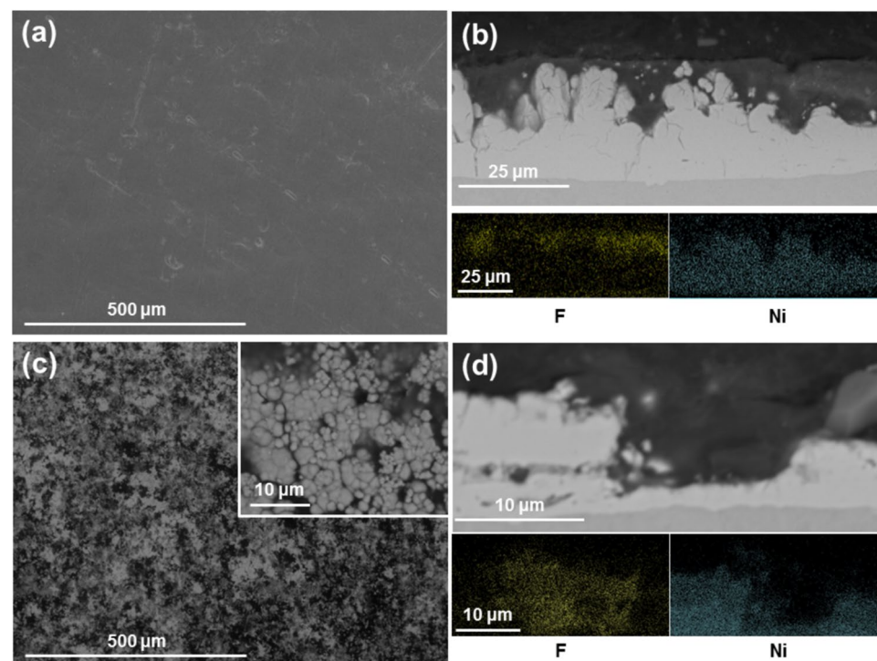
Fig. 5. SEM images and EDX mapping of Ni/PTFE coatings produced using IPA as PTFE suspension agent, a current density of 37 \text{ A/dm}^2 and white brush. (a) corresponds to a secondary electrons image of a thick coating surface, whereas (b) is a cross-section (BSE) of (a), together with EDX mapping of F (yellow) and Ni (blue). (c) is a thin coating surface (BSE), with (d) the cross-section (BSE) and EDX mapping of (c).
