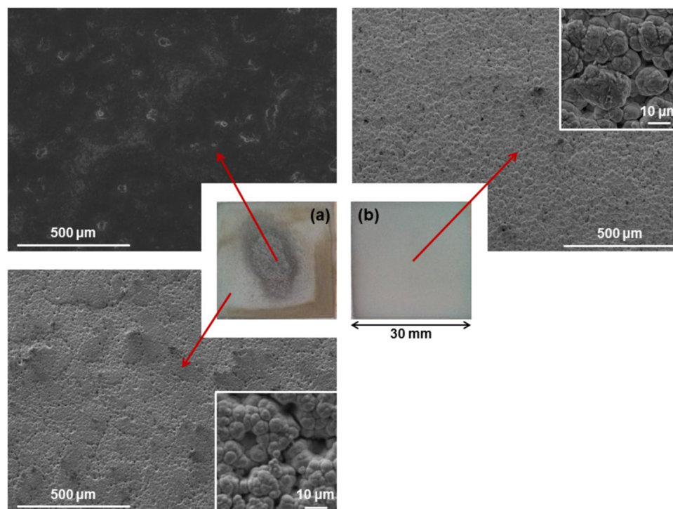
Fig. 2. Surface images from Ni/PTFE coating without the use of surfactants. In the centre, two macro images of the coatings, (a) produced with white brush and 124 \text{ A/dm}^2 current density and (b) produced with red brush and 75 \text{ A/dm}^2 . Around the edges, SEM images taken from the regions indicated with the red arrows are given with higher magnifications in the corners.
