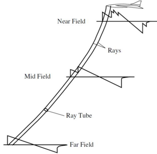
Fig. 3 Schematic of sonic boom propagation
