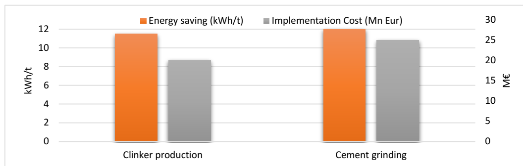
Figure 5 Energy saving (kWh/t) VS Cost (M€)
