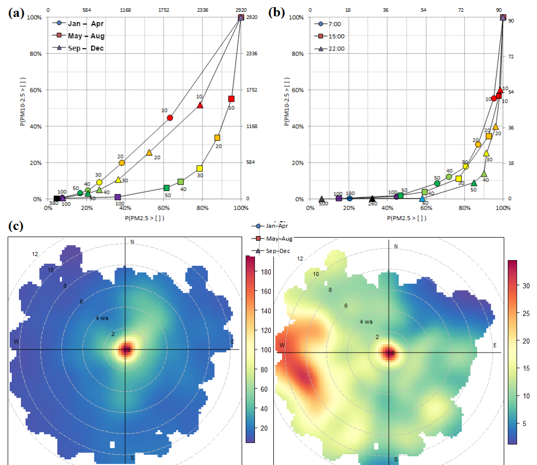
Figure 6. (a) Probability curves of fine PM and coarse PM concentrations for Coyhaique per periods of three months each. (b) Probability curves of fine PM and coarse concentrations in three different periods of the day during the cold season. The values within the graphs indicate the concentrations in \mu\text{g m}^{-3} . For each graph, secondary axes indicate the number of hours at which the concentrations exceeded. (c) Bivariate polar plot for mean concentration of \text{PM}_{2.5} by wind speed and direction. (d) Bivariate polar plot for mean concentration of coarse PM by wind speed and direction. For each polar plot, the radius was an indicator of wind speed ( \text{m s}^{-1} ) while the color showed the mean PM concentration.
