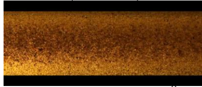
Figure 6: Sand transport condition for oil (340 cP at 16°C) and for 200 lb/1000 bbl, V_{Oil}=0.25\text{ m/s} (Bottom view)
