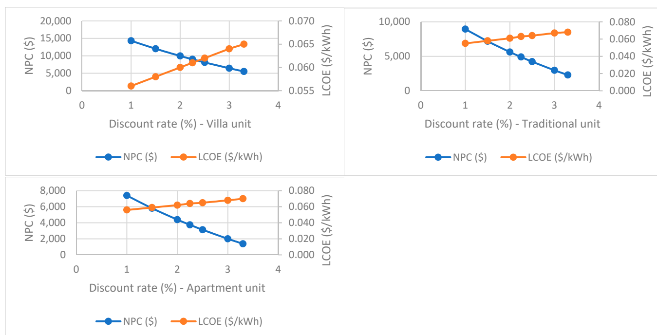
Figure 8. Effect of discount rate variability on NPC and LCOE for villa, traditional dwelling, and apartment.
