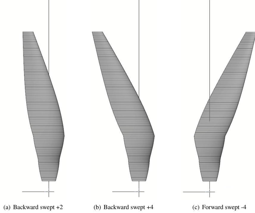
Fig. 3 Swept propeller blade geometries for three different sweep configurations; leading edge is on the right hand of each image
