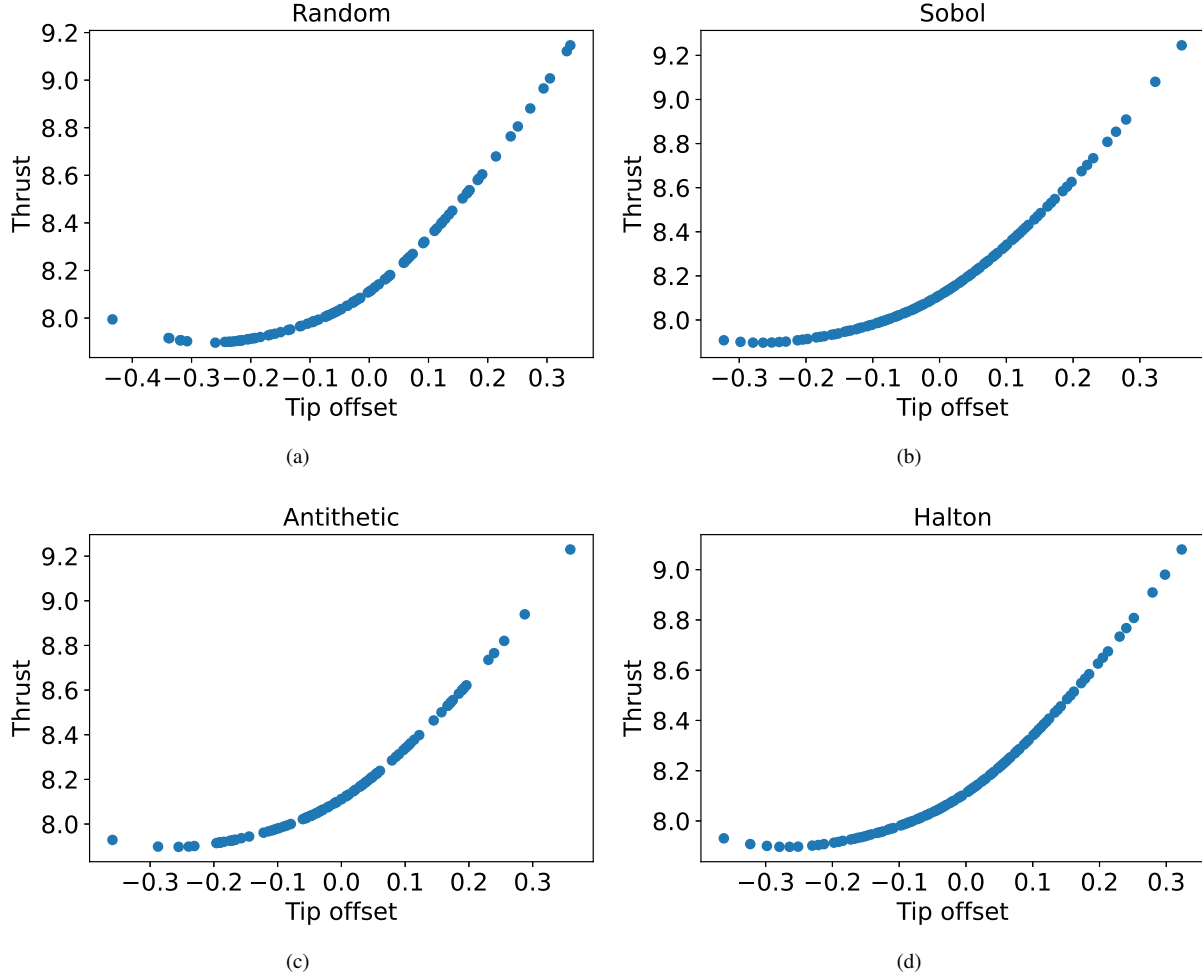
Fig. 11 Scatter plot for thrust values as predicted by the MFK method using various sampling methods, for 100 samples (as an example); mean is at tip offset = 0 with a standard deviation of 0.15; Thrust values are in N
