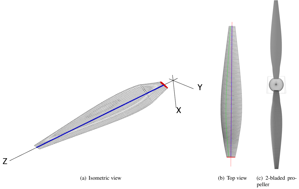
Fig. 1 Baseline propeller geometry, referred to as Sweep+0
