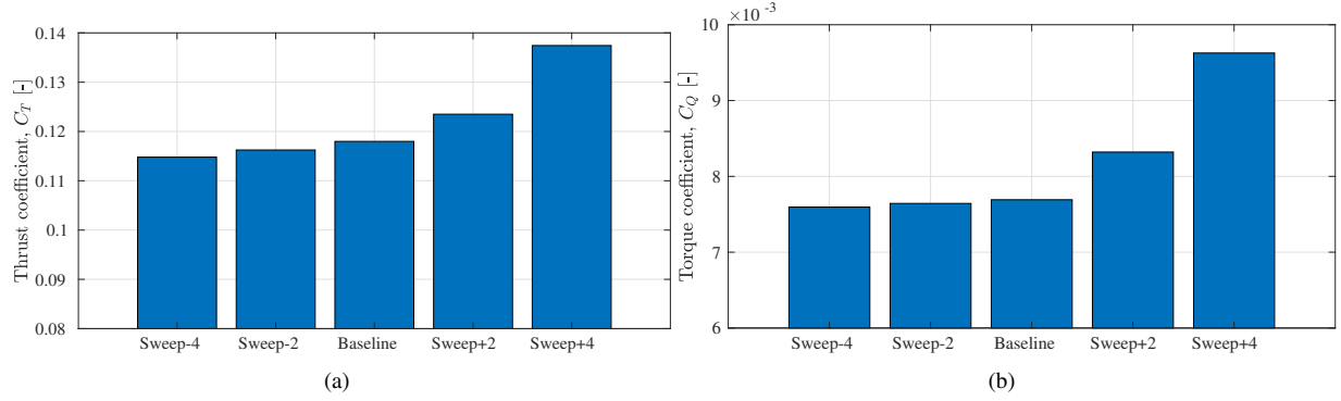
Fig. 7 Thrust coefficient C_T and torque coefficient C_Q comparison for different propeller blade sweep and the baseline propeller, using high-fidelity LBM
