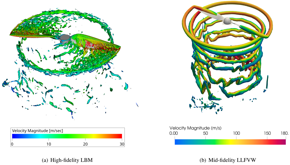
Fig. 8 Instantaneous 3D flowfield using iso-surfaces of the \lambda_2 criterion for vortices visualization for the baseline propeller
