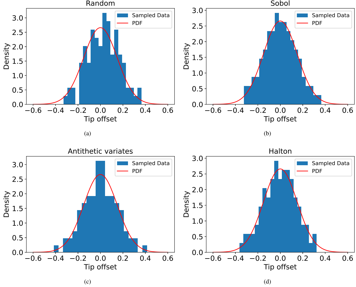
Fig. 10 Different sampling methods used in this study along with probability density function of the tip offset parameter for uncertainty quantification
