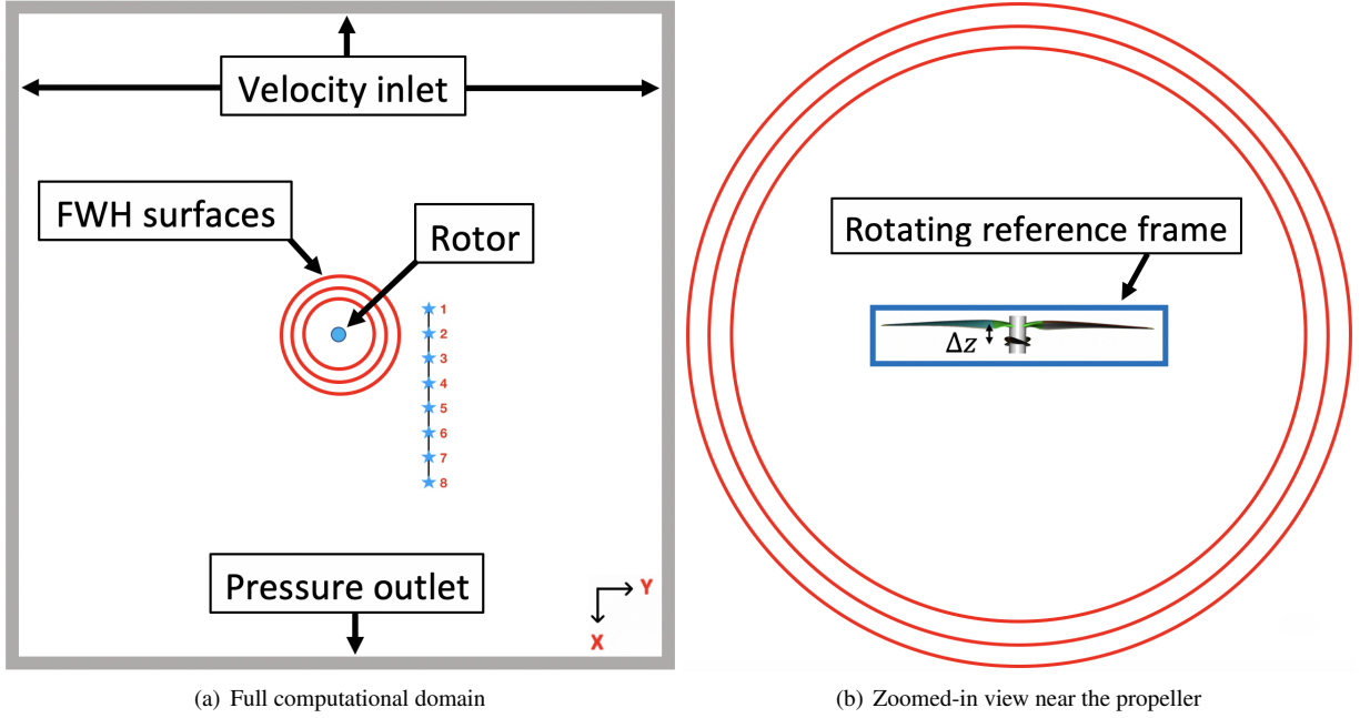
Fig. 4 Numerical setup (adapted from Shubham et al. [30, 81])
