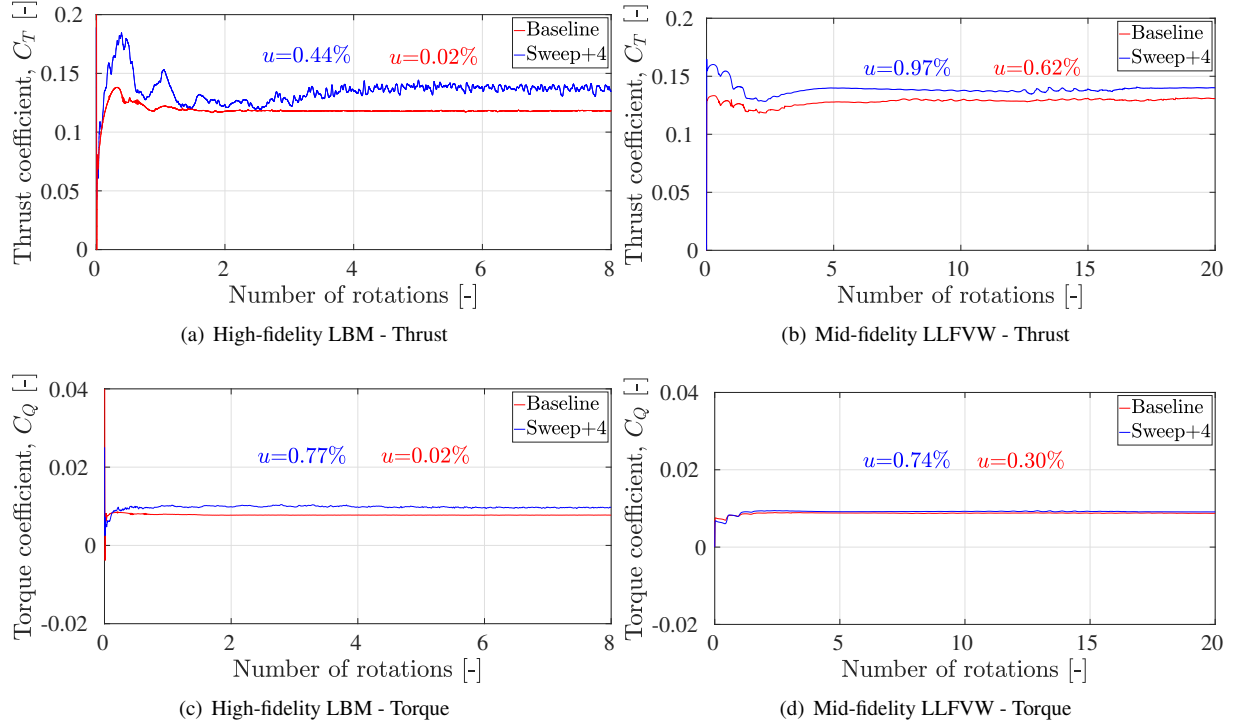
Fig. 6 Statistical temporal convergence study for thrust coefficient C_T and torque coefficient C_Q using high-fidelity LBM and mid-fidelity LLFVW
