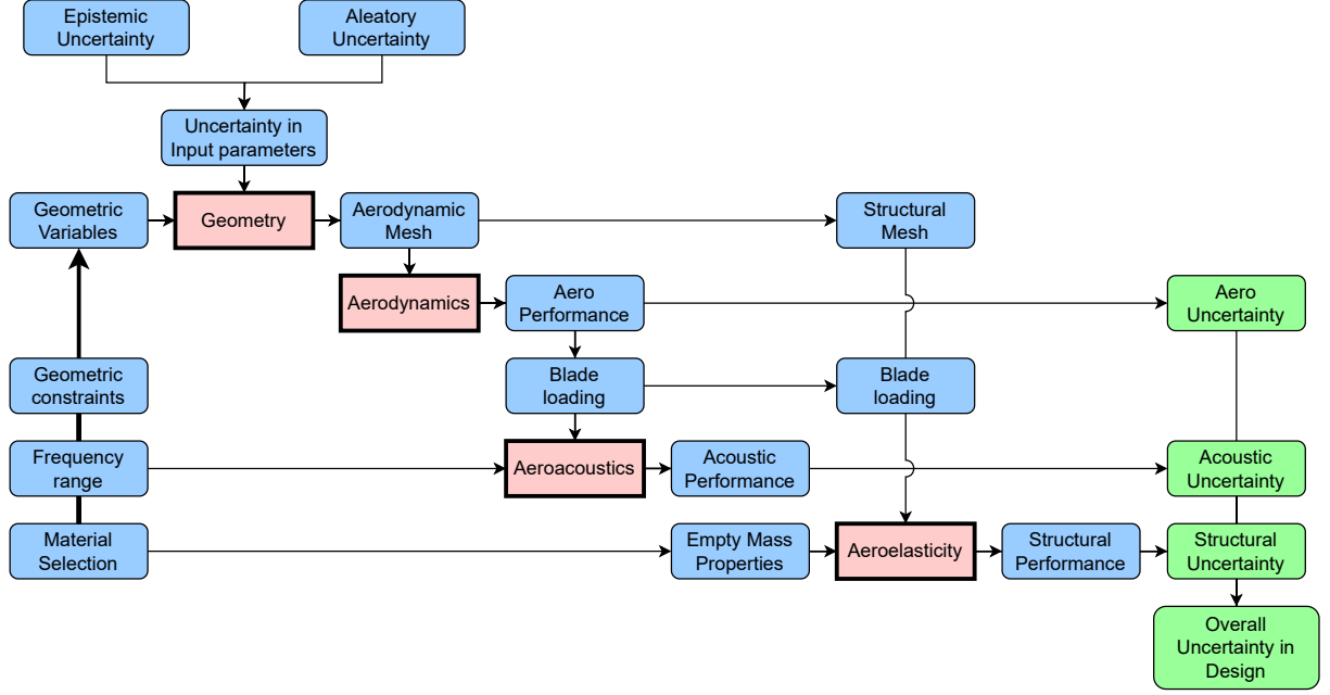
Fig. 5 Mixed Aleatory-Epistemic Uncertainty Propagation Framework
