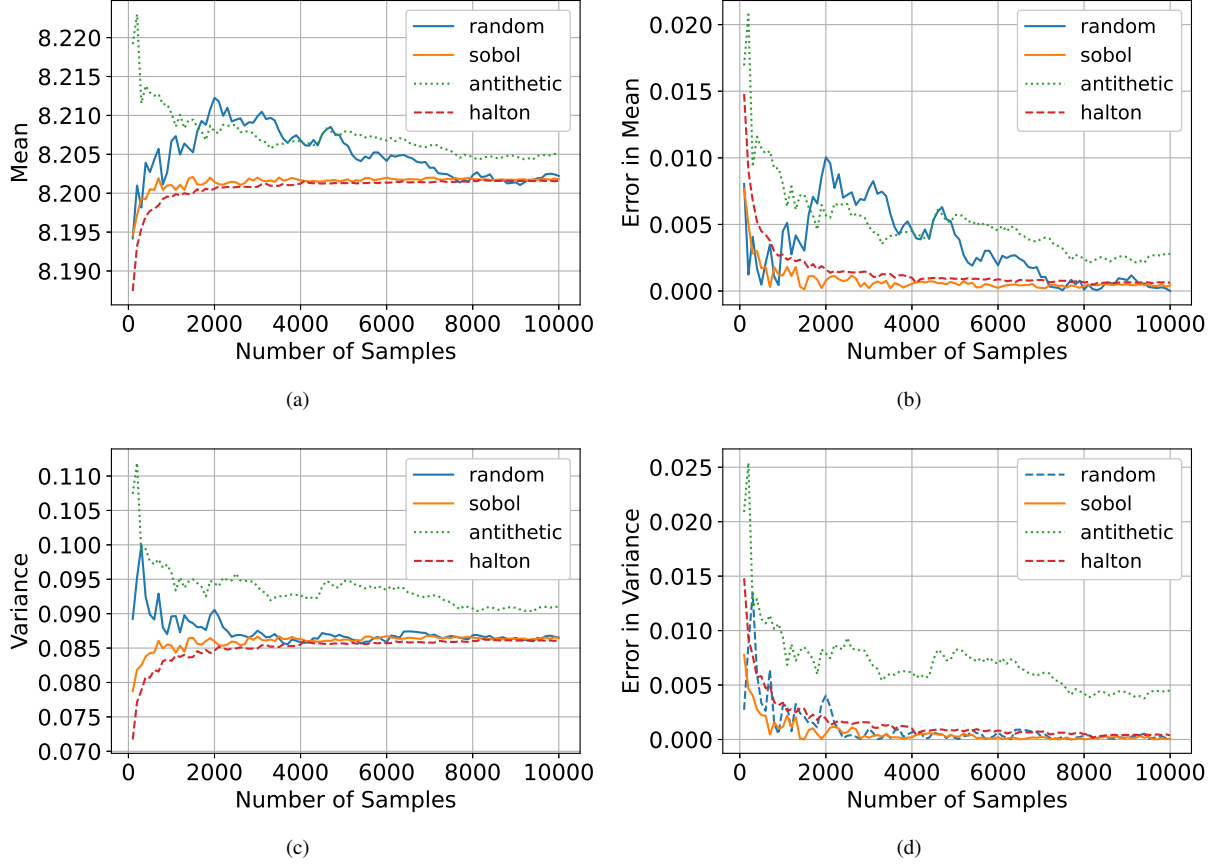
Fig. 12 Convergence behaviour of statistical metrics for thrust values obtained using four different sampling methods; y-axis of all sub-figures are in N
