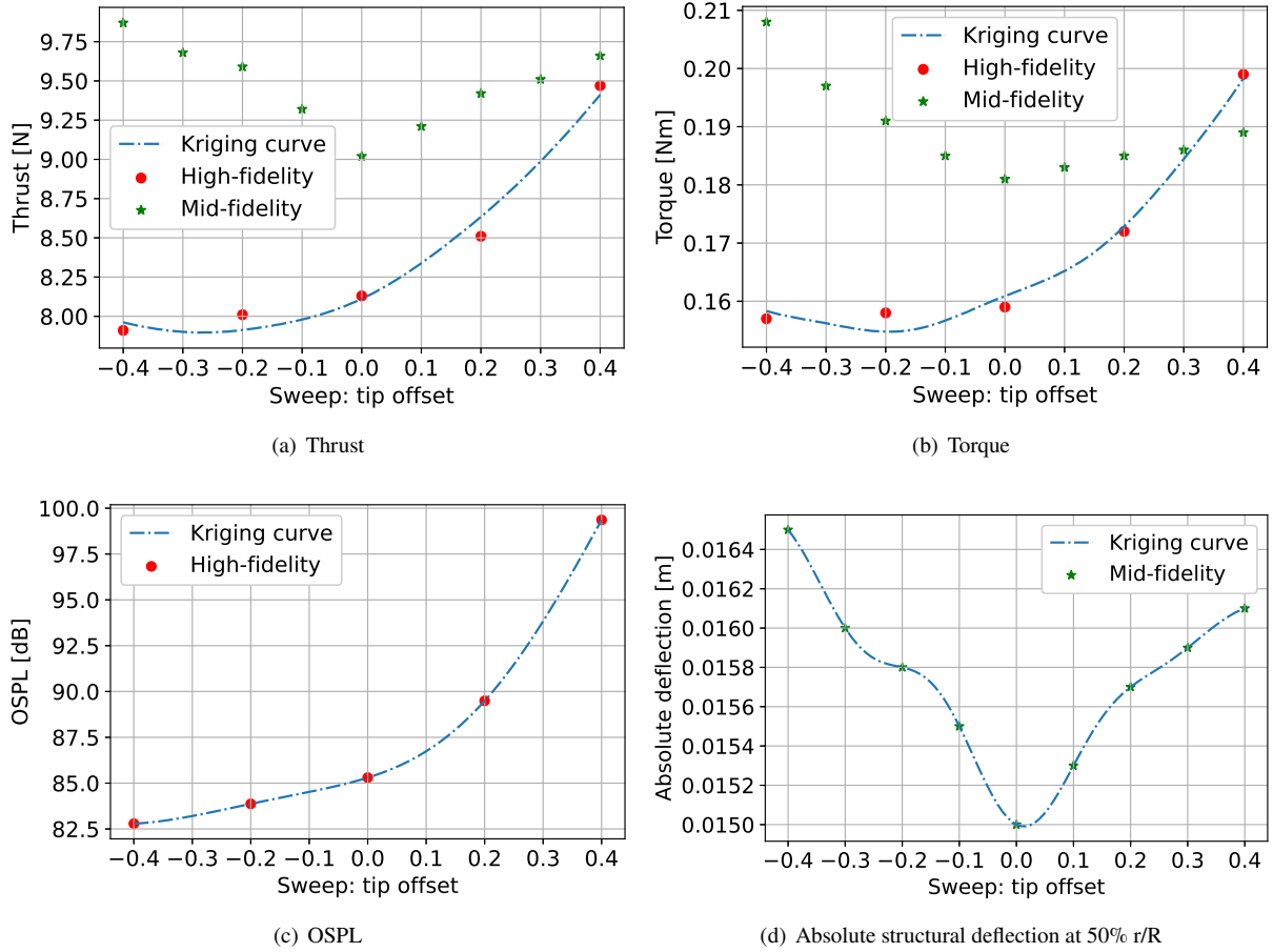
Fig. 9 Values obtained using both the mid and high-fidelity methods for different blade sweep defined by tip offsets and curve predicted using Kriging
