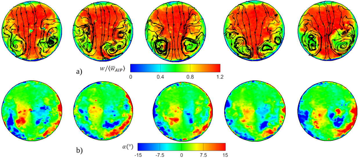
Fig. 19 VG5 configuration instantaneous out of plane velocity (a) and swirl angle (b) flow field from S-PIV M_{in}=0.27
