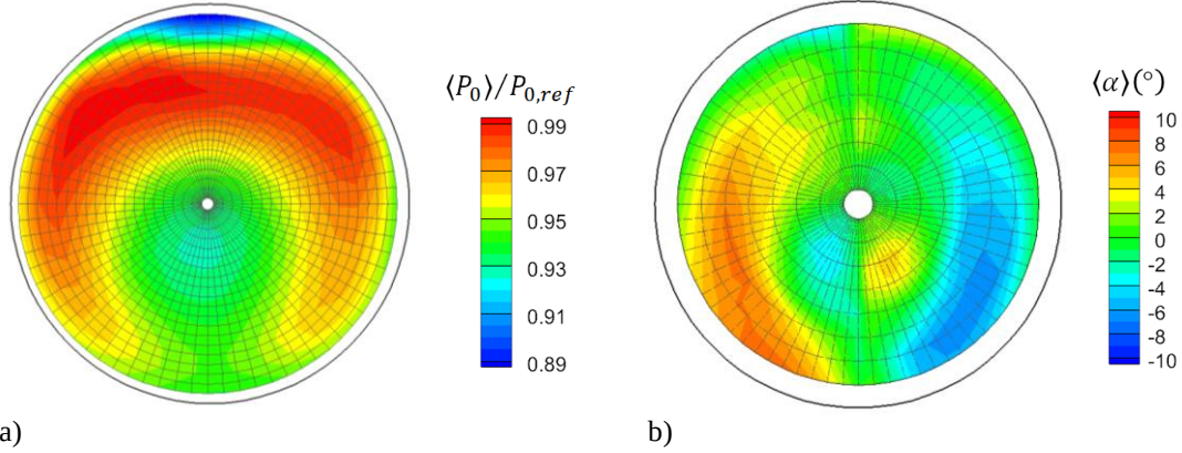
Fig. 8 Total pressure recovery (a) and swirl angle (b) field at the AIP for Min = 0.6
