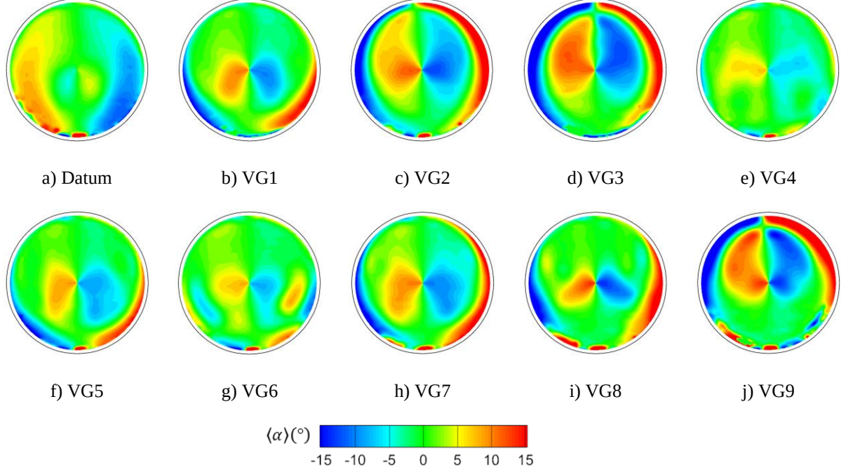
Fig. 13 Time averaged swirl angle from S-PIV at M_{in}=0.27
