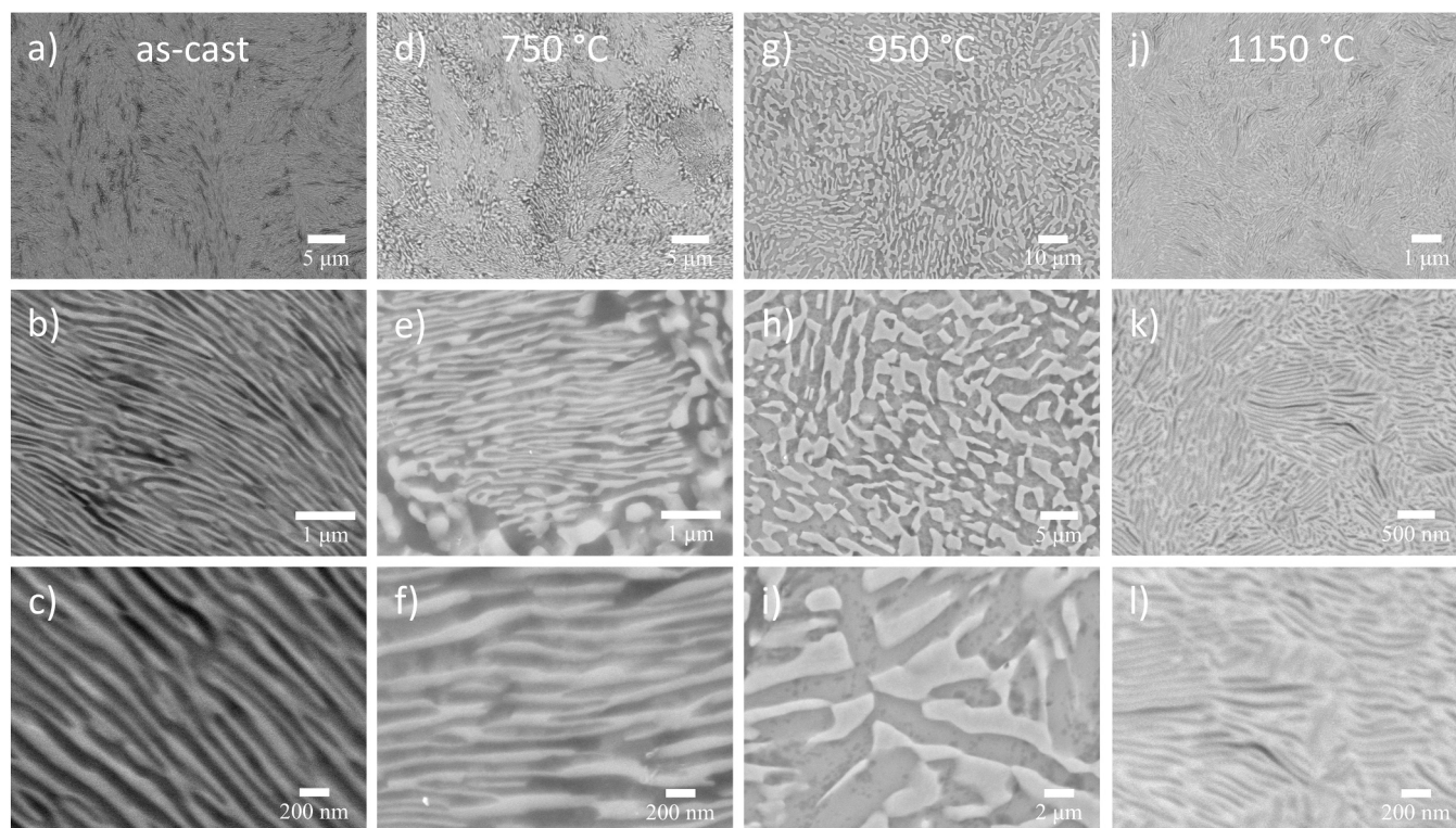
Fig. 8. SEM micrographs of surface-etched bulk \text{Ti}_{50}\text{Sc}_{50} (at%) alloys: (a–c) as-cast, and annealed for 4 h at: (d–f) 750 °C; (g–i) 950 °C; (j–l) 1150 °C.
