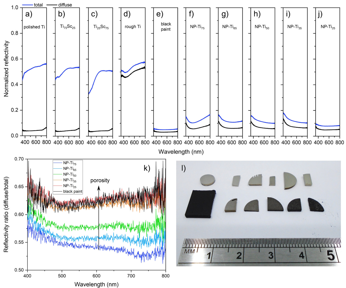
Fig. 6. Normalized total and diffuse reflectivities of: (a) polished bulk Ti; (b,c) bulk-cast Ti-rich and Sc-rich Ti-Sc alloys in the present work; (d) mechanically roughened bulk Ti; (e) matt-black paint; and (f-j) the NP-Ti alloys in the present work. Data over the full spectral range are given in Fig. S8. (k) Ratio of the diffuse to total reflectivity of NP-Ti samples compared to that of matt-black paint. (l) Photographs: top row: Ti (left) and bulk-cast Ti-Sc alloys (Sc at% increasing from left to right); bottom row: matt-black painted sample (left) and NP-Ti samples (porosity increasing from left to right).
