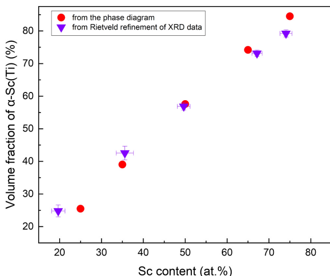
Fig. 2. The volume fraction of the \alpha -Sc(Ti) terminal solid solution in bulk-cast alloys estimated, as a function of overall Sc content in the alloy, by applying the lever rule to the phase compositions (Table S3). The volume-fraction values are supported by semi-quantitative Rietveld analysis of the XRD data (Fig. 1 and Table S1); the estimated standard deviations in these Rietveld-derived values are shown as vertical error bars.
