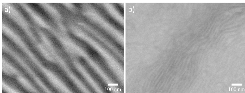
Fig. 7. Comparison of (a) bulk-cast and (b) suction-cast \text{Ti}_{50}\text{Sc}_{50} showing the finer lamellar microstructure in the latter case. The bulk-cast sample is more deeply etched than the suction-cast rod.
