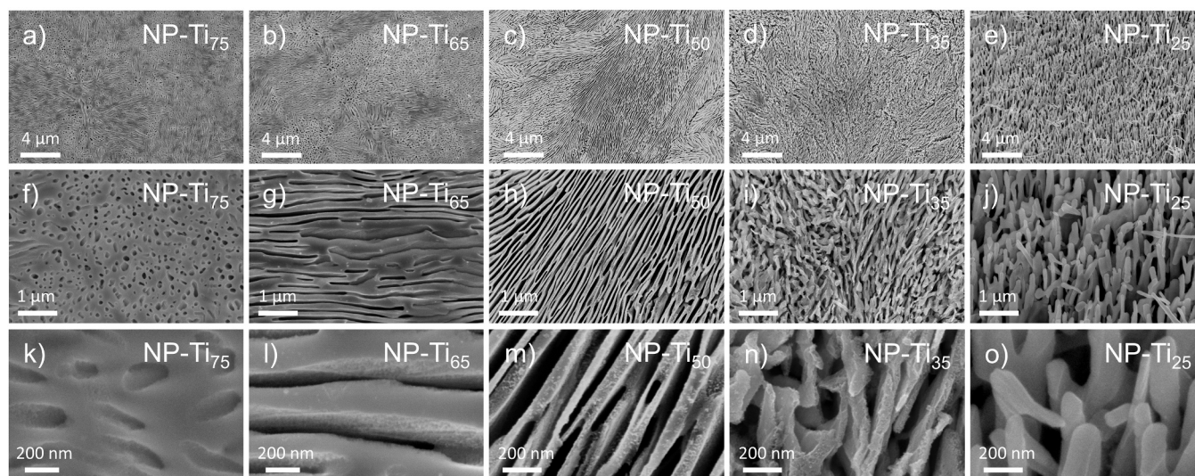
Fig. 3. SEM images of the nanoporous Ti produced by selective dissolution of the \alpha -Sc(Ti) phase from the Ti-Sc alloys (Ti content given in at%). (a–e) low, (f–j) intermediate, and (k–o) high magnification.
