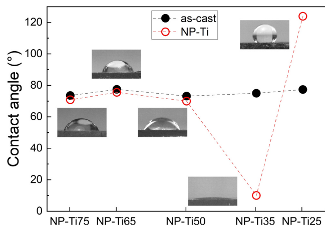
Fig. 5. The images show water droplets on NP-Ti prepared from the bulk-cast samples by selective dissolution. Droplets were also characterized on the corresponding as-cast Ti-Sc samples. Contact-angle values are compared for the as-cast samples (black solid circles) and the NP-Ti (red open circles).
