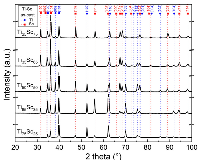
Fig. 1. X-ray diffractograms (CuK \alpha ) for bulk-cast samples of compositions (at %) from Ti 25 Sc 75 to Ti 75 Sc 25 . The peaks are indexed separately for the Ti-rich and Sc-rich terminal solid solutions.
