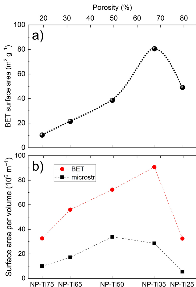
Fig. 4. Specific surface area (SSA) for the NP-Ti samples prepared from bulk-cast Ti-Sc alloys: (a) SSA per gram from BET measurements; (b) SSA per unit volume, from BET measurements and estimated from the microstructures of the samples.
