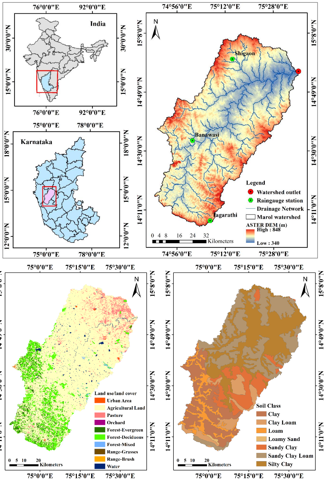
Figure 1: Study area description maps a) Location map, b) Land use/ land cover map and c) Soil map
