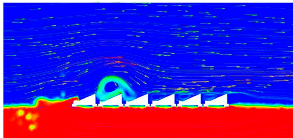
Figure 13. Wave-wind velocity streamlines [47].
