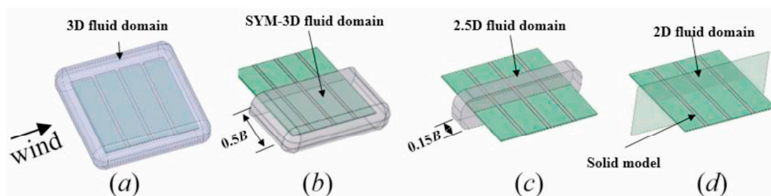
Figure 9. Fluid computational domains employed (a) 3D domain (b) 3D domain with symmetrical boundary condition (c) 2.5D Domain with reduced thickness (d) 2D domain [41].
