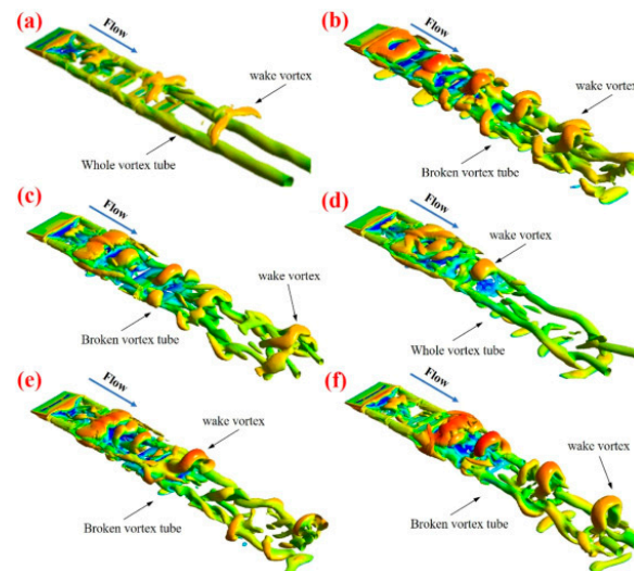
Figure 12. The vortex structure around the solar panel for arrangement in Figure 11b (a) array a (b) array b (c) array c (d) array d (e) array e (f) array f [37].
