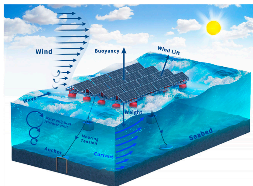
Figure 7. Loads on a Floating photovoltaic [35,36].
