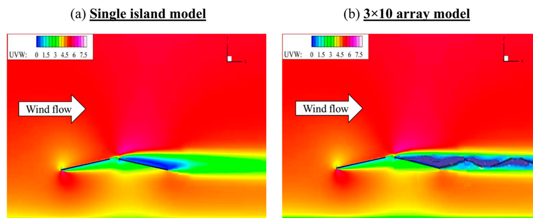
Figure 8. Flow visualisation of a (a) single FPV module and (b) FPV array [38].
