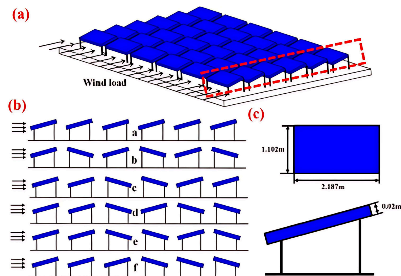
Figure 11. Arrangement of FPV panel (a) section of the FPV under consideration (b) six arrangement types (c) Dimensions of the photovoltaic [37].
