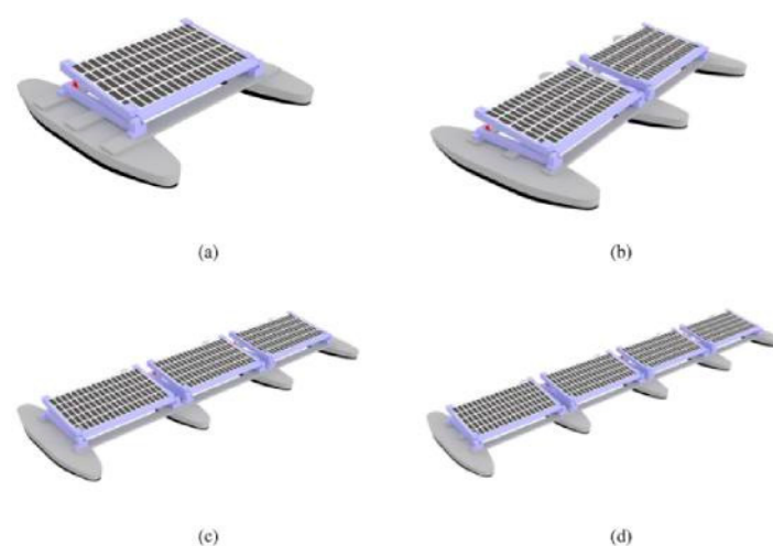
Figure 17. Catamaran Platform for FPVs (a) catamaran, (b) trimaran, (c) quadrimaran, (d) pentamaran. [60].
