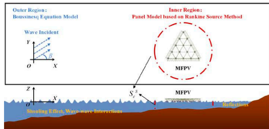
Figure 18. Computational methodology of HBPM [72].
