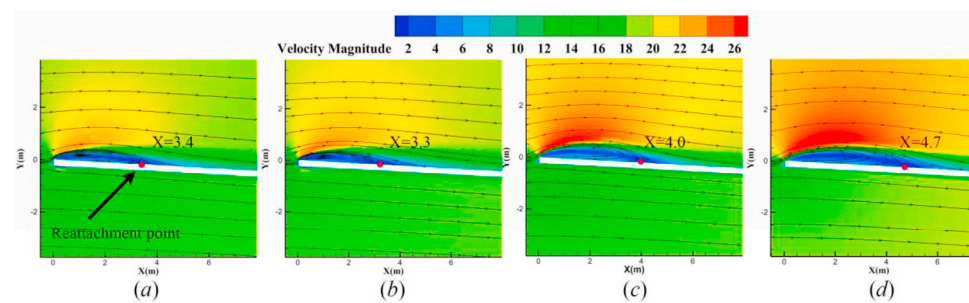
Figure 10. Velocity distribution and streamlines around the leading edge from (a) 3D, (b) SYM-3D, (c) 2.5D and (d) 2D fluid computational domains [41].
