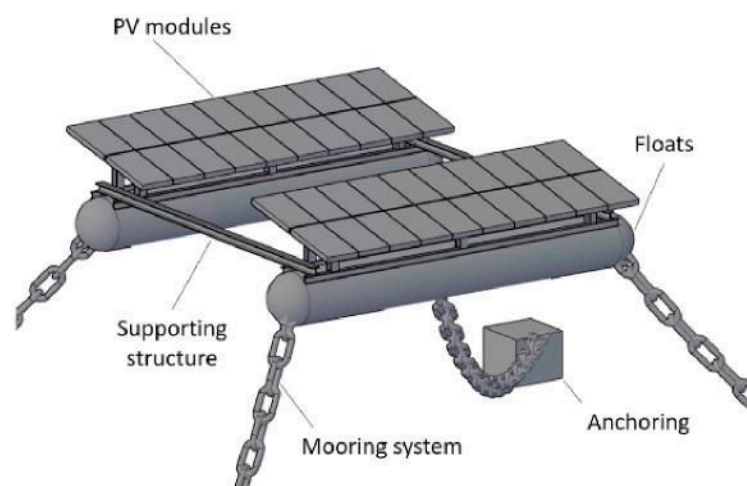
Figure 2. Components of an FPV system [25].
