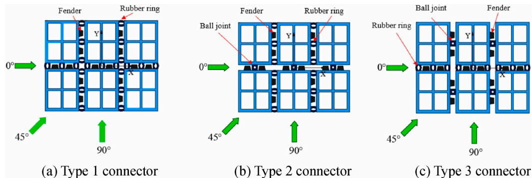
Figure 15. Schematic of connectors (a) Type 1 connector (b) Type 2 connector (c) Type 2 connector [61].
