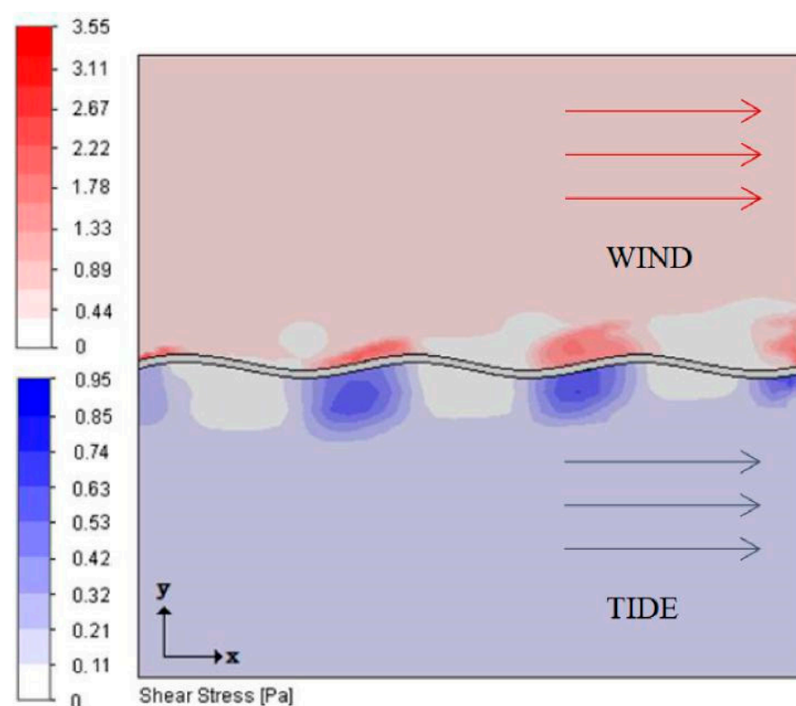
Figure 14. Shear stress on a thin film PV subject to wind and wave loads [53].
