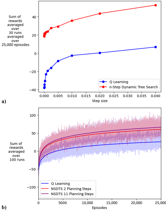
Fig. 5 n -step dynamic tree search performance against Q -learning temporal-difference method: a) step size analysis, and b) algorithm performance with optimal learning rates through averaged sum of rewards.
