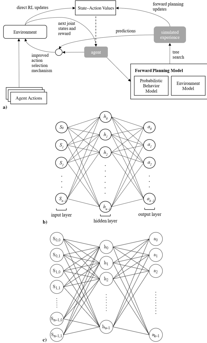
Fig. 3 NSDTS system overview from an individual agent perspective (Fig. 3a), probabilistic behavior model for stochastic prey study (Fig. 3b), and probabilistic behavior model for intelligent prey study (Fig. 3c).
