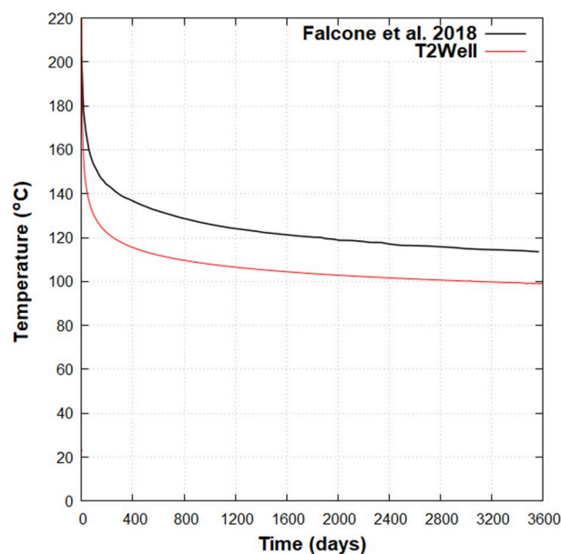
Fig. 4 Numerical results comparison from Falcone et al. (2018) and the T2Well/EOS1 model
