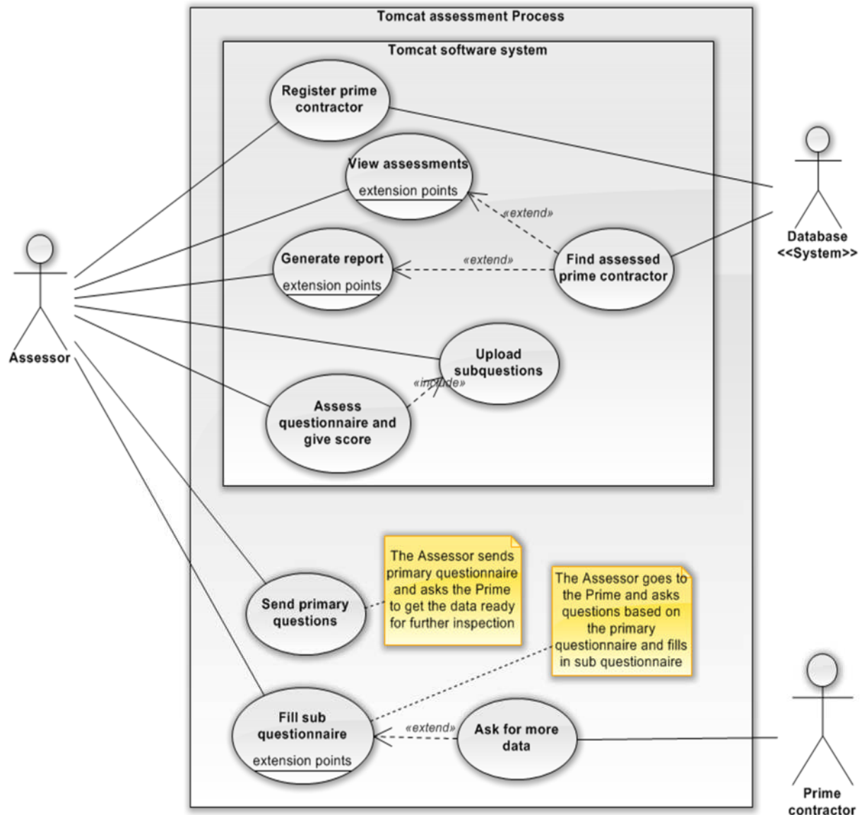
Figure 4. Unified Modelling Language (UML) Diagram of TOMCAT Process
