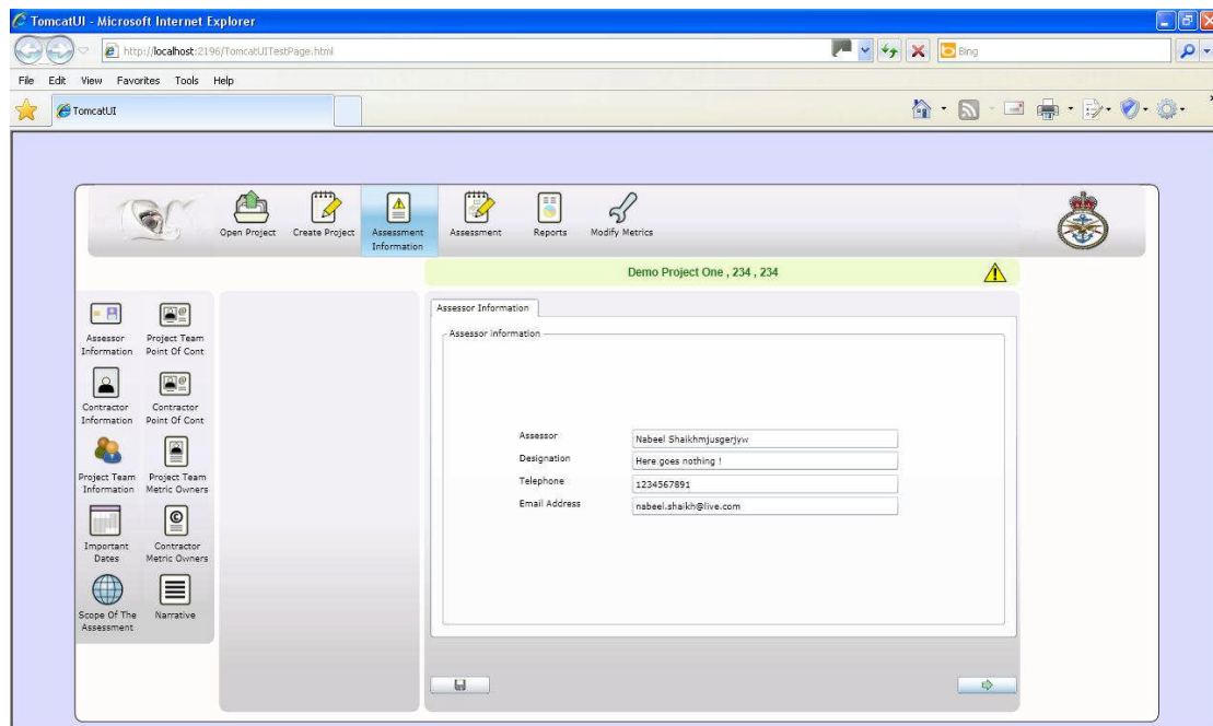
Figure 6. Snapshot of Assessment data input in TOMCAT
