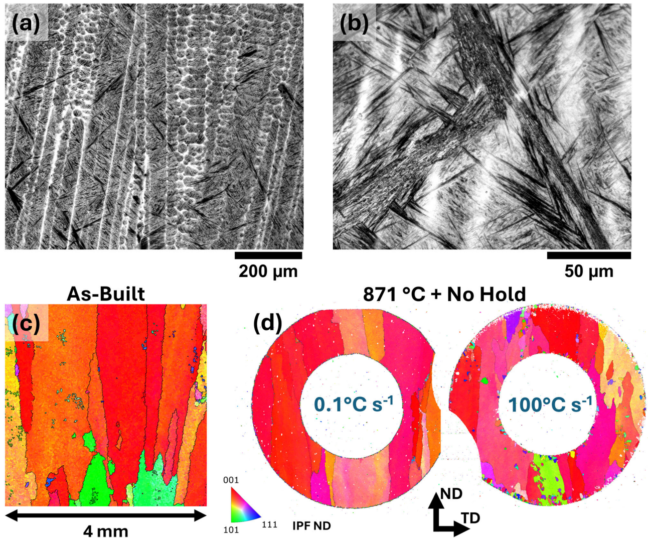
Fig. 3—(a) and (b) Optical micrographs of the 300 M wall in the as-built condition after nital etching, at (a) low magnification and (b) higher magnification. (c) An EBSD PAG reconstruction of the as-built 300 M microstructure. (d) EBSD PAG reconstructions of the 300 M dilatometry sample cross-sections heated to 871 °C and immediately quenched, at slow and fast heating rates, respectively.
