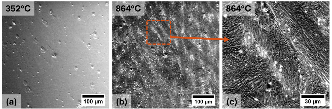
Fig. 9—(a) and (b) SE images of the Test 1 in-situ EBSD region at 352 °C and 864 °C, respectively, showing particle evolution in enriched areas. (c) Magnified view of the boxed region in (b).
