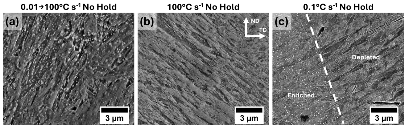
Fig. 6—SE images from etched 300 M dilatometry samples (bold in Table III) heated to 871 °C (a) using the 0.01 → 100 °C s -1 heating profile (b) at 100 °C s -1 and (c) at 0.1 °C s -1 . All three samples were immediately quenched after reaching 871 °C.
