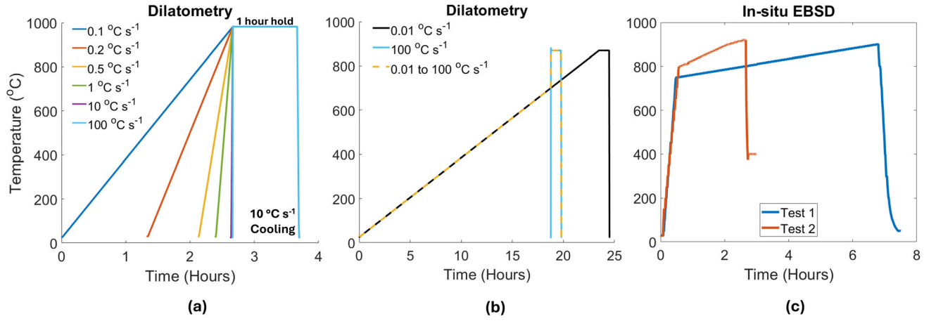
Fig. 2—(a) and (b) Example temperature profiles used for the dilatometry experiments with holds. Samples were heated to their respective austenitisation temperature (871 °C for 300 M and 982 °C for C465) with one of 6 different heating rates. The yellow dashed profile was performed for 300 M only. (c) The temperature profiles used for the two 300 M in-situ EBSD experiments (Color figure online).
