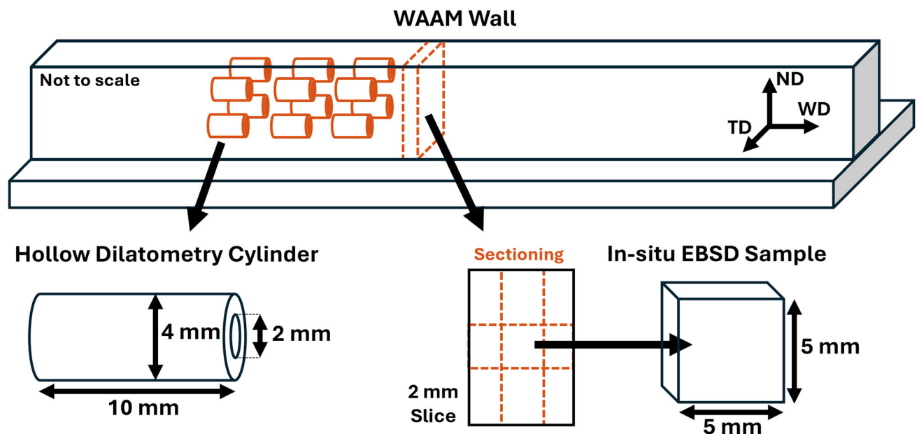
Fig. 1—A schematic displaying how the dilatometer and in-situ EBSD samples were machined from the WAAM walls.
