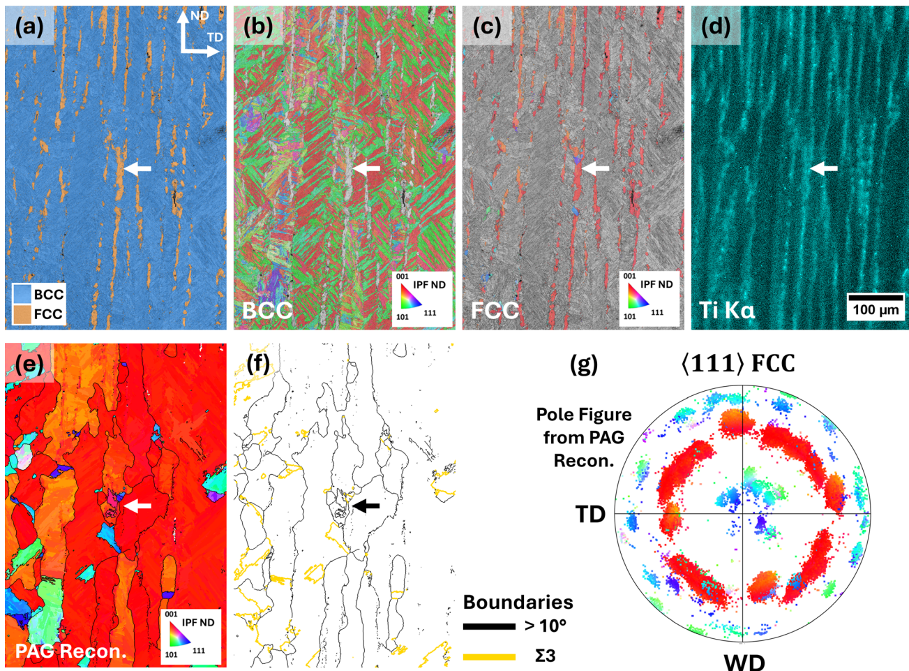
Fig. 14—A small-area EBSD map with simultaneous EDS of C465 in the as-built condition. (a) through (c) The phase colour map, the inverse pole figure (IPF) maps for the BCC phase and the IPF map for the FCC phase, respectively. All are overlaid with band contrast and the IPF orientations are aligned to the build normal direction. (d) The corresponding EDS map showing Ti Ka intensity. An arrow is positioned at the same location on each map. (e) A PAG reconstruction of the same EBSD map, also displayed in (a) through (c), here presented as an orientation map. (f) The same PAG reconstruction showing only grain boundaries, \Sigma 3 boundaries are highlighted in gold. (g) A pole figure from the same reconstruction showing all pixels, coloured as they were in (e) (Color figure online).
