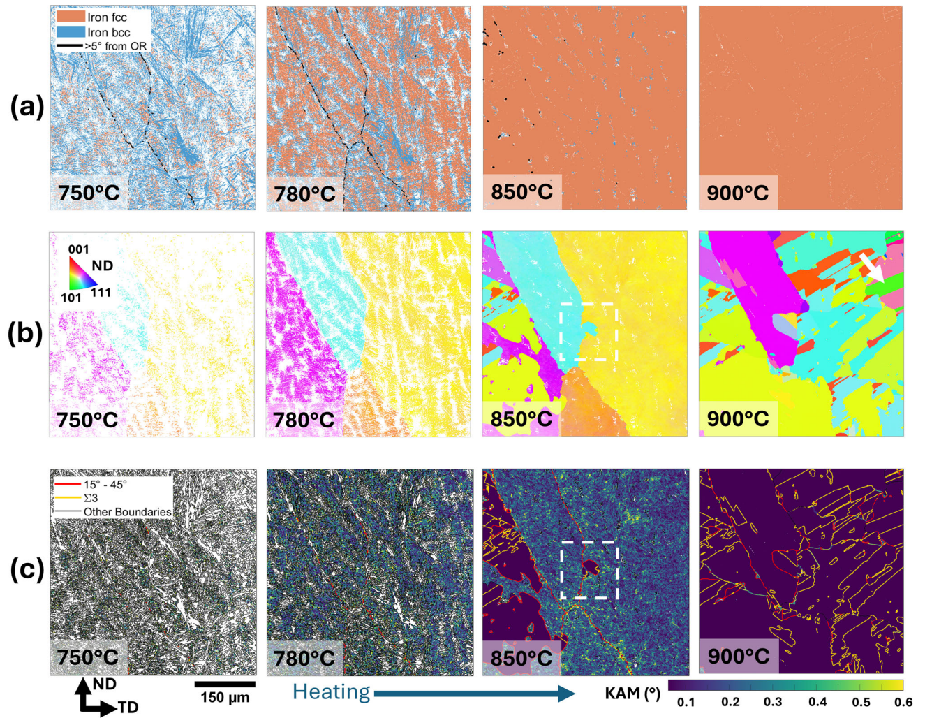
Fig. 10—Selected EBSD frames from the Test 1 (slow heating rate) in-situ EBSD experiment conducted with 300 M. The same four frames have been presented as: (a) phase maps with phase boundaries that do not obey an OR highlighted in black ( > 5 deg), (b) EBSD orientation maps (FCC phase only) and (c) KAM maps with high-angle grain boundaries, twin boundaries and other boundaries highlighted in red, gold, and black, respectively. Dashed boxes indicate regions magnified in Figure 12. Animated GIFs using all frames can be found in Ref. [47] (Color figure online).
