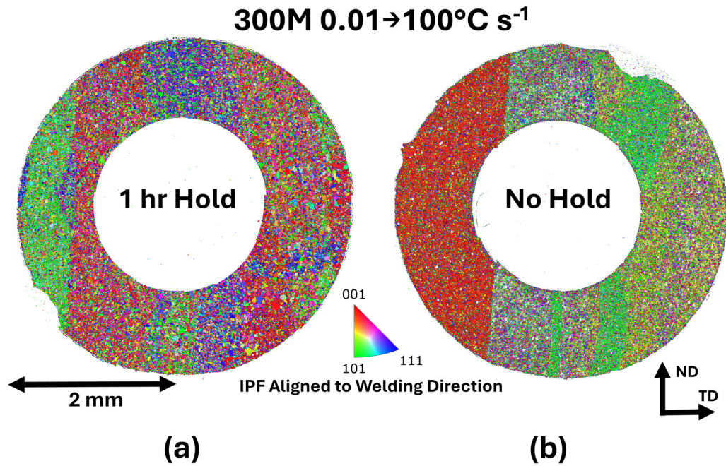
Fig. 5—The samples heated to 871 °C with the 0.01 → 100 °C s -1 heating profile, (a) was held for 1 h hold before quenching and (b) was immediately quenched after reaching 871 °C. The IPF key here was aligned to the welding (torch travel) direction as these colours better highlight the small grains present within larger columnar grains (Color figure online).
