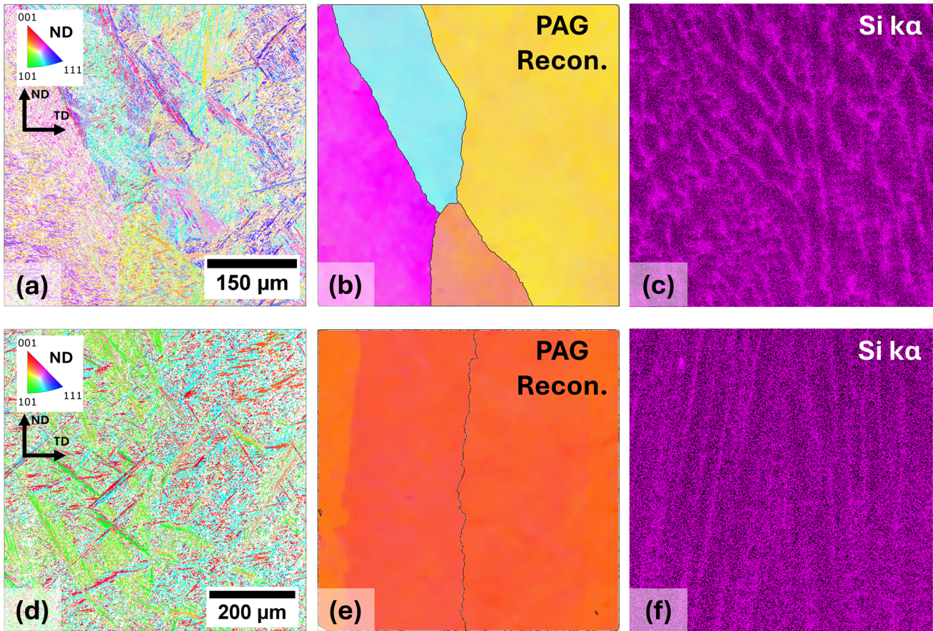
Fig. 8—(a) through (c) EBSD orientation map of the Test 1 300 M in-situ experiment region prior to heating, its PAG reconstruction with grain boundaries shown in black ( > 10^{\circ} deg), and a k\alpha intensity Si EDS map collected simultaneously. (d) through (f) Equivalent maps for Test 2 (Color figure online).
