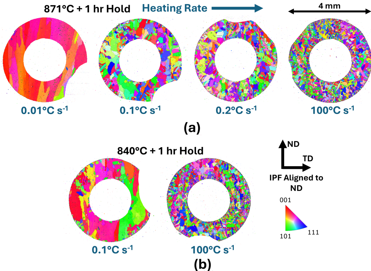
Fig. 4—EBSD PAG reconstructions from the 300 M dilatometry investigation. (a) The 871 °C and 1 h hold samples with varying heating rates. (b) The samples heated to the lower 840 °C austenitisation temperature and held for 1 h with slow and fast heating rates.
