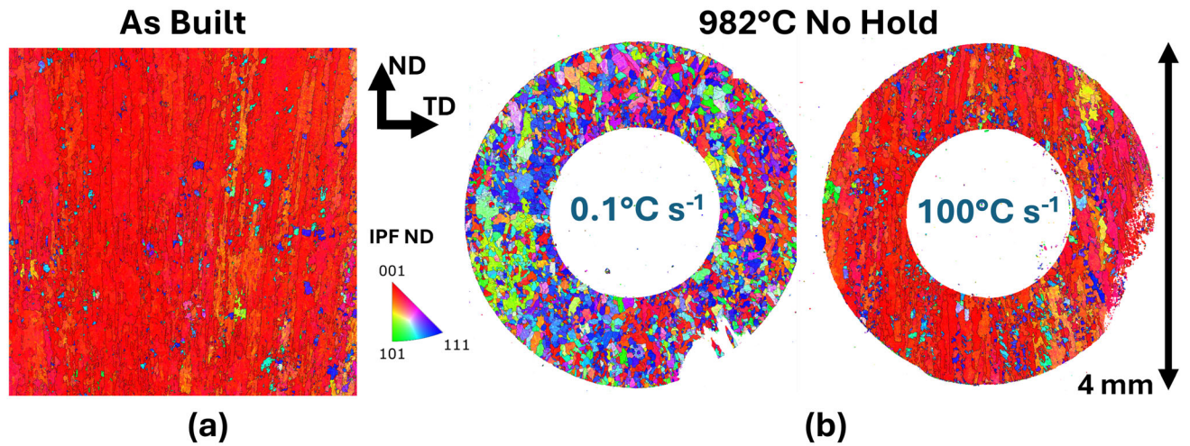
Fig. 15—(a) A large-area EBSD PAG reconstruction of the as-built C465 microstructure. (b) EBSD PAG reconstructions of the C465 dilatometry sample cross-sections heated to 982 °C and immediately quenched, at slow and fast heating rates, respectively.
