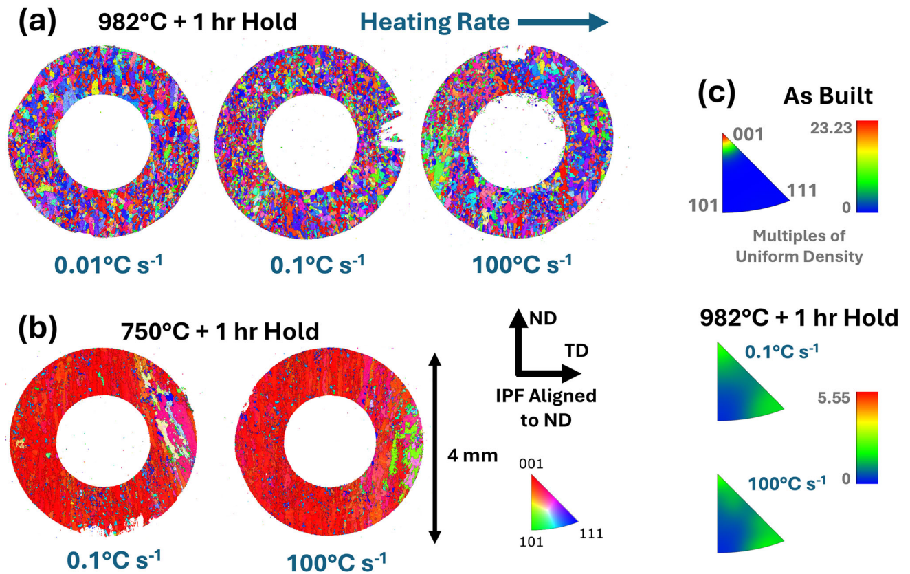
Fig. 16—EBSD PAG reconstructions from the C465 dilatometry investigation. (a) The 982 °C and 1 h hold samples with varying heating rates. (b) The samples heated to the lower 750 °C austenitisation temperature and held for 1 h with slow and fast heating rates. (c) IPF plots constructed from PAG reconstructions showing FCC texture evolution in the as-built material [Figure 15(a)] and in slow and fast heating rate 982 °C and 1 h hold dilatometry samples after recrystallisation.
