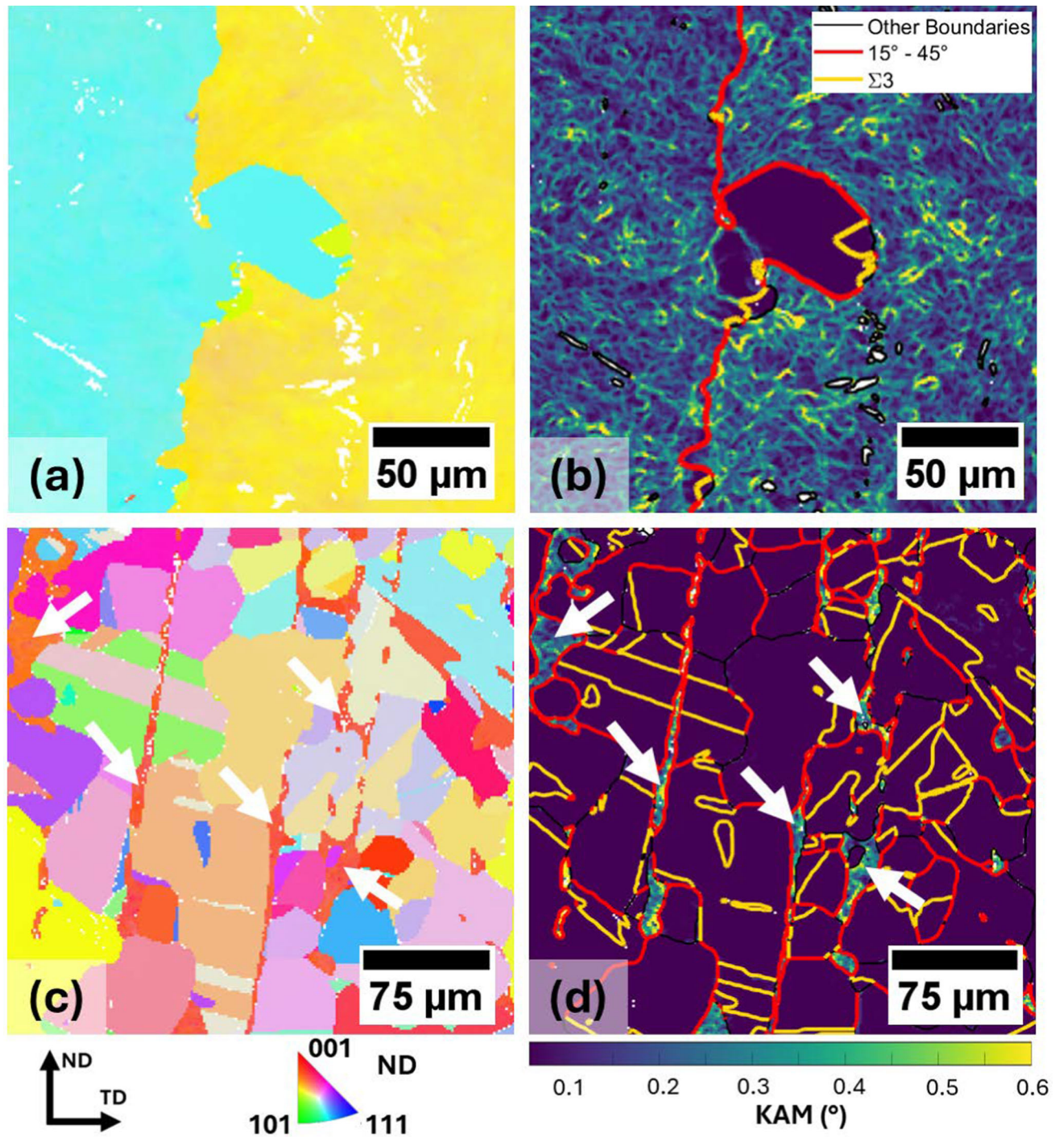
Fig. 12—(a) and (b) A magnified area from the Test 1 (300 M) 850 °C frame, also displayed in Figure 10. (c) and (d) A magnified area from the Test 2 (300 M) 900 °C frame, also displayed in Figure 11, memory orientation grains are highlighted by white arrows. Both areas are displayed as an FCC orientation map and a KAM map, respectively. In the KAM map high angle grain boundaries have been highlighted in red and twin boundaries in gold (Color figure online).
