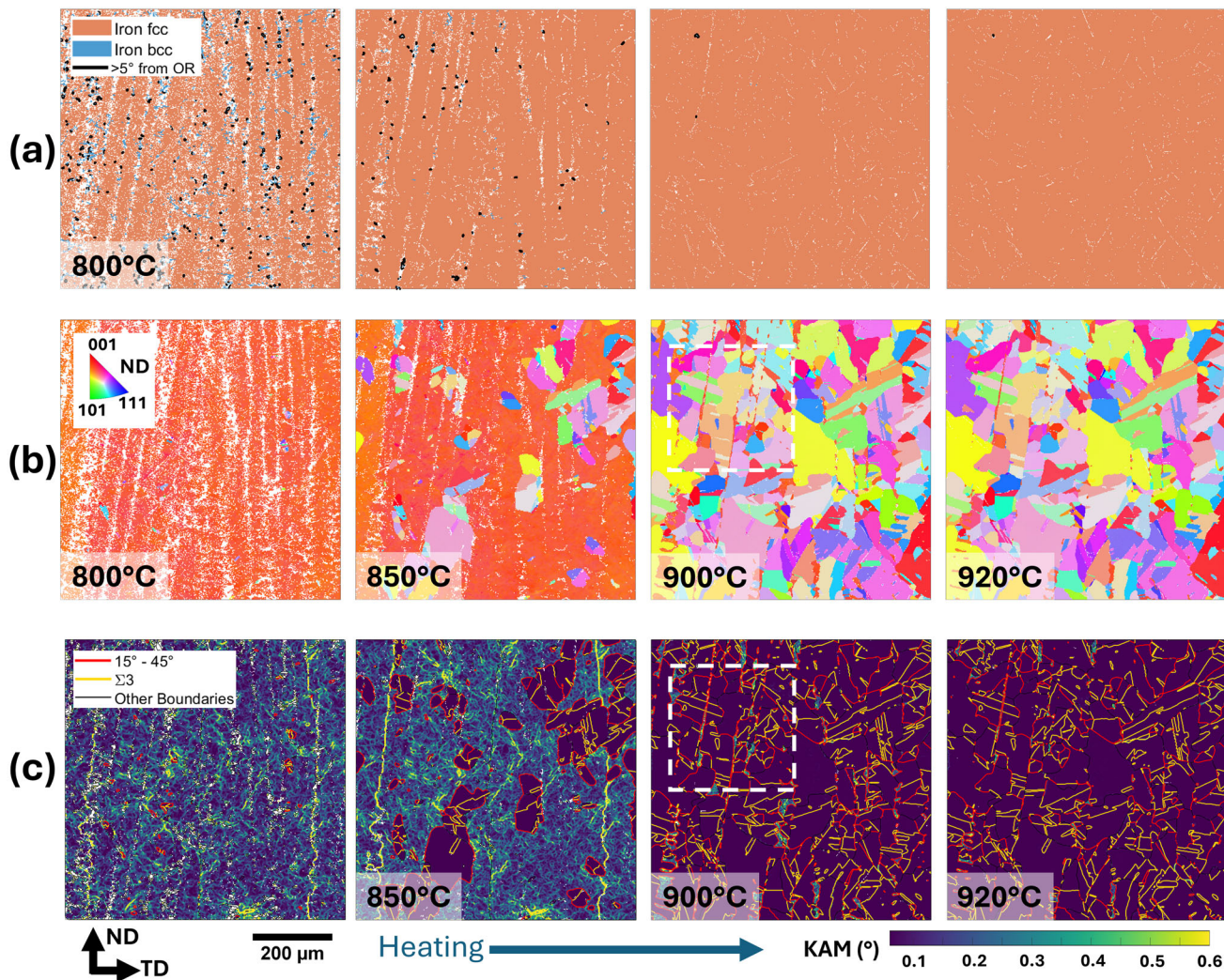
Fig. 11—Selected EBSD frames from the Test 2 (fast heating rate) in-situ EBSD experiment conducted with 300 M. The same four frames have been presented as: (a) phase maps with phase boundaries that do not obey an OR highlighted in black ( > 5^\circ ), (b) EBSD orientation maps (FCC phase only) and (c) KAM maps with high-angle grain boundaries, twin boundaries and other boundaries highlighted in red, gold, and black, respectively. Dashed boxes indicate regions magnified in Figure 12. Animated GIFs using all frames can be found in Ref. [47] (Color figure online).
