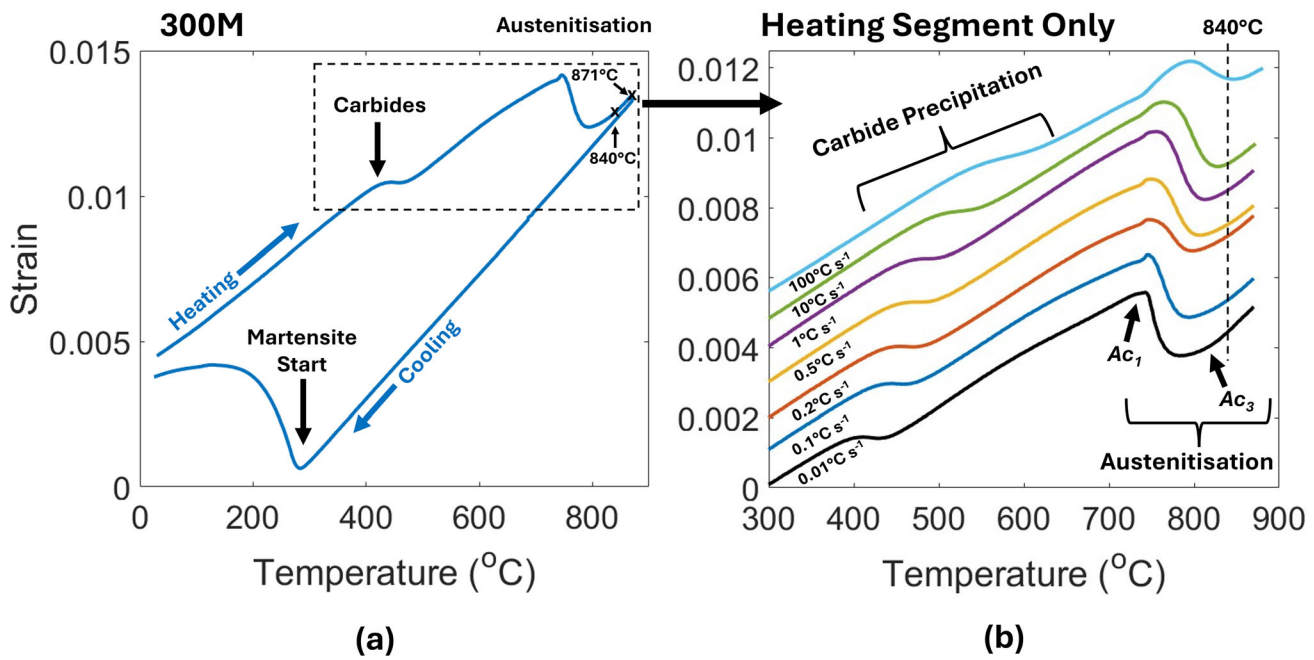
Fig. 7—(a) The full dilatometry curve from the 300 M 0.1^{\circ}\text{C s}^{-1} heating rate to 871^{\circ}\text{C} test, with a 1 h hold at temperature. (b) The heating data between 300^{\circ}\text{C} and 870^{\circ}\text{C} from the boxed section shown in (a). The same region from the other the 300 M dilatometry curves with different heating rates are also displayed, their strain has been offset to allow for direct comparison.
