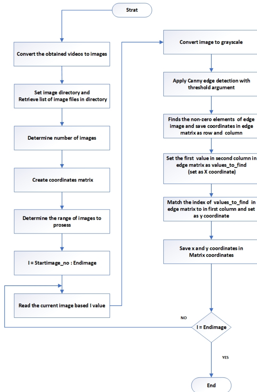
Figure 9. Beam tip detection flowchart.
