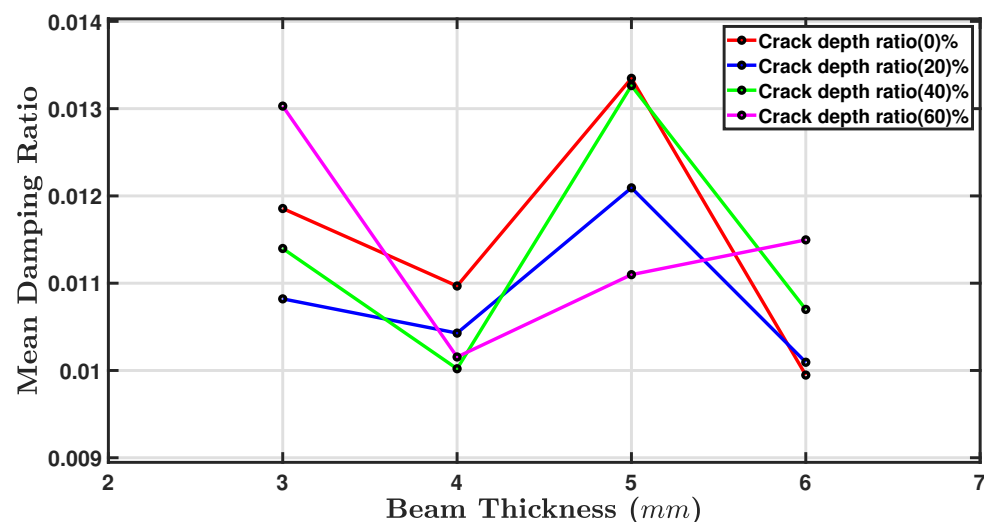
Figure 16. The relationship between mean damping ratio and beam thickness in different crack depth ratios.
