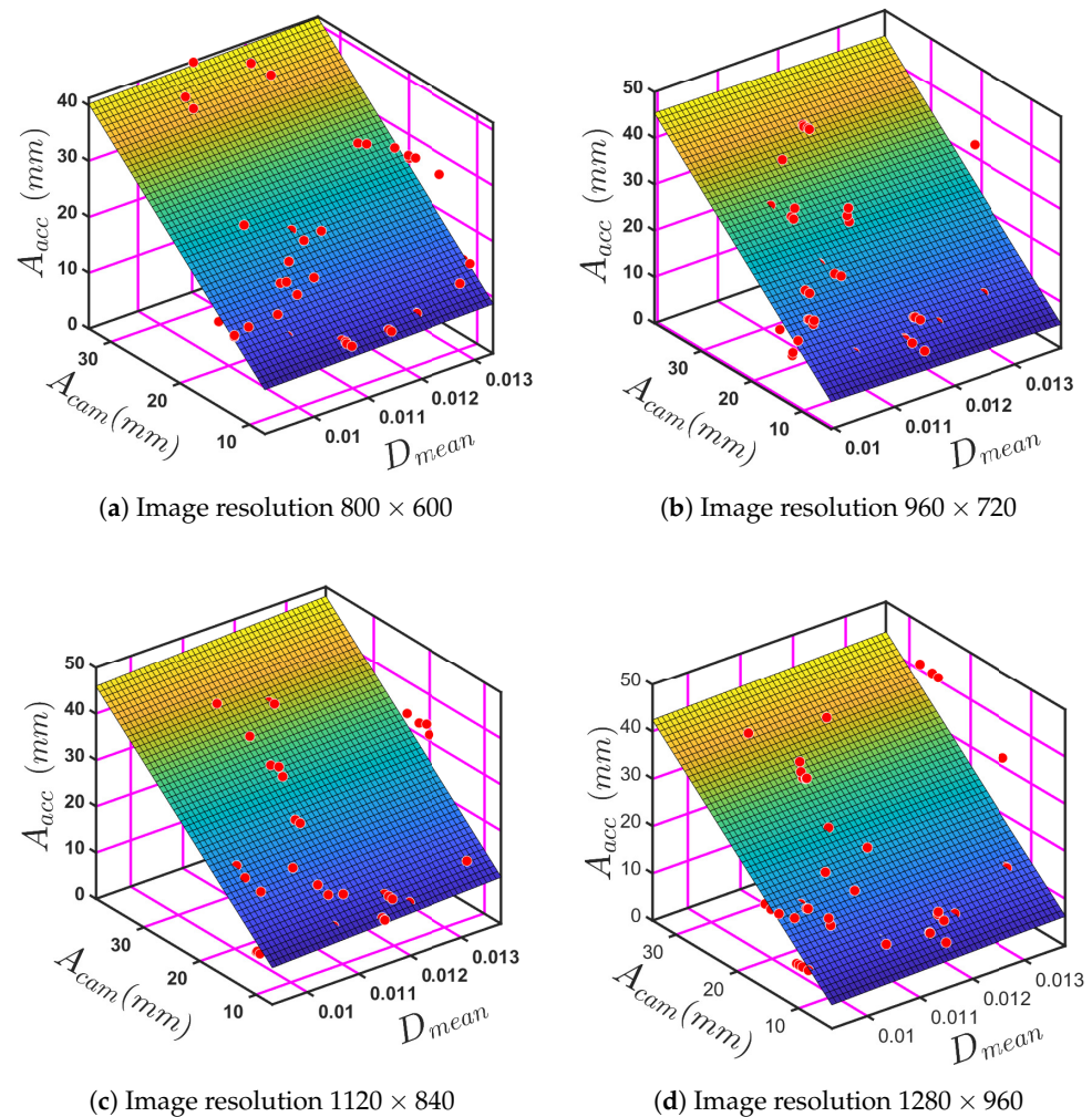
Figure 26. 3D linear model to predict resonance amplitude A_{acc} from A_{cam} and D_{mean} with four different image resolutions.
