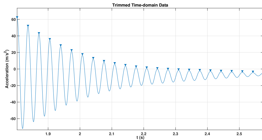
Figure 6. The gradual reduction in the amplitude of free vibrations.
