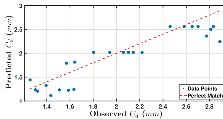
Figure 33. The observed C_d and predicted C_d measurements.
