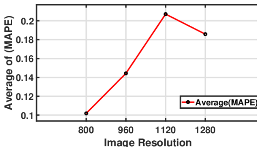
Figure 22. Average MAPE for natural frequency as a function of image resolution.
