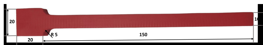
Figure 1. One specimen was printed using a nozzle size of 0.4 mm, 0° raster angle printing orientation, and 0.5 mm layer thickness (Unit: mm).
