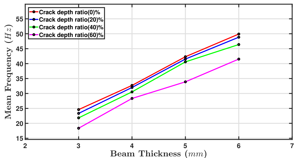
Figure 14. The relationship between mean frequency and beam thickness.
