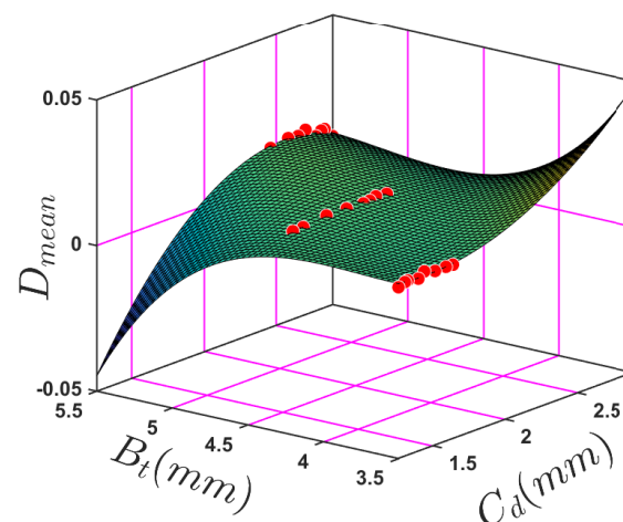
Figure 29. Nonlinear least squares are used to optimise empirical correlation between crack depth, beam thickness and mean damping ratio.
