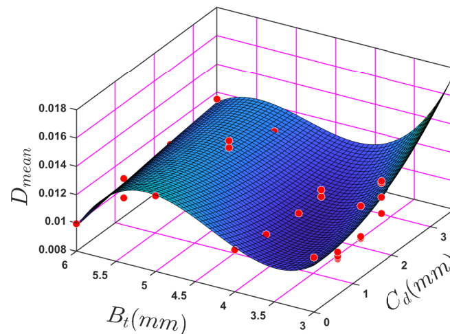
Figure 28. Experimental and surface fitted data for nonlinear empirical correlation between crack depth, beam thickness and mean damping ratio.
