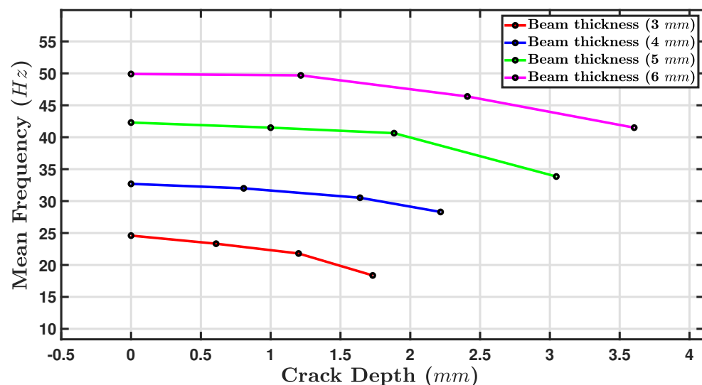
Figure 15. The relationship between mean frequency and crack depth.
