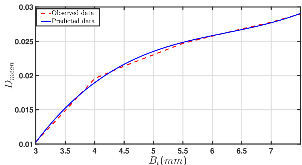
Figure 23. The relationship between beam thickness and damping ratio: measured and predicted.
