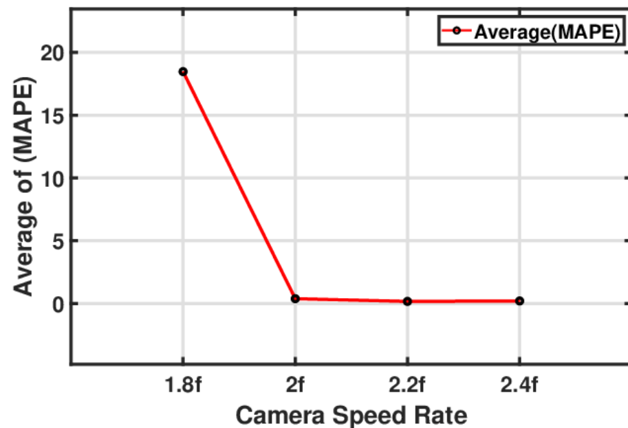
Figure 19. Average mean absolute percentage error for fundamental natural frequency as a function of camera speed.
