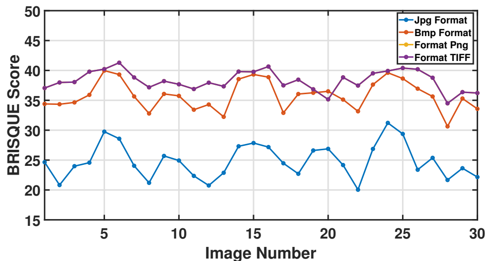
Figure 8. BRISQUE scores for 30 images with different image formats.
