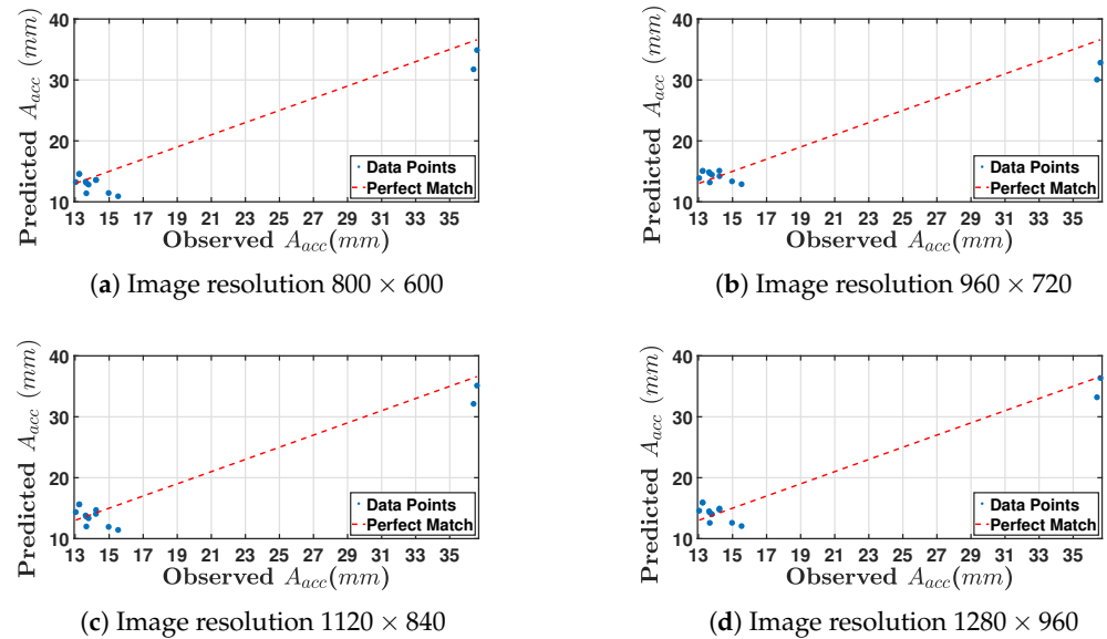
Figure 32. Four different image resolutions of observed ( A_{acc} ) and predicted ( A_{acc} ) values.
