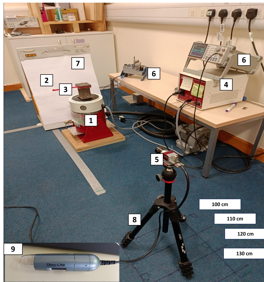
Figure 3. Experimental setup and procedures. 1 Shaker 2 Accelerometer 3 Specimen 4 Power Amplifier 5 Camera 6 Function Generator 7 White Background 8 Tripod 9 Microscopy Camera.
