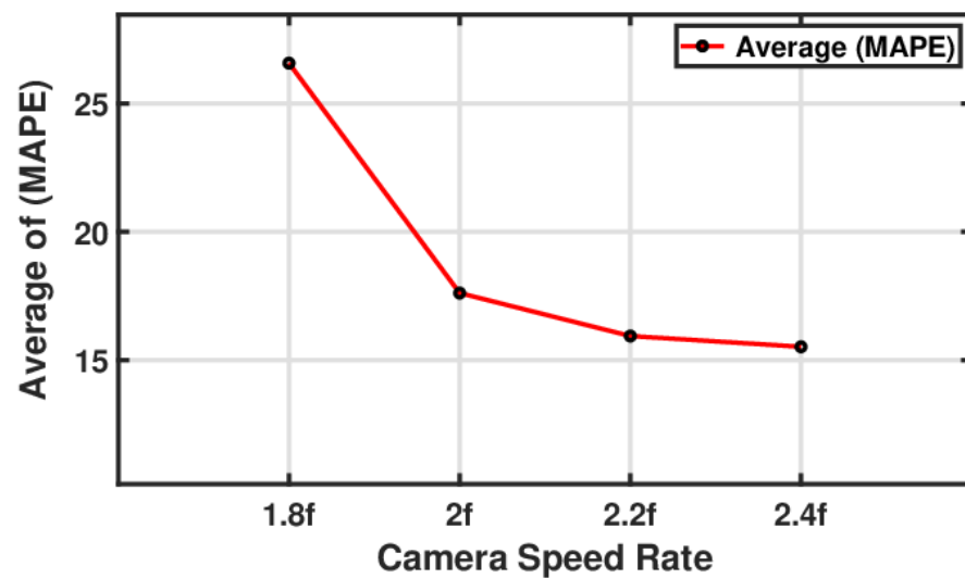
Figure 20. Average mean absolute percentage error for resonance amplitude as a function of camera speed.
