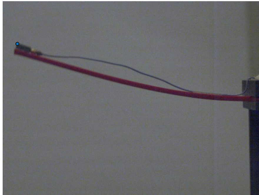
Figure 10. Beam tip detection in coloured image.
