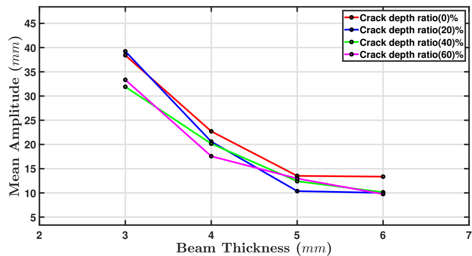
Figure 17. Mean amplitude as a function of beam thickness for four crack depth ratios.
