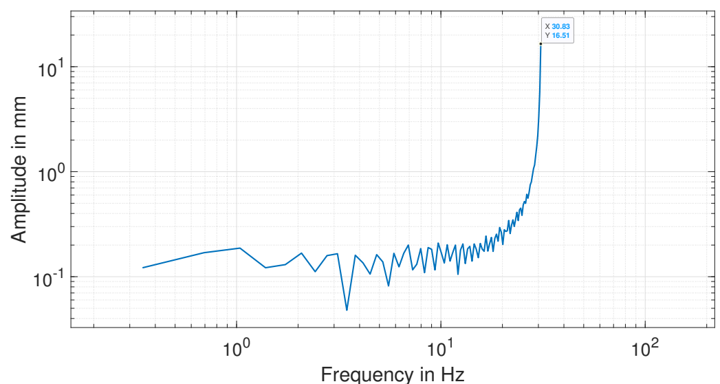
Figure 13. Camera frequency domain using FFT.
