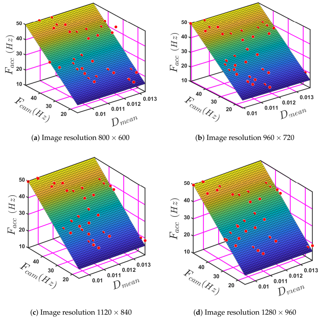
Figure 24. The 3D linear model to predict frequency F_{acc} from F_{cam} and D_{mean} for four image resolutions.
