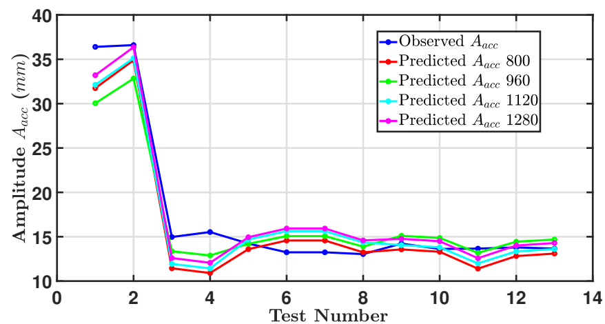
Figure 27. Comparison of validation and model prediction results for the A_{acc} .
