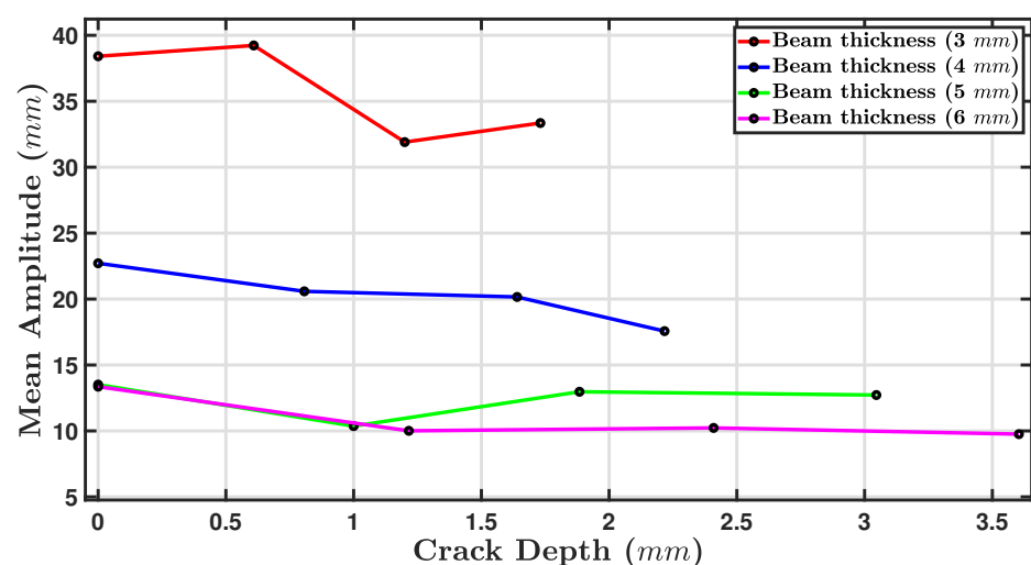
Figure 18. The relationship between mean amplitude and beam thickness.
