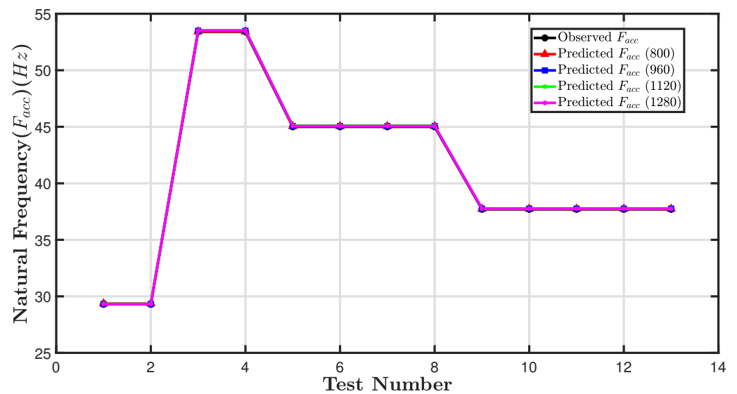
Figure 25. Comparison of validation and model prediction results for the F_{acc} .
