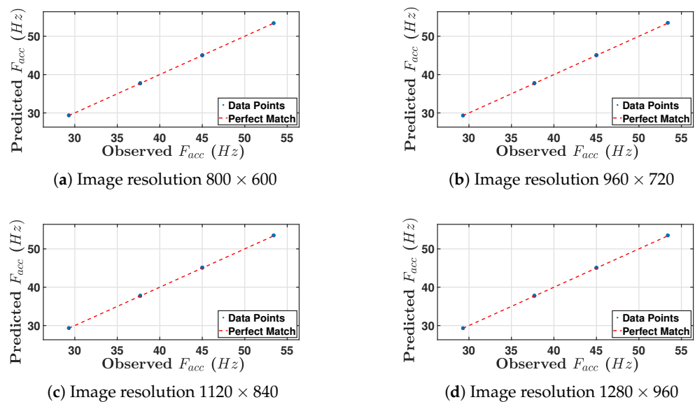
Figure 31. Observed and predicted ( F_{acc} ) values for four different image resolutions.
