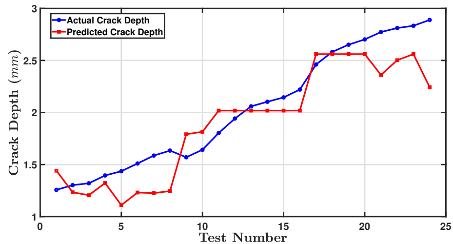
Figure 30. Comparison of model actual crack depth with predicted crack depth optimised with nonlinear least squares ( NLS ).
