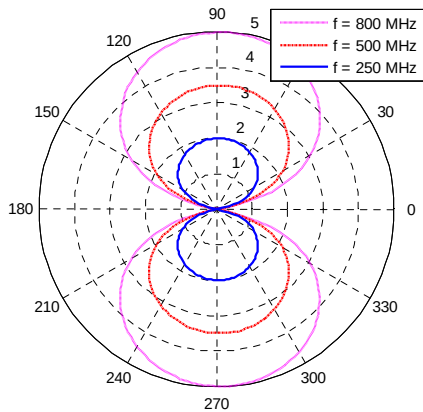
Fig. 9 Radiation patterns simulated for the antenna in the E_0 component of the E-plane (1 dBi/div).
