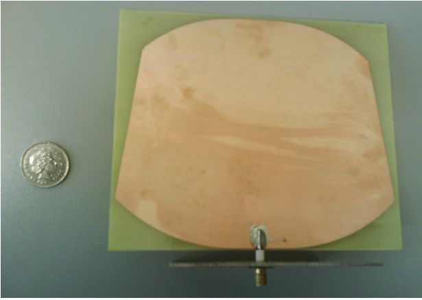
Fig. 2 Picture of the wideband blade monopole antenna (dimensions: height =145 mm , width =166 mm, bevel angle 15° ).
