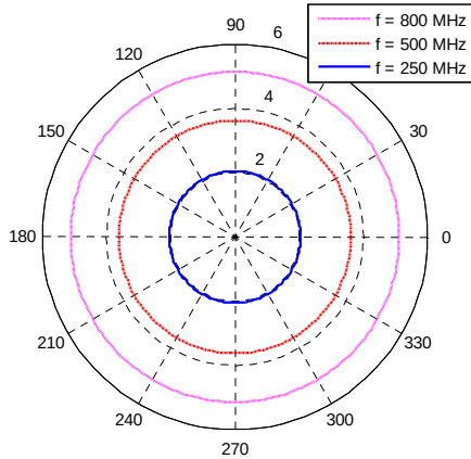
Fig. 8 Radiation patterns simulated for the antenna in the E_0 component of the H-plane (2 dBi/div).
