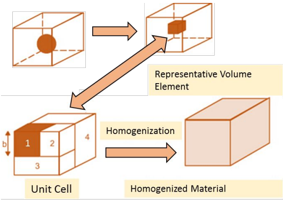
Figure 4 Representative unit-cell model for the particulate composite with cubic particle embedded in a matrix.
