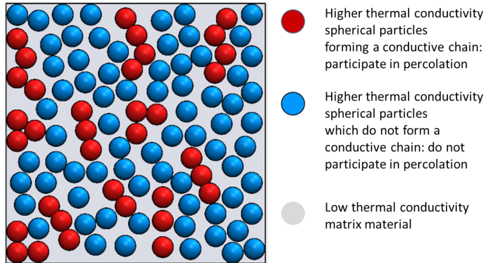
Figure 1: Percolation model showing particles forming a conductive chain and participating in percolation paths, and randomly distributed particles in low thermal conductivity matrix.
