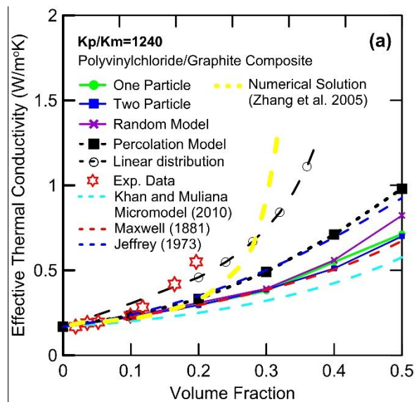
Figure 13. Comparison of the experimental data and predicted ETC for a) Polyvinylchloride/Graphite b) Polyethylene/Graphite composites.
