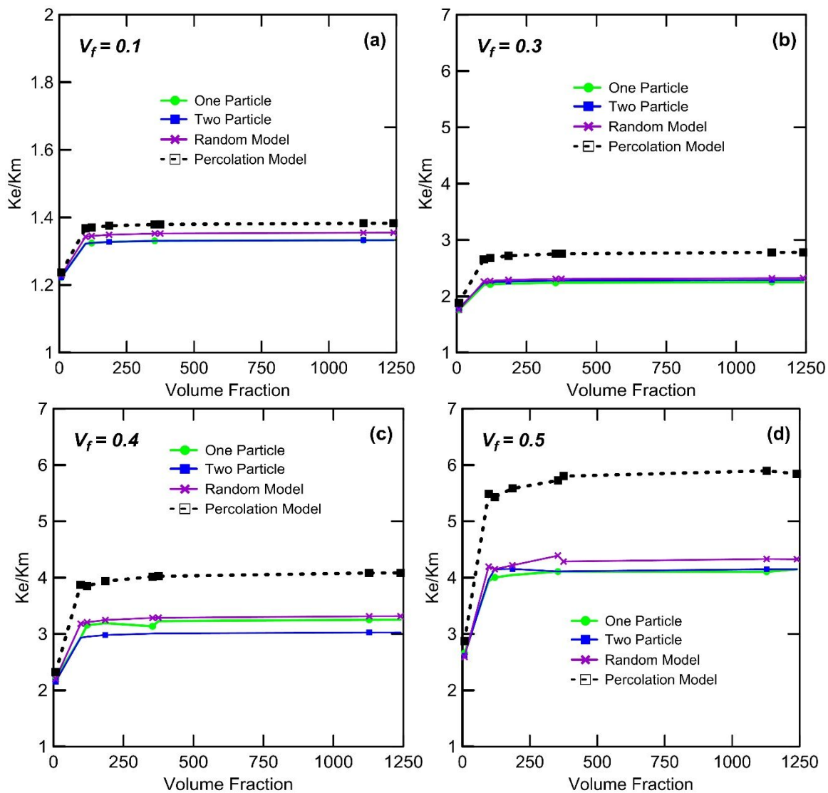
Figure 6. Conductivity mismatch in a two-phase composite material and its effect on the ETC for various micromechanical models..
