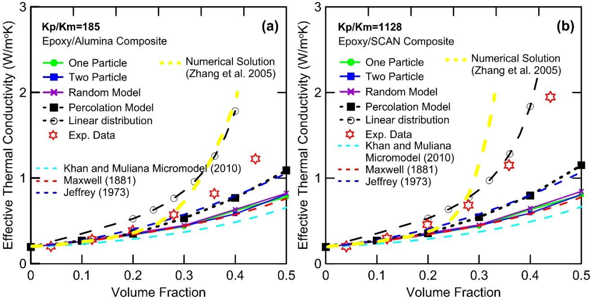
Figure 10. Comparison of the experimental data and predicted ETC for a) Epoxy/Alumina b) Epoxy/silica coated aluminum nitride composites.
