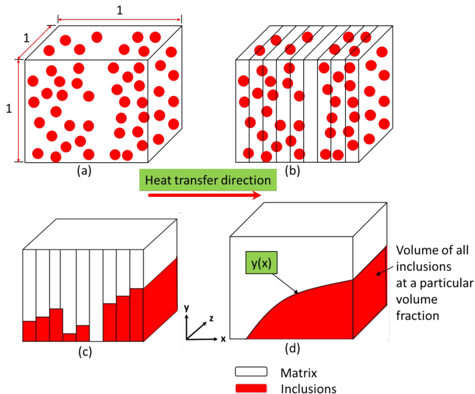
Figure 5. A cubic unit cell for the study of the ETC of a two-phase composite material (after [28]). (a) Inclusions randomly distributed in the matrix, (b) hypothetically sliced thin layers, (c) histogram of the layers and (d) corresponding equivalent continuous distribution of the histogram.
