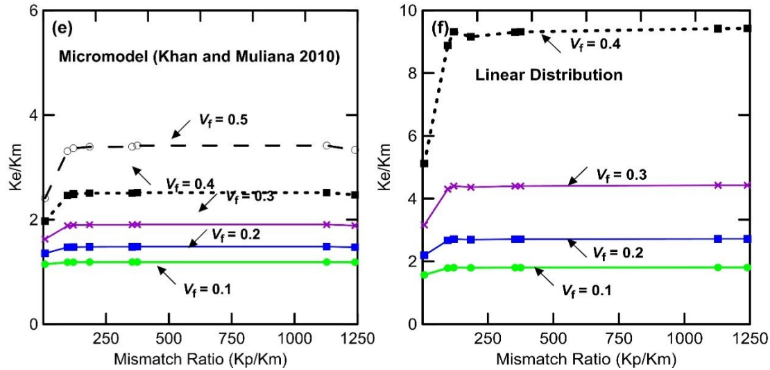
Figure 7. Conductivity mismatch in a two-phase composite material and its effect on the ETC for various micromechanical models.
