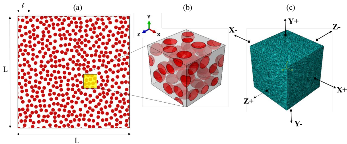
Figure 3 (a) Random distribution of particle (b) RVE (c) Meshed RVE with 10-noded quadratic heat transfer tetrahedron elements (DC3D10) showing 6 boundary faces with respect to the axes directions.
