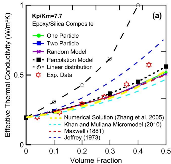
Figure 9. Conductivity mismatch in a two-phase composite material and its effect on the ETC for various micromechanical models.
