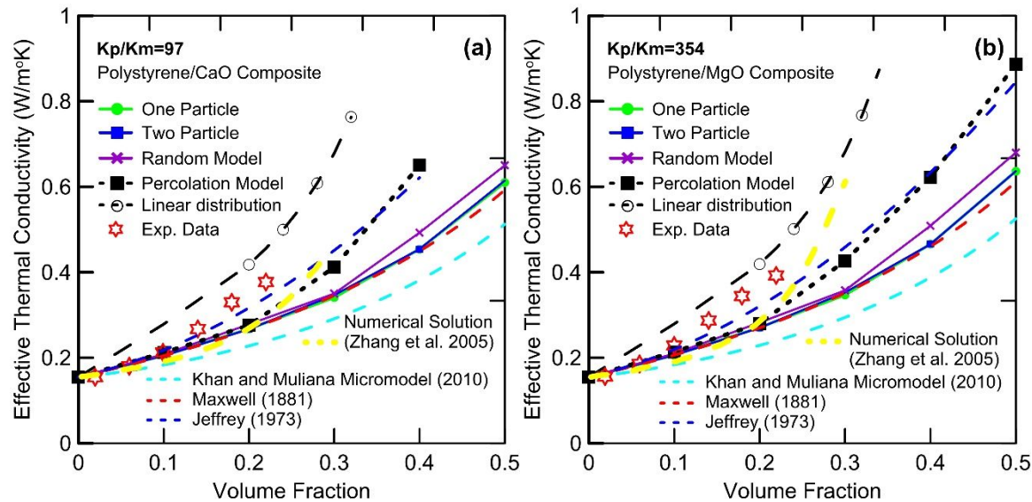
Figure 11. Comparison of the experimental data and predicted ETC for a) Polystyrene/CaO b) Polystyrene/MgO composites.
