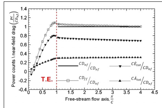
Figure 10. Comparison of near-field and exergy-based drag of the unpowered 3D wing configuration decomposed into total anergy rate and total exergy outflows components.
