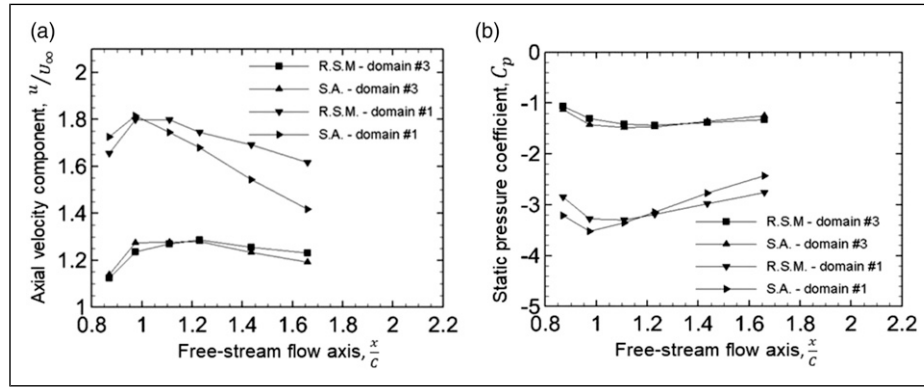
Figure 8. Dependency of vortex core flow quantities, of (a) axial velocity component u/U_\infty and (b) static pressure coefficient C_p , on turbulent models of Spalart–Allmaras (S.A.) and Reynolds Stress Model (R.S.M.) as calculated on domains #1 and #3.
