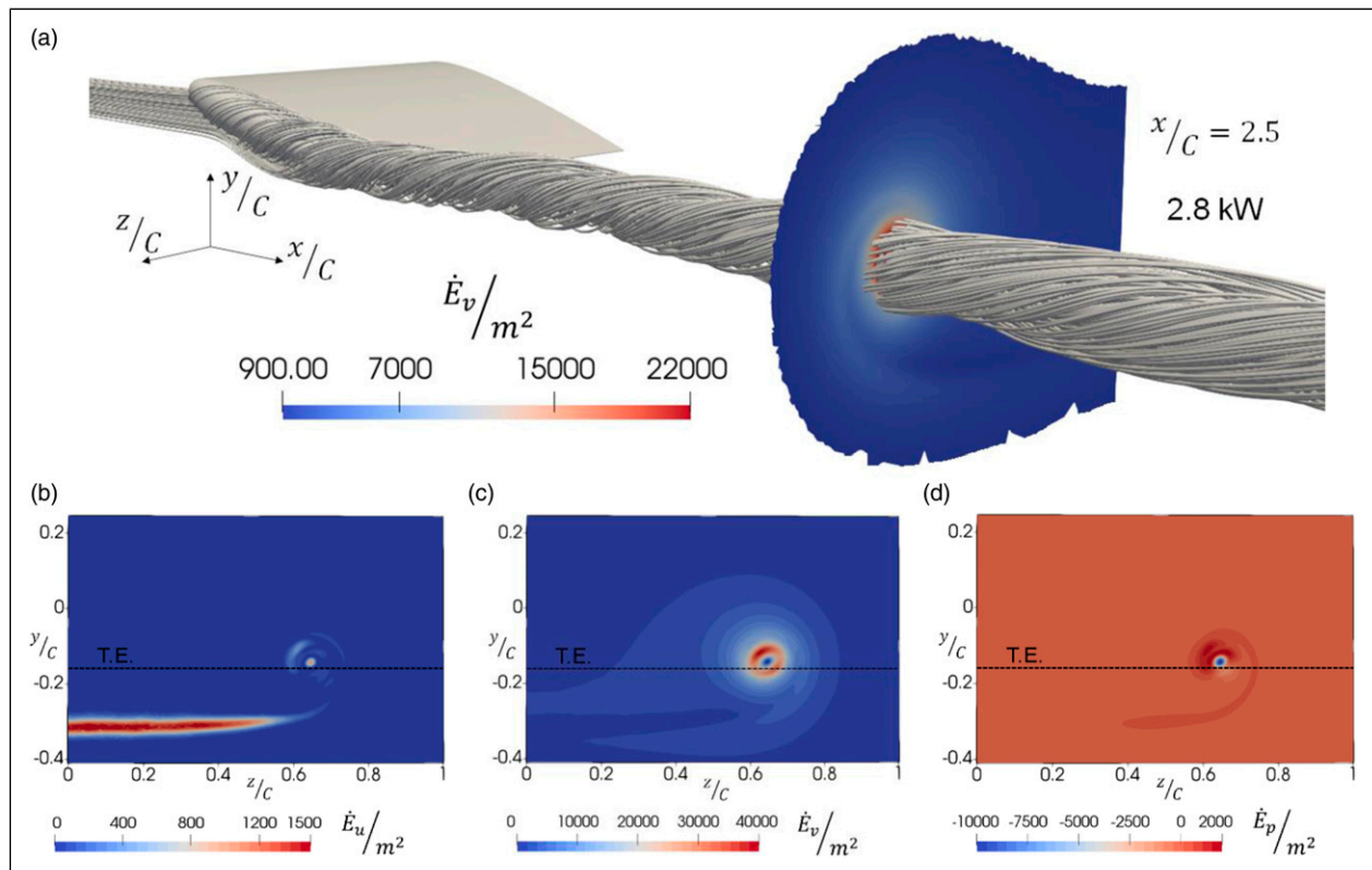
Figure 14. Flow stream tracers, representing the recuperation potential of the vortex (a). Contours of (b) \dot{E}_u (c) \dot{E}_v and (d) \dot{E}_p , exergetic sources at x/c = 2.5 downstream of the wing’s trailing-edge.
