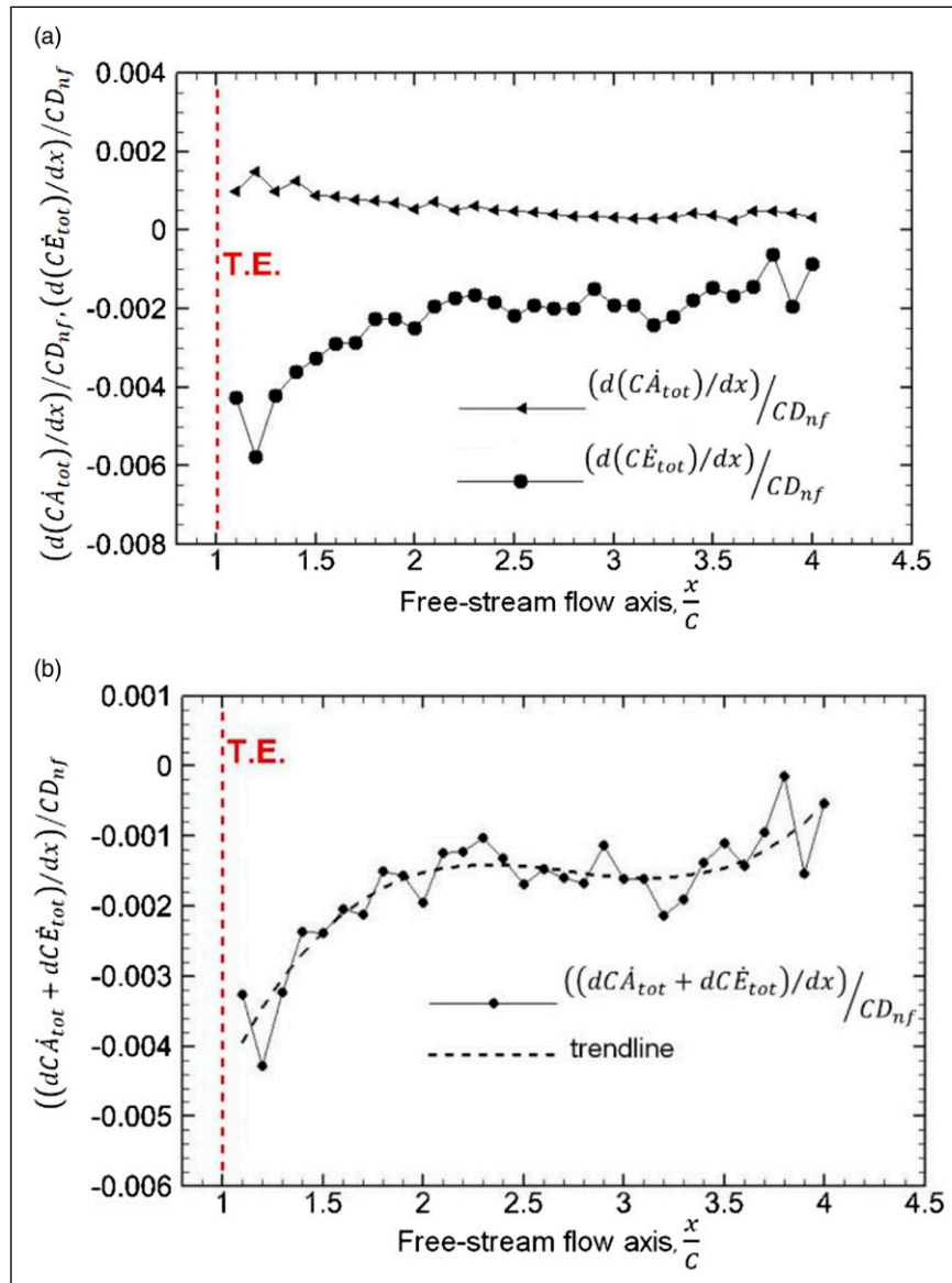
Figure 11. Evolution of exergy destruction and anergy production rates (a) and study of (in)consistency between the theoretical exergy balance formulation and CFD implementation (b).
