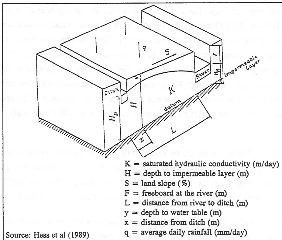
Figure 2.5: Steady State Water Table Model
