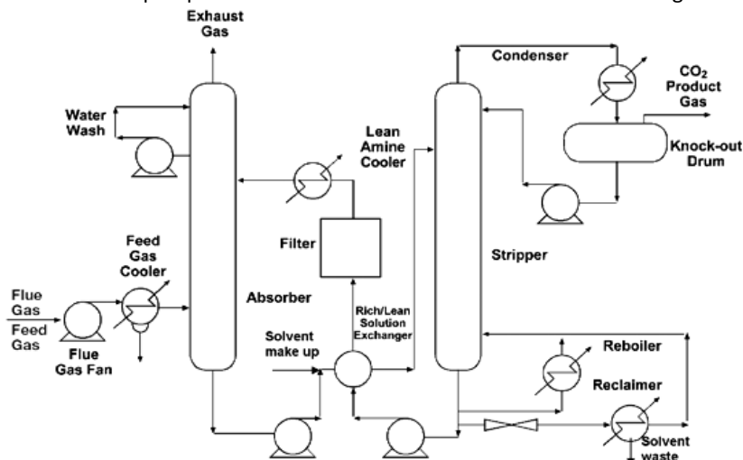
Figure 2 Process flow diagram for \text{CO}_2 capture from flue gas by chemical absorption (IPCC, 2005)
