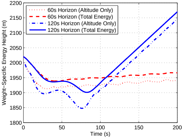
Fig. 4. Comparison of energies between two simulations with differing control horizons — 60 s (red) and 120 s (blue).
