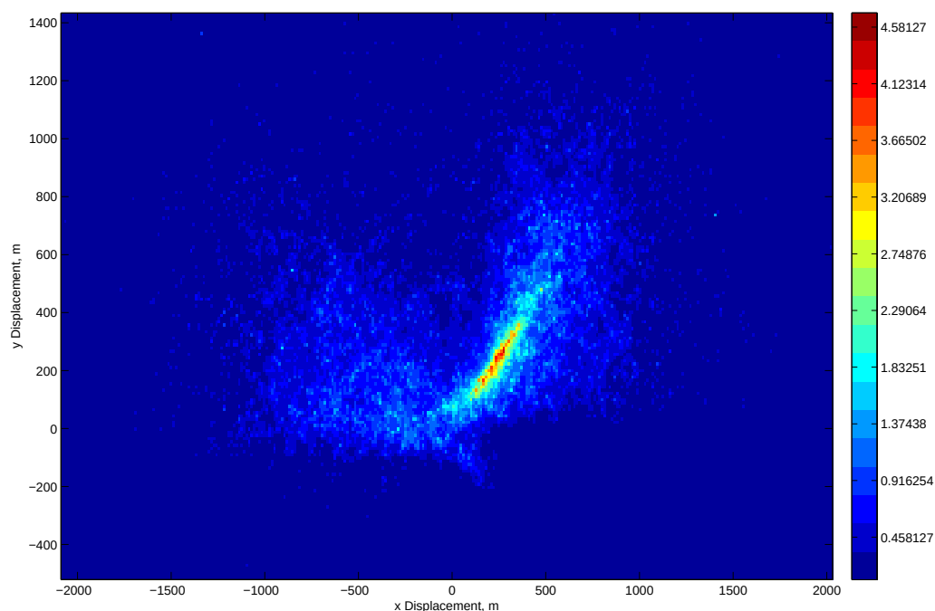
Figure 8. Monte Carlo simulation of the Algeria test case contoured by cell frequency, 10 000 iterations, 1 h simulation.
