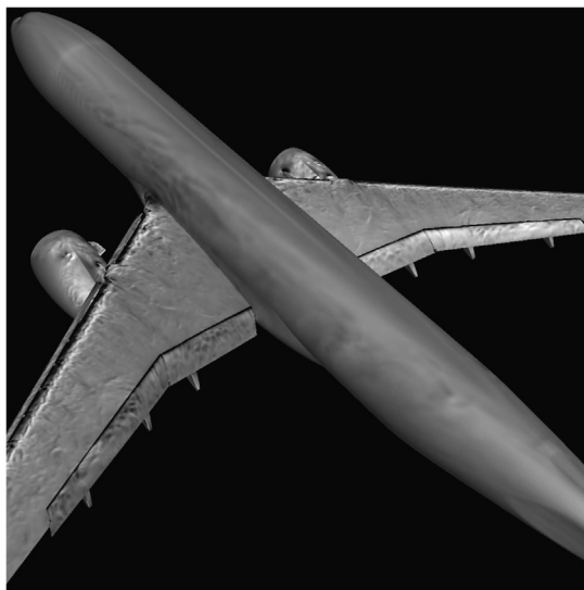
Fig. 22. Contour plot of skin friction coefficient on the surface of the NASA CRM High-Lift model used for the iLES simulation at Reynolds 5.49 Million, and AoA=21.47^\circ .
