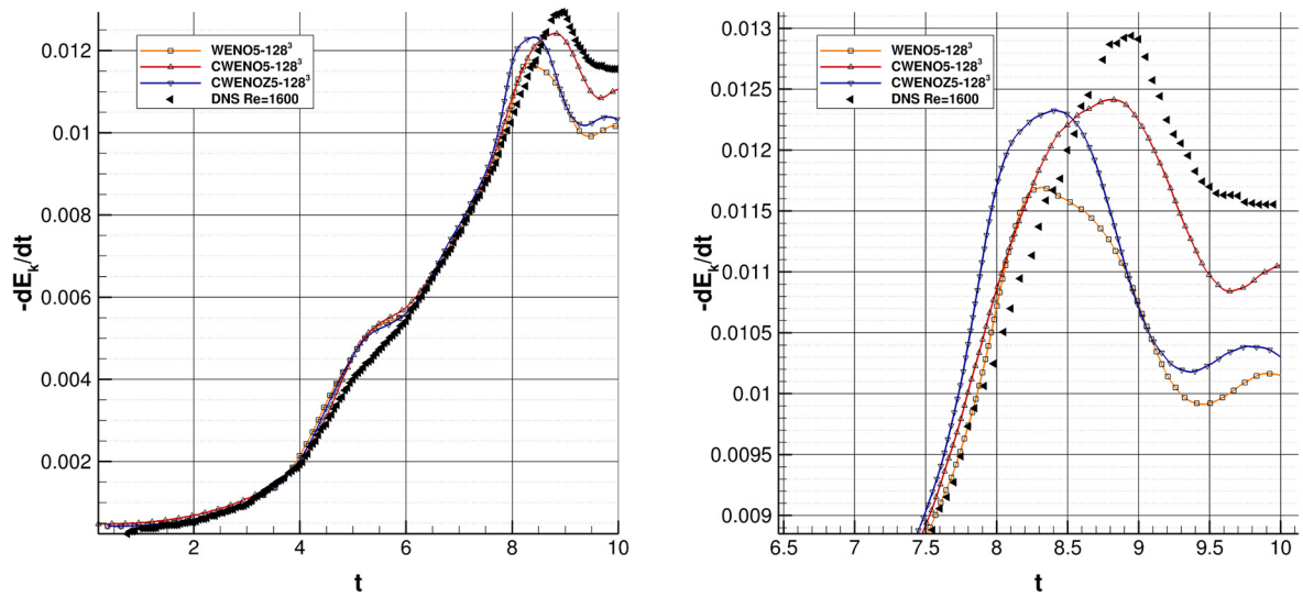
Fig. 8. Kinetic energy dissipation rate for the iLES of the Taylor-Green Vortex Re = 1600 obtained with various schemes on 128^3 hexahedral mesh, and comparison with the DNS results of Brachet et al. [122]. It can be noticed that all the schemes perform similarly, with CWENO and CWENOZ schemes being marginally less dissipative compared to WENO.
