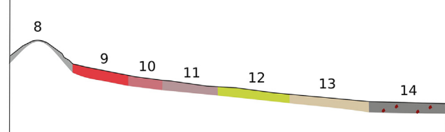
Fig. 4. Schematic transects of Tanganyikan catenas (Based on Milne, 1947 ): (a) Ukiriguru catena: 1 Granite tors with shallow grey coarse loam; 2 Brownish red loam over granite; 3 Brownish red loam with soft iron concretions; 4 Grey sand with iron concretions; 5 Non-calcareous hard pan soil; 6 Calcareous black sandy clay; 7 Heavy black clay. (b) Unyanyembe catena: 8 stony grey loam & bare rock; 9 Bright red earth; 10 Dull red earth; 11 Slightly reddish grey sand; 12 Yellowish grey sand; 13 Drab sand; 14 Mottled grey sandy clay.
