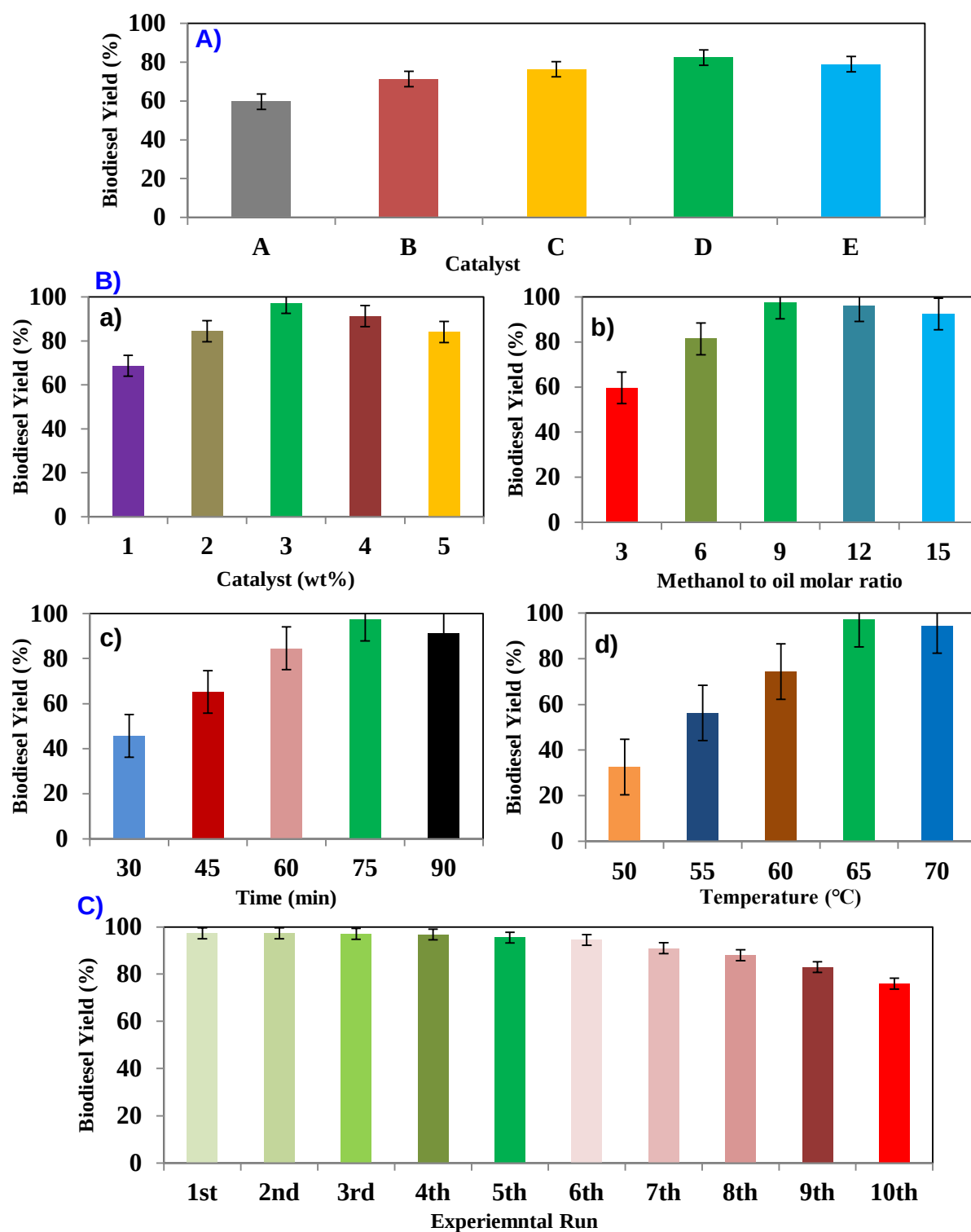
Figure 4: A) Biodiesel yield (%) for catalysts with varying concentrations of Sr and La. B) parametric study for: (a) catalyst loading, (b) methanol to PAS oil molar ratio, (c) reaction time and (d) reaction temperature. C) Evaluation of Sr: La-C catalyst reusability to produce biodiesel from PAS oil by transesterification.
