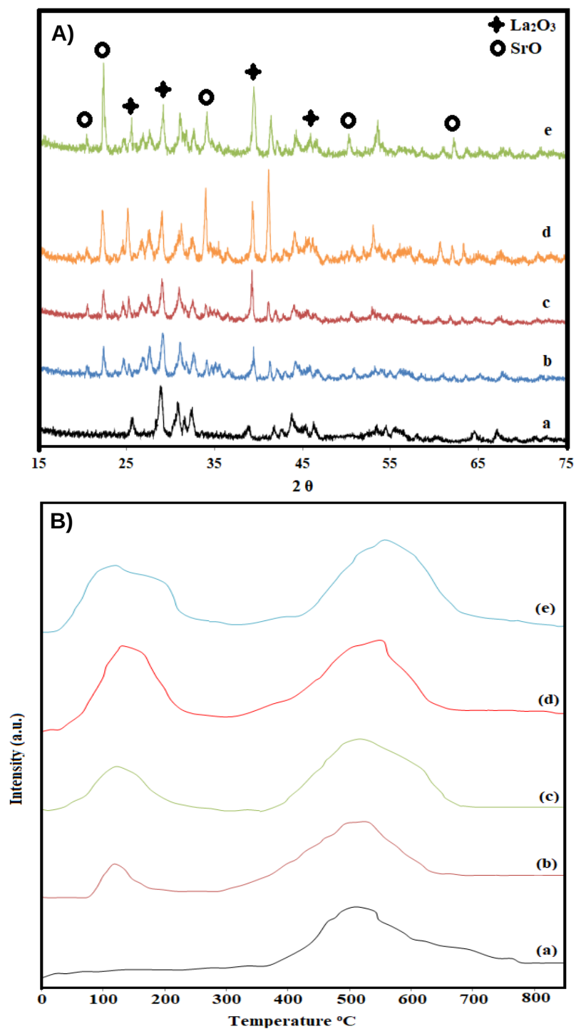
Figure 1: A) XRD diffractograms B) \text{CO}_2 -TPD results for synthesised catalysts: (a) parent \text{La}_2\text{O}_3 , (b) modified form of \text{La}_2\text{O}_3 with \text{SrO} with atomic ratio 4, (c) modified form of \text{La}_2\text{O}_3 with \text{SrO} with atomic ratio 6, (d) modified form of \text{La}_2\text{O}_3 with \text{SrO} with atomic ratio 8 and (e) modified form of \text{La}_2\text{O}_3 with \text{SrO} with atomic ratio 10.
