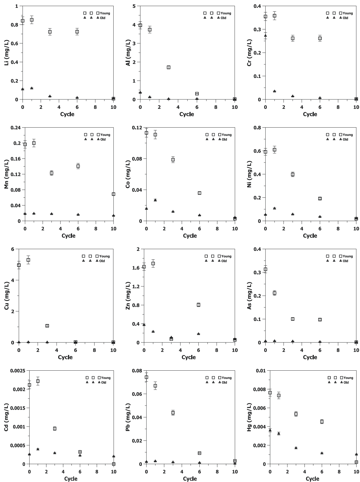
Fig. 4. Variations of metal(loid)s in the leachate from young (S.S) and old (S.G) landfill leachate.
