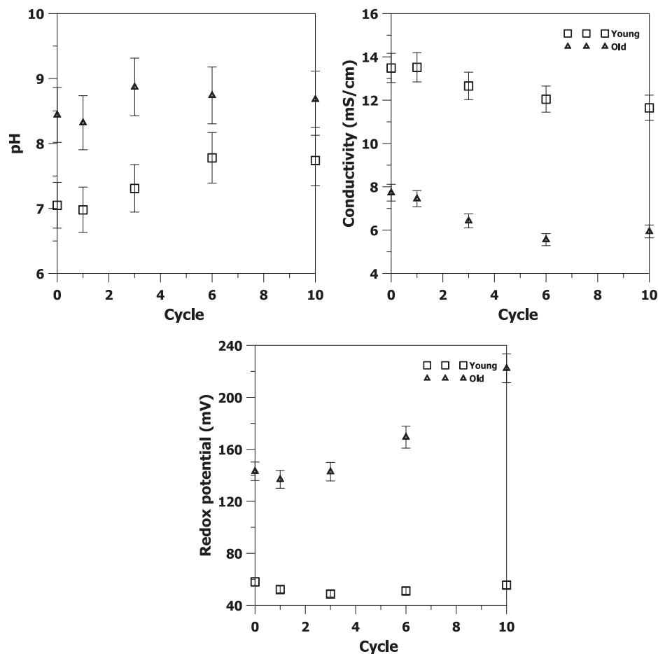
Fig. 2. Variations of pH, conductivity and ORP in the leachate from young (S.S) and old (S.G) landfill leachate.
