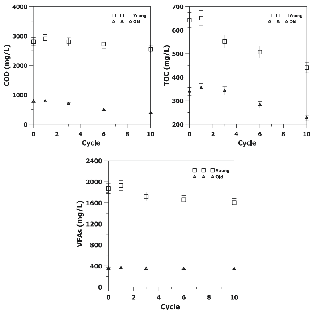
Fig. 3. Variations of COD, TOC and VFAs in the leachate from young (S.G) and old (S.G) landfill leachate.
