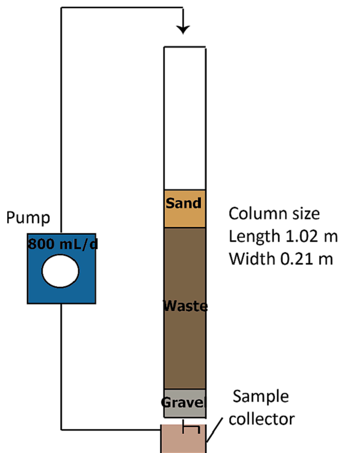
Fig. 1. Schematic diagram of the column percolation test.
