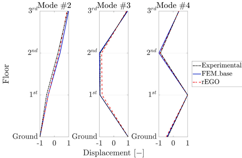
Fig. 9. Three-storey frame structure: Comparison of the \phi_{2-4} identified from Experimental data and computed from FEM_base and rEGO.
