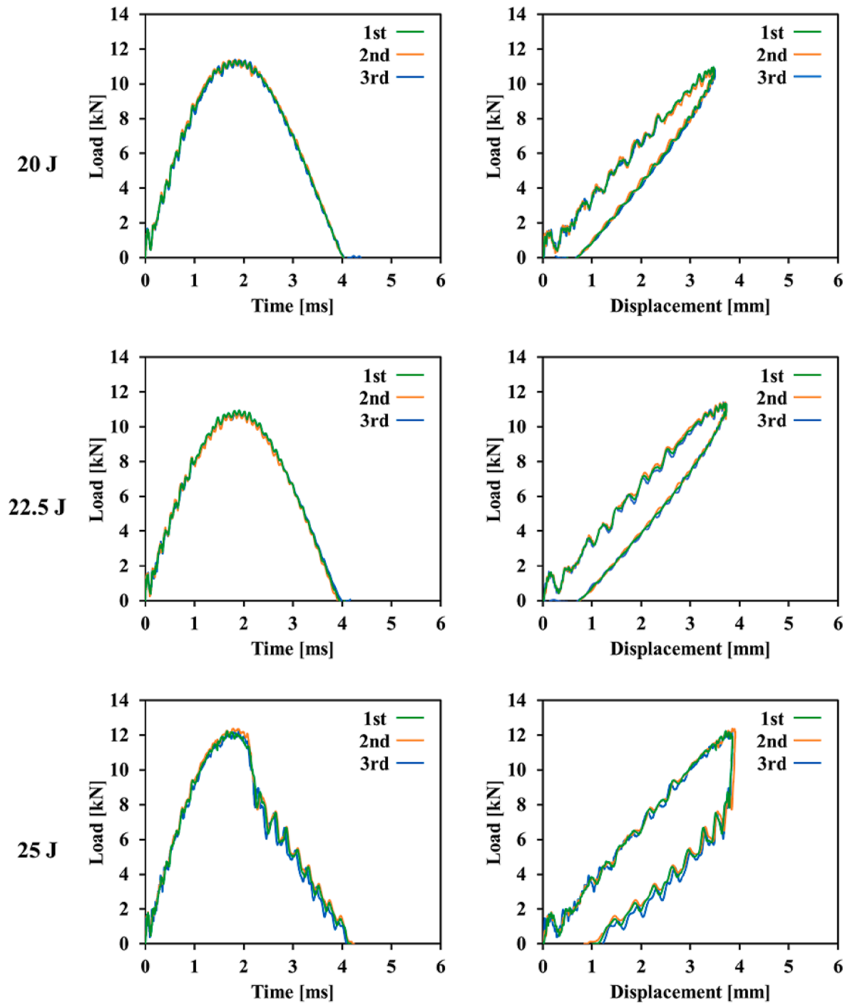
Fig. 12. Comparison between the load-time and load-displacement traces obtained for three replicate experiments for the flat-ended impactor at impact energies of 20, 22.5 and 25 J.
