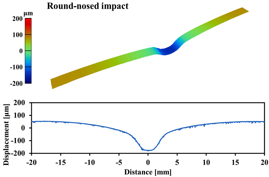
Fig. 13. A white light interferometer (WLI) scan of the indentation profile on the CFRP panel specimen subjected to the round-nosed impactor at an impact energy of 25 J.
