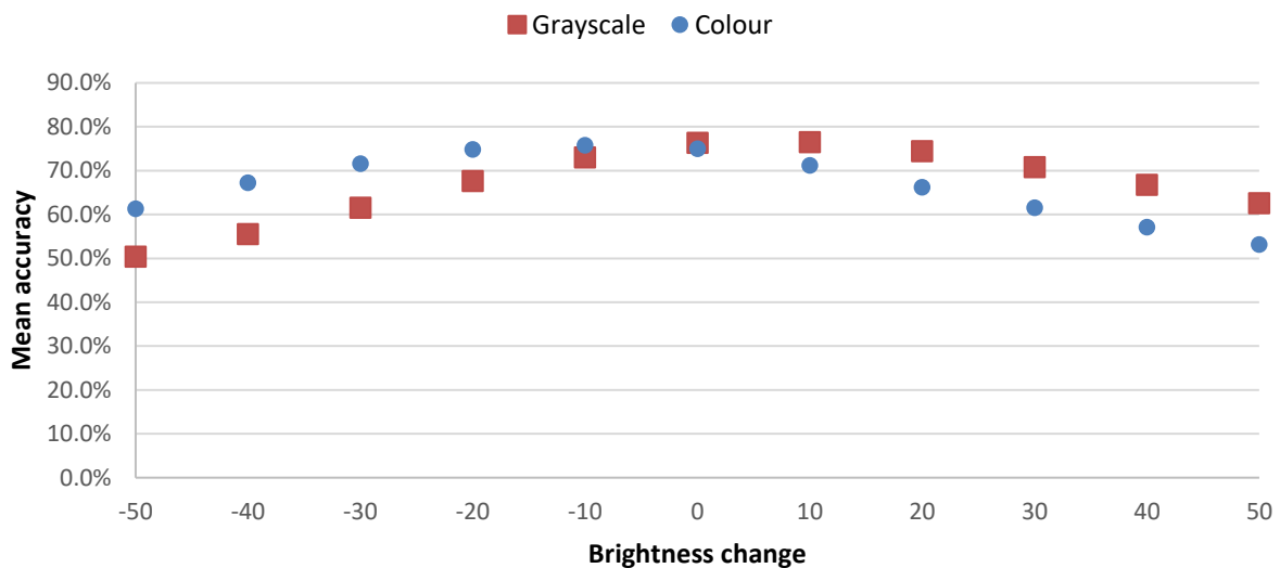
Figure 4-4. Comparison of the effects of changing the brightness channel when testing coloured or converted-to-greyscale images. Standard deviations (not shown due to scale) ranged from 0.2% to 0.7% and from 0.1% to 1.2% for colour and greyscale images, respectively.
