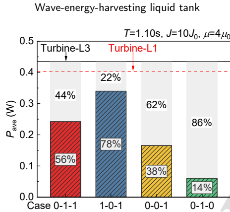
Figure 27: Capability loss of Turbine-L3 in different failure cases
