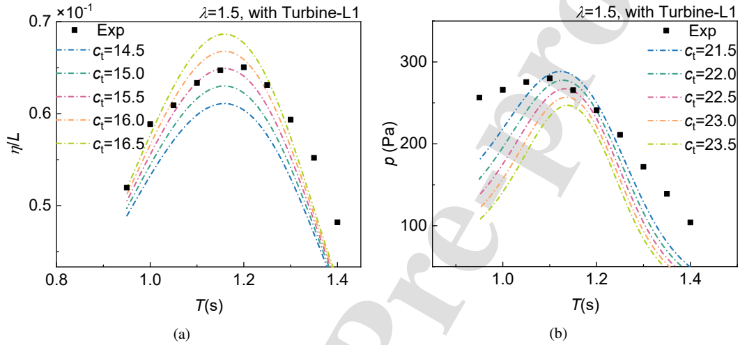
Figure 12: Comparison between theoretical and experimental results with Turbine-L1, for (a) free-surface amplitude; and (b) air pressure
