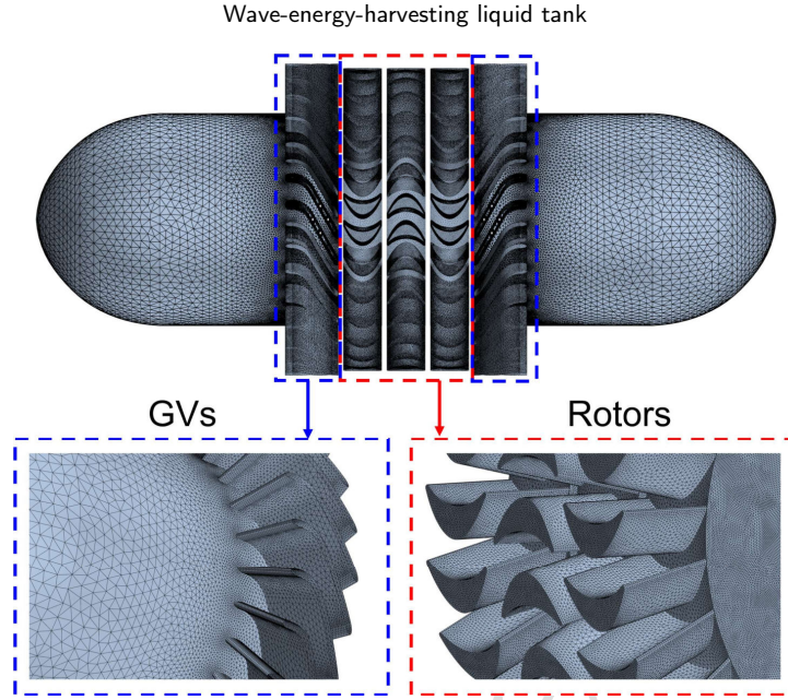
Figure 9: Surface mesh of multi-layered air turbine system
