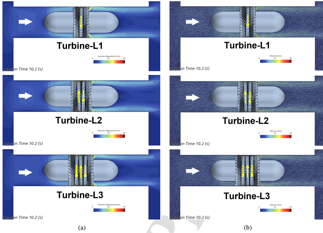
Figure 24: (a) Amplitude distribution and (b) vector field of air-flow velocity near the turbine system, in excitation condition of T = 1.10s
