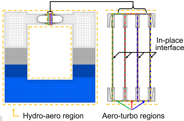
Figure 8: Illustration of hydro-aero and aero-turbo regions and zoomed-in view of aero-turbo regions
