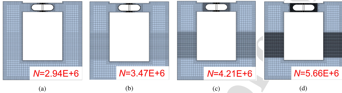
Figure 13: Mesh models for spatial convergence study: (a) mesh-1; (b) mesh-2; (c) mesh-3; and (d) mesh-4
