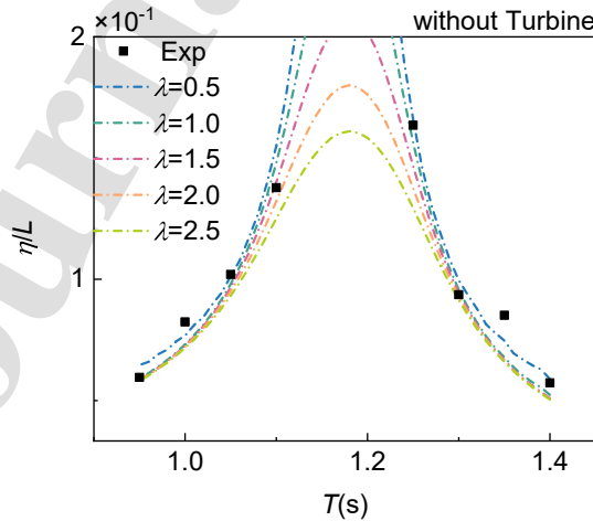
Figure 11: Comparison between theoretical and experimental results with Turbine-L1 for free-surface amplitude
