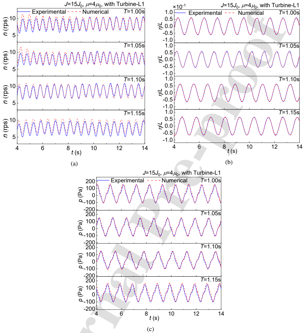
Figure 17: (a) Validation of rotor speed (b) validation of liquid surface displacement; (c) validation of pressure
