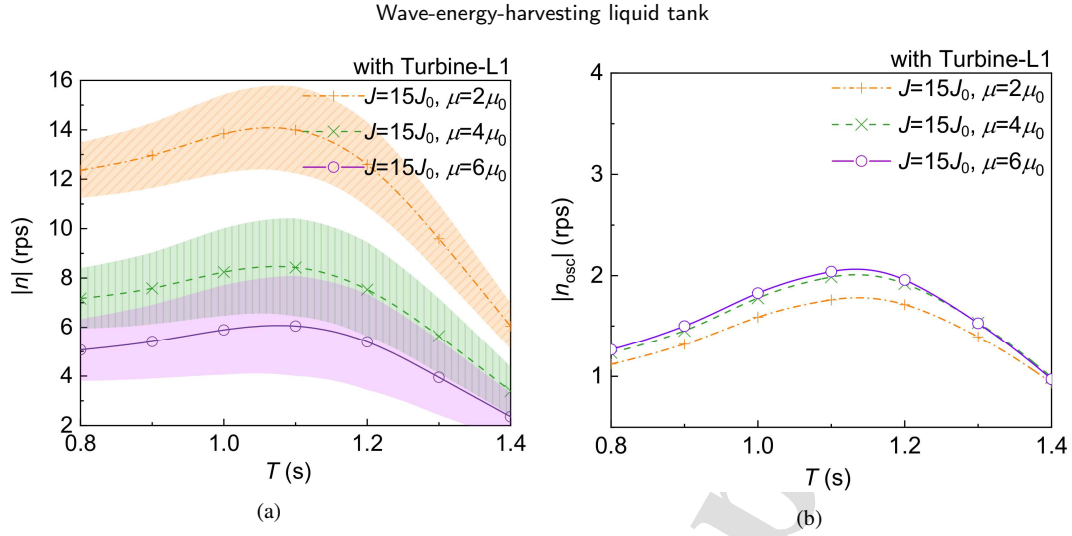
Figure 20: Effect of damping coefficient on rotor speed: (a) averaged rotor speed and speed limits; (b) variation range of rotor speed
