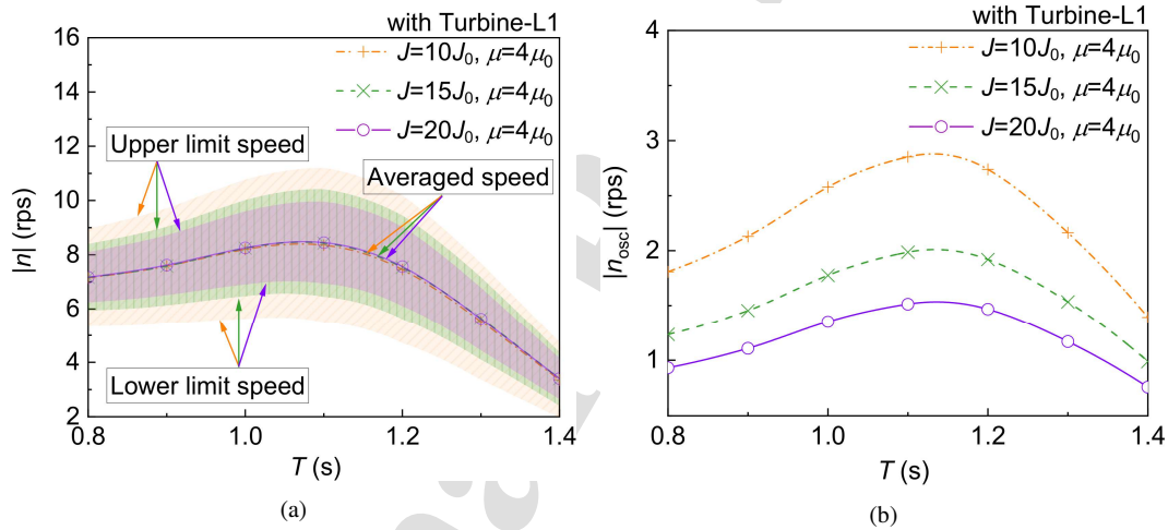
Figure 19: Effect of moment of inertia on rotor speed: (a) averaged rotor speed and speed limits; (b) variation range of rotor speed
