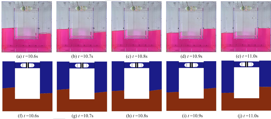
Figure 16: Comparison of experimental snapshots at t = (a) 10.6s, (b) 10.7s, (c) 10.8s, (d) 10.9s, and (e) 11.0s with numerical results at t = (f) 10.6s, (g) 10.7s, (h) 10.8s, (i) 10.9s, and (j) 11.0s, for wave-energy-harvesting tank with Turbine-L1 in excitation condition of T=1.10s
