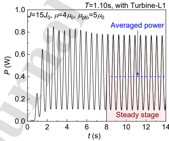
Figure 21: History of generated power of wave-energy-harvesting liquid tank
