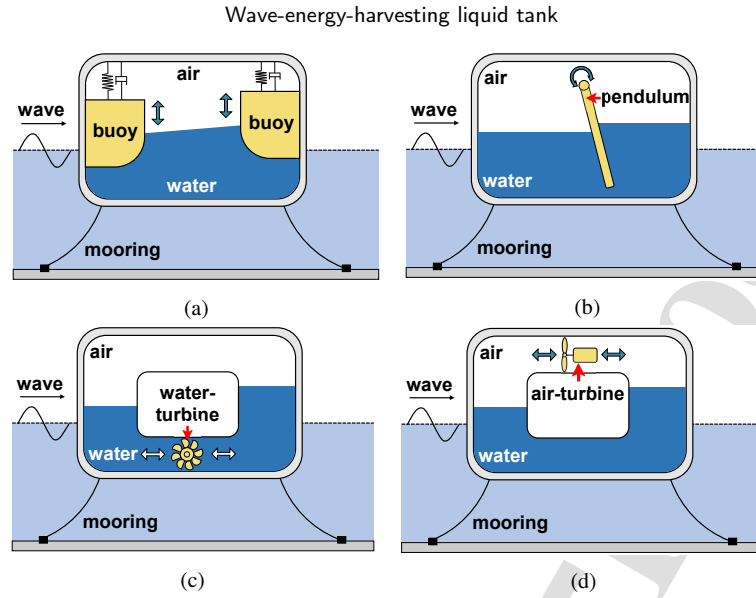
Figure 3: Mechanical principle of liquid-tank En-WEC with (a) buoy system [36]; (b) pendulum system; (c) water-turbine system; and (d) air-turbine system
