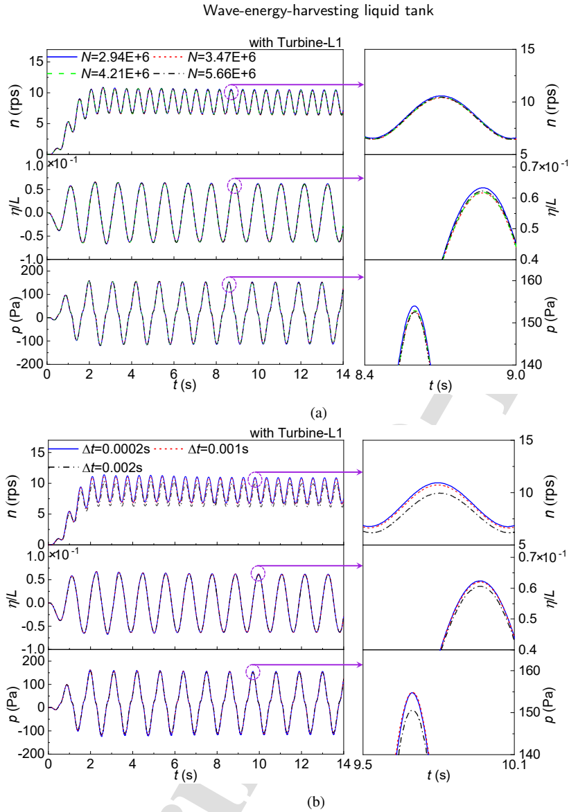
Figure 14: Convergence study for (a) mesh discretization, and (b) time step
