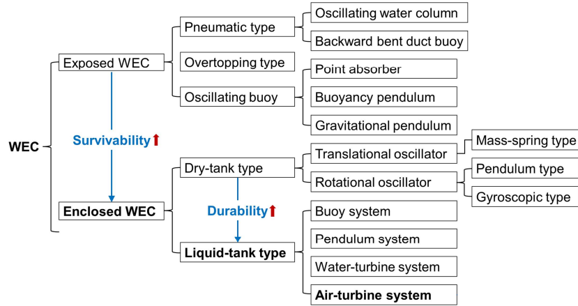
Figure 1: Classification of working principles of wave energy converters
