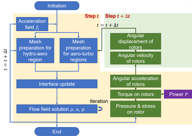
Figure 10: Flow chart of integrated numerical model for coupled hydro-aero-turbo dynamics of wave-energy-harvesting liquid tank
