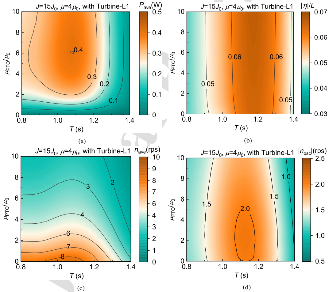
Figure 22: Effect of power take-off damping on (a) averaged power, (b) free-surface amplitude, (c) averaged rotor speed, and (d) variation range of rotor speed
