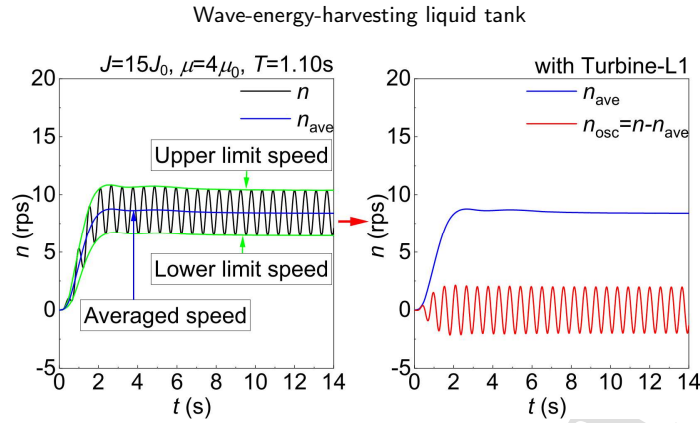
Figure 18: History of rotor speed and its decomposition
