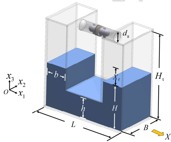
Figure 6: Illustration of wave-energy-harvesting liquid tank model
