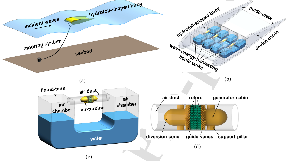
Figure 4: (a) External appearance of hydrofoil-shaped buoy; (b) concept of wave-energy-harvesting liquid tanks inside the buoy; (c) components of wave-energy-harvesting liquid tank; (d) components of multi-layered impulse air-turbine system
