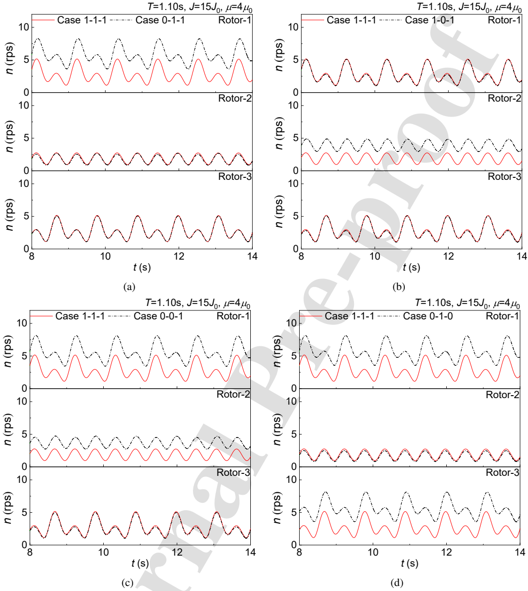
Figure 26: Rotor speed status of Turbine-L3, in failure cases of (a) 0-1-1, (b) 1-0-1, (c) 0-0-1, and (d) 0-1-0
