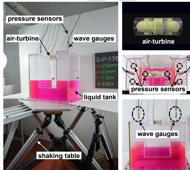
Figure 7: Scaled prototype of wave-energy-harvesting liquid tank and measurement system
