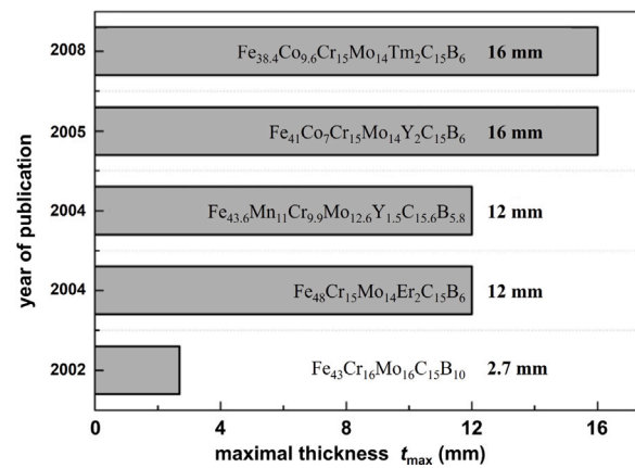
Fig. 3. Illustrative example of successfully increased of GFA (given in terms of the maximal casting thickness t_{\max} ) by compositional tuning of a family of Fe-based MGs with elevated-temperature resistance also called “amorphous steels” (adapted with permission from [158]). Optimisation for application in NF in this example would focus on the replacement of Mo, possibly by W, as has been done previously in case of crystalline steels [159].
