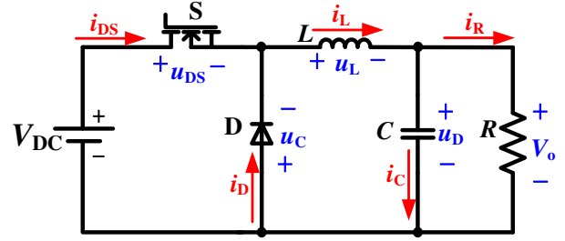
Fig. 13. The positive direction of voltage and current on each device.
