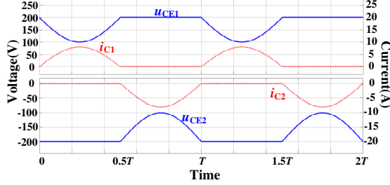
Fig. 4. The voltage and current waveforms on T 1 and T 2 under the Normal power supply mode.
