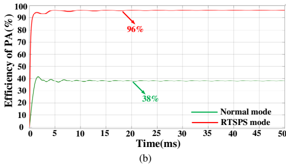
Fig. 16. Output power and efficiency comparison of PAs under normal power supply model. (a) Output power of each stage. (b) Comparison of PA efficiency under two models.
