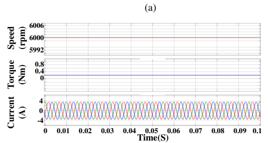
Fig. 19. Simulation results with PA drive system. (a) 30rpm. (b) 6000rpm.
