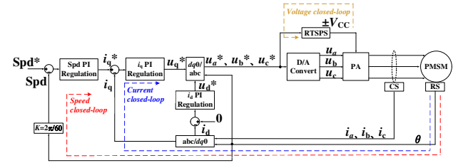
Fig. 18. The control structure block diagram of the motor drive system based on PAs and RTSPSs.
