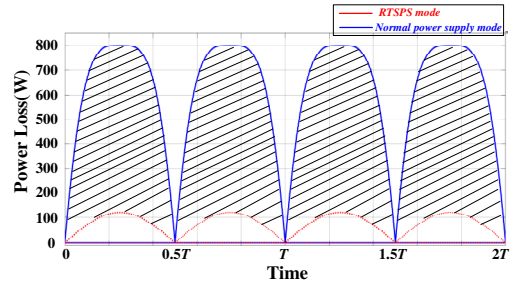
Fig. 7. Losses comparison of PA between two modes.
