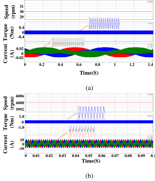
Fig. 20. Simulation results with SVPWM drive system. (a) 30rpm. (b) 6000rpm.
