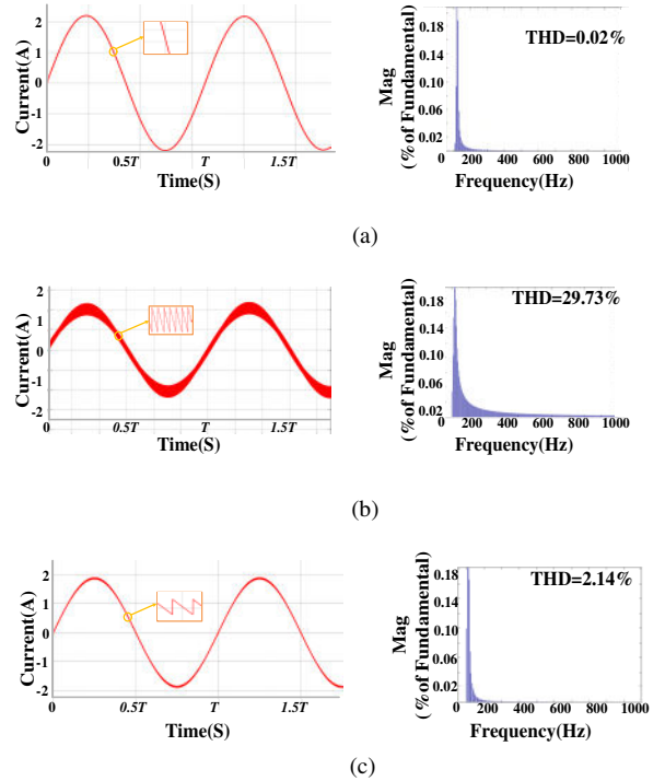
Fig. 21. Stator current and its THD in different mode. (a) PA drive system. (b) SVPWM drive system. (c) SVPWM drive system with filter.
