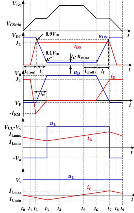
Fig. 14. The voltage and current waveforms of each device.
