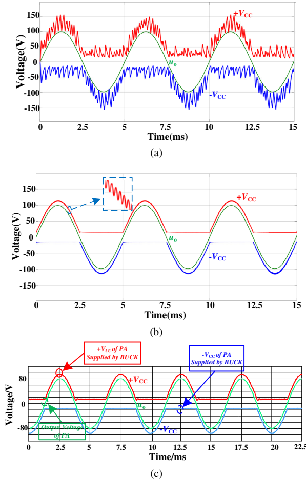
Fig. 11. Output of RTSPSs. (a) f_s=15\text{kHz} . (b) f_s=100\text{kHz} . (c) The experimental waveforms: f_s=100\text{kHz}
