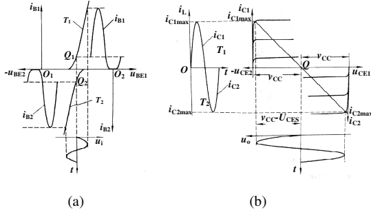
Fig. 2. Working principle of the OCL. (a) The input features of the T_1 and T_2 transistors under u_i . (b) The waveform analysis diagram of the OCL power amplifier circuit.
