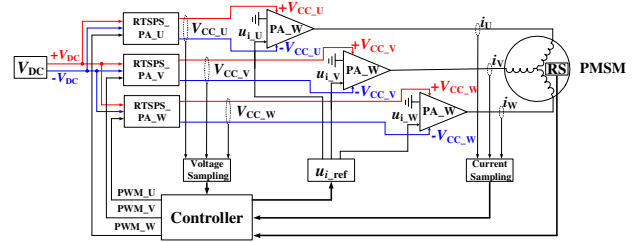
Fig. 17. The PMSM drive topology based on PAs and the RTSPSs.
