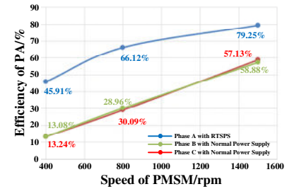
Fig. 29. Comparison of PA efficiency with different speeds.
