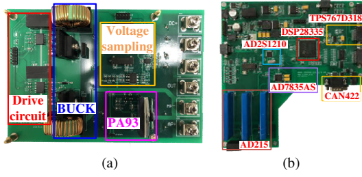
Fig. 22. The designed PCB. (a) RTSPSs PCB. (b) Controller PCB based on DSP28335.
