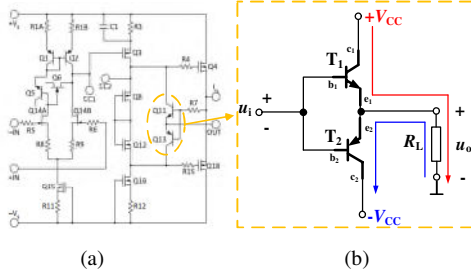
Fig. 1. OCL power amplifier circuit. (a) Internal structure. (b) Simplified structure.
