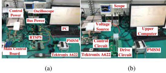
Fig. 23. The PMSM drive experimental platform. (a) Based on PAs and RTSPSs. (b) Based on traditional SVPWM.
