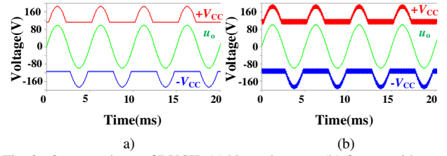
Fig. 8. Output voltage of BUCK. (a) Normal output. (b) Output with harmonics.
