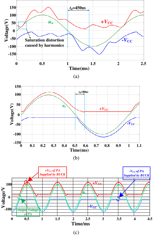
Fig. 12. Comparison of RTSPSs simulation. (a) f_s=15\text{kHz} . (b) f_s=100\text{kHz} . (c) The experimental waveforms: f_s=100\text{kHz}
