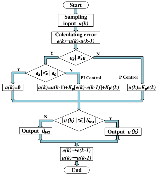
Fig. 24. Flow chart of PI regulator algorithm.
