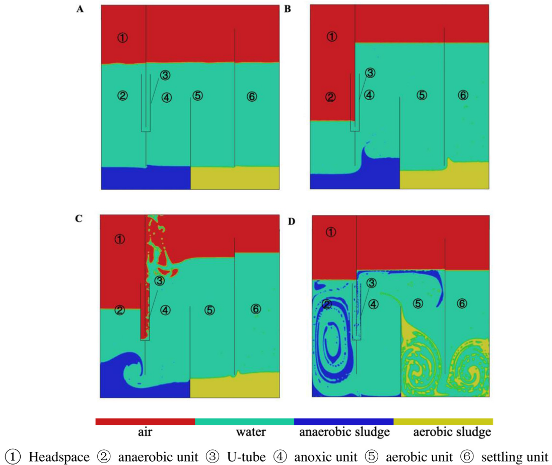
Fig. 4. CFD simulation for a laboratory-scale system (13 L) for the mixing status of the fluid during one cycle of pneumatic agitation. (A) the original state, (B) air is pressurized to push the fluid level down and the anaerobic sludge to the anoxic unit, (C) the fluid level reaches the bottom position of the U-tube, the pressurized air is released from the anaerobic headspace to the anoxic unit through the U-tube and the fluid is flushed back from the anoxic unit to the anaerobic unit through the bottom channel, and (D) the anaerobic fluid level is raised to its original state and the fluid in the reactor is mixed up to a certain extent. The timeframe for one cycle of agitation is set as 2.5 min.
