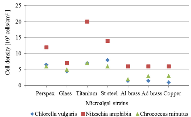
Fig. 4. Growth of Chlorella vulgaris , Nitzschia amphibia , and Chroococcus minutus on different materials. Data taken from study conducted by Sekar in 2004 [73].
