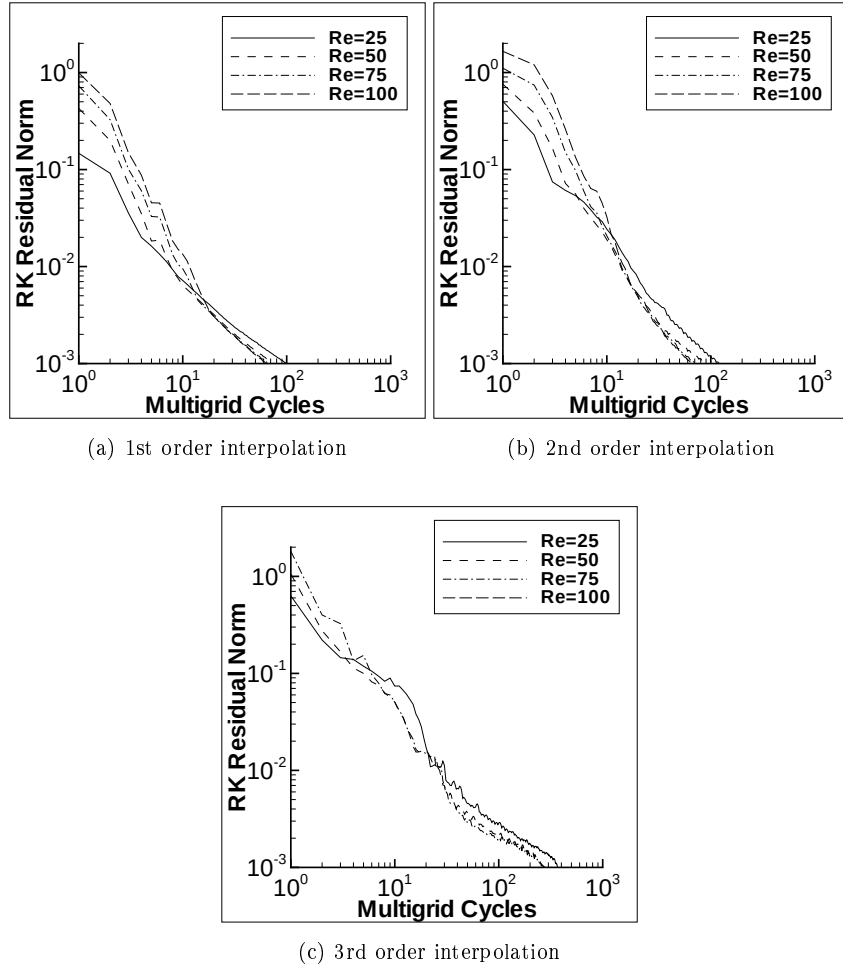
Figure 15: Dependence of multigrid convergence on the Reynolds number for the diffusion broadening problem.
