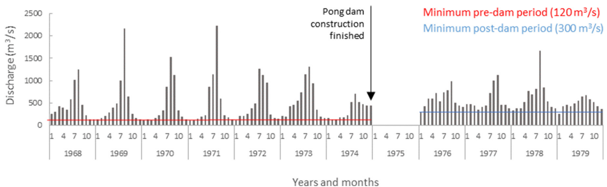
Fig. 3. Monthly average river discharge of Beas River at Mandi (Fig. 2) derived from the Global Monthly River Discharge Data Set (Vorosmarty et al., 1998).
