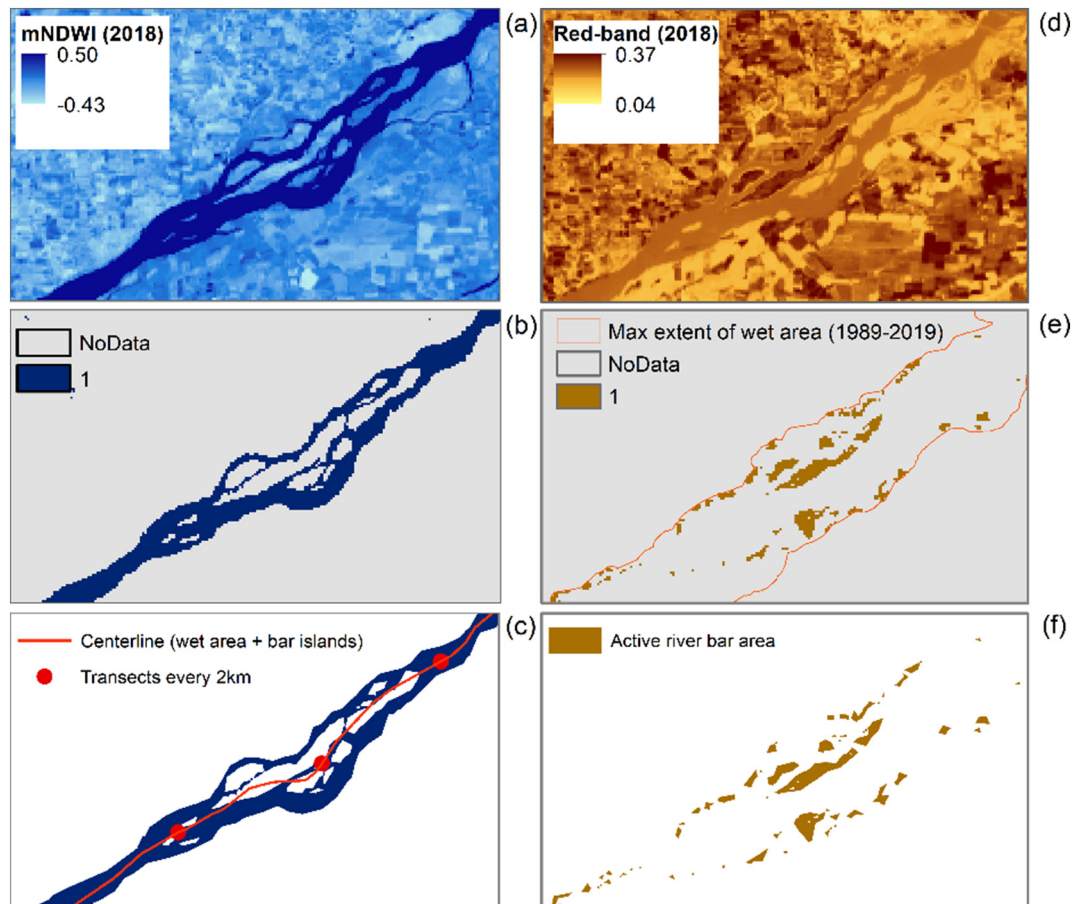
Fig. 4. Extraction of the wet river area and active gravel bars using remote sensing: (a) Landsat mNDWI imagery, (b) reclassification of mNDWI values (>0.15: water, rest: no data), (c) conversion from raster to wet river area polygon, (d) Landsat visible red imagery, (e) reclassification of reflectance values (>0.16: gravel bars, rest: no data) within a buffer defined by the maximal extent of all wet area polygons between 1989 and 2019, (f) conversion from raster to active gravel bar polygons.
