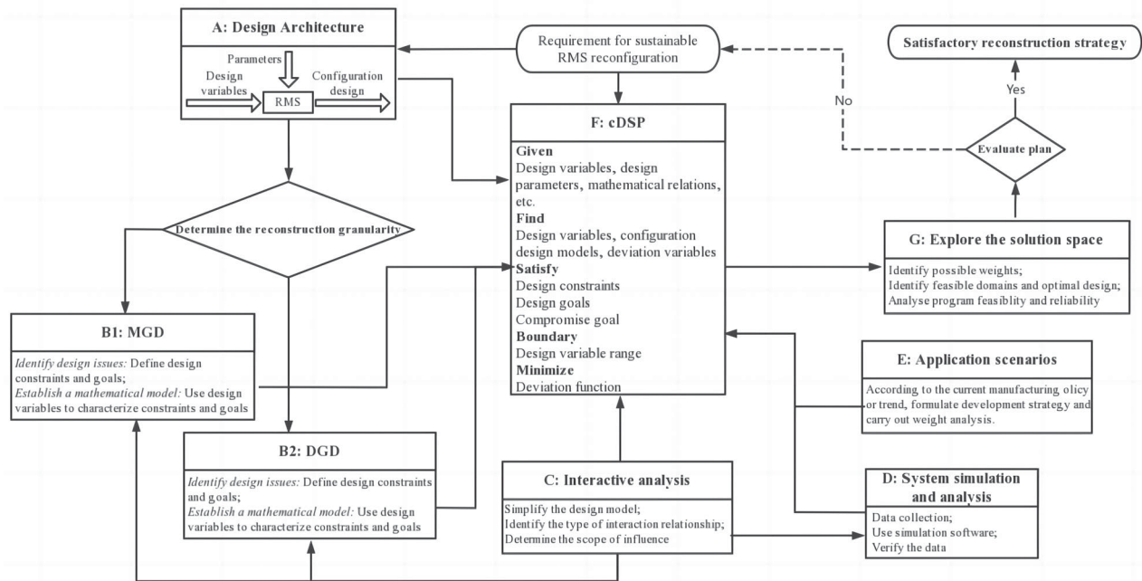
Figure 7. Decision network for exploring the sustainable RMS reconfiguration strategy.
