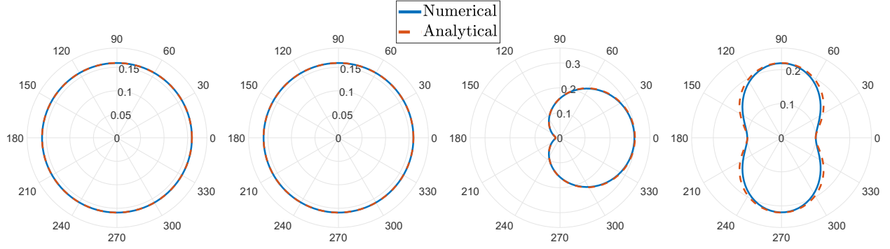
Fig. 6 Comparison of the analytical and numerical calculation of the integral in Equation 27 for four different directivity functions of which the coefficients from left to right are: A_\ell^m = [1 \ 0 \ 0 \ 0] , A_\ell^m = [0 \ 0 \ 0 \ 1] , A_\ell^m = [1 \ 1 \ 0 \ 0] , A_\ell^m = [1 \ 1 \ 1 \ 1] .
