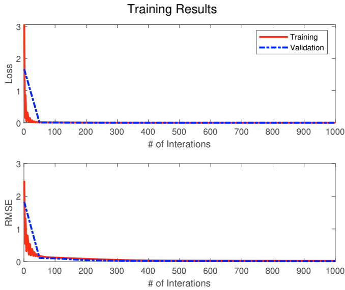
Fig. 7. Training Results for CNN-based Model
