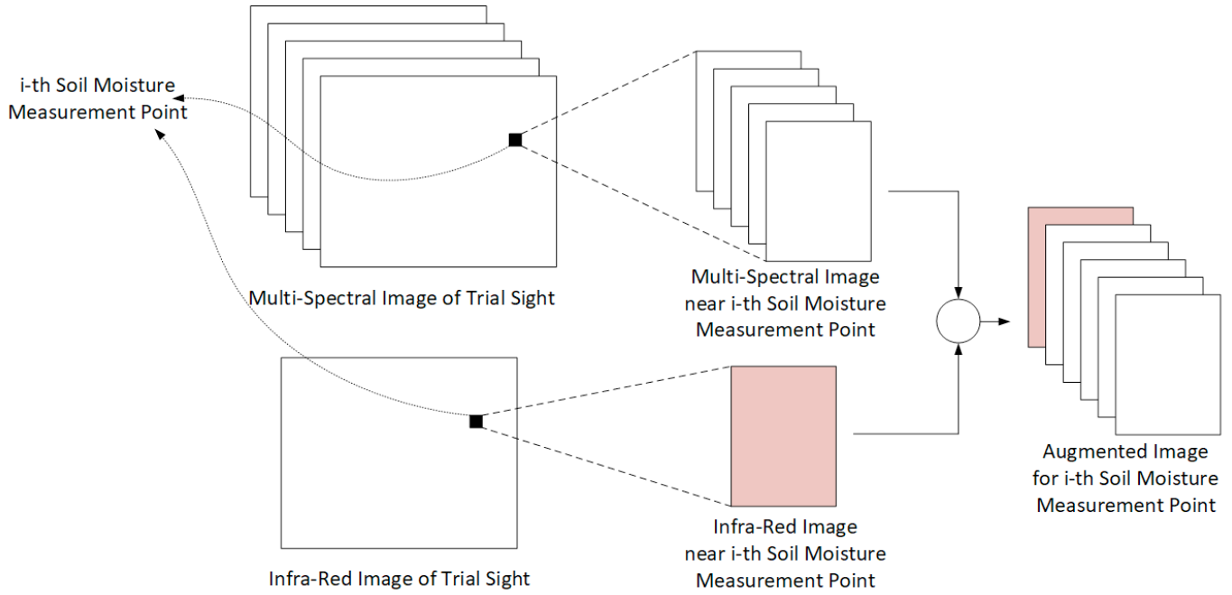
Fig. 4. Cropping and Stacking Images for Soil Moisture Measurement Point
