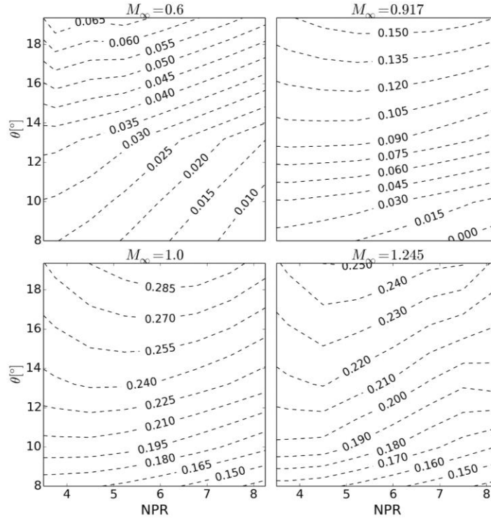
Fig. 13: C_D iso lines – A_9/A_8=1.2 \beta=10^\circ
