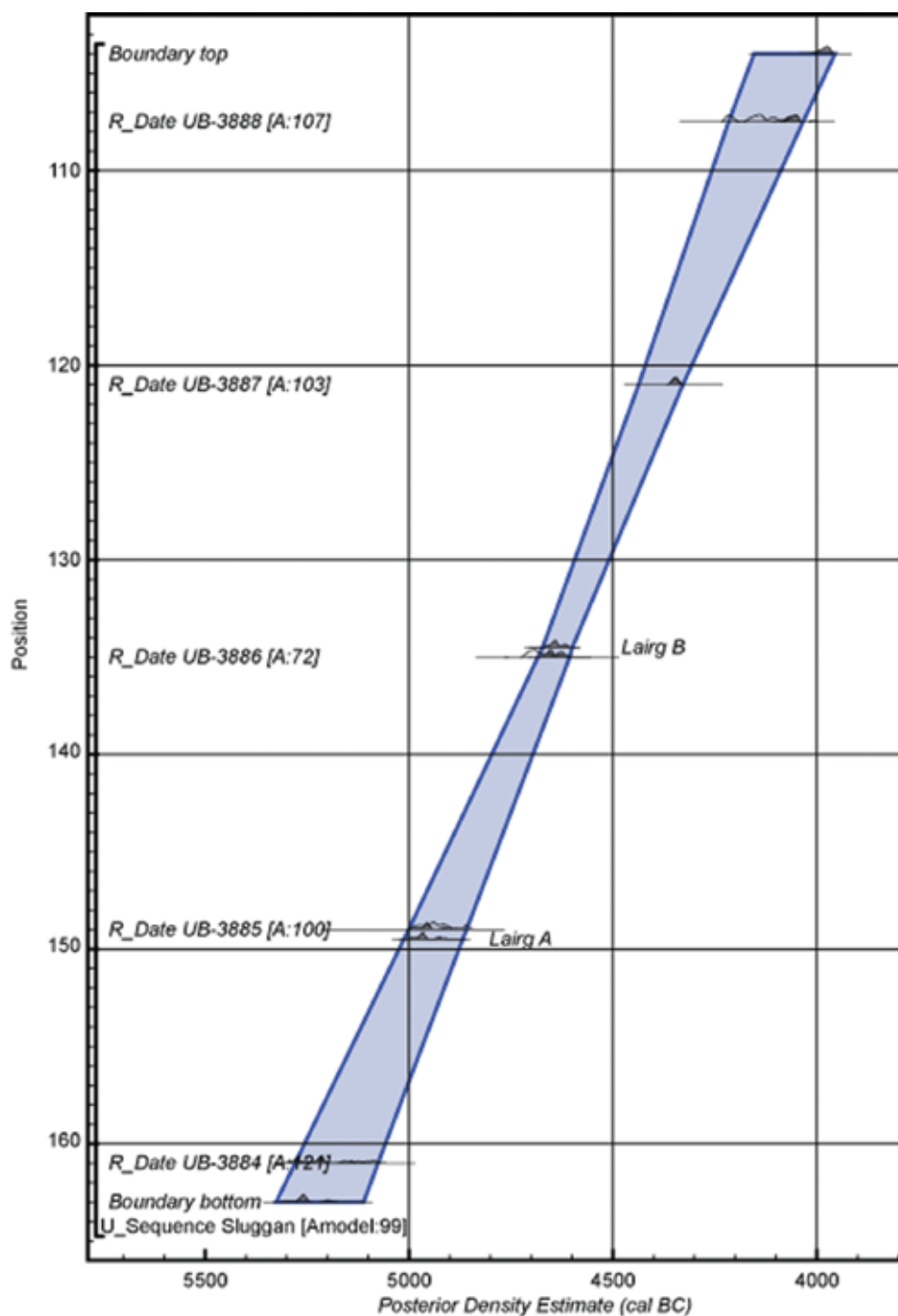
Figure 20.6: Bayesian age-depth model of the chronology of the sediment sequence at Sluggan Bog (U_Sequence model; Bronk Ramsey 2008) and estimates for the dates of the Lairg A and B tephra horizons. The coloured band shows the estimated date of the sediment at the corresponding depth, at 95% probability. For radiocarbon dates the lighter distribution is the result of simple calibration and the darker distribution is the posterior density estimate provided by the model.
