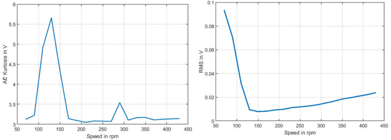
Figure 5: RMS and Kurtosis of pre-processed AE patterns for a speed ramp at a constant load.
