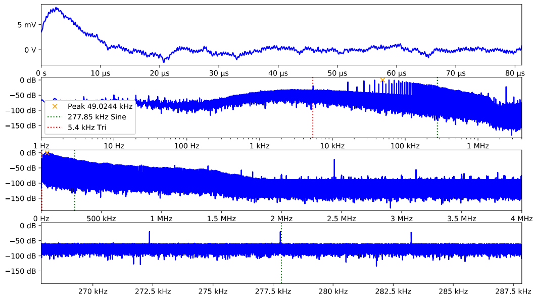
Figure 9: Test Result Subscale WDTU at 2200 min-1
