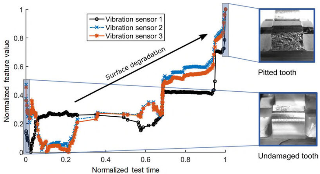
Figure 3: Pitting detection features
