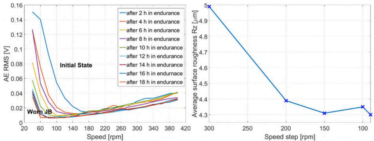
Figure 6: Degradation levels indicated by AE RMS for speed sweeps from 40 to 400 rpm, constant load of 1500 N (left). Average surface roughness over different speed steps (right).
