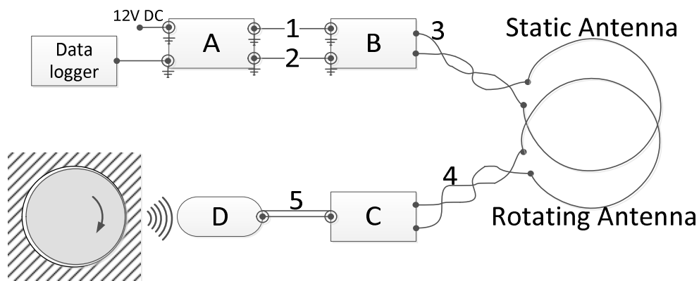
Figure 8: WDTU system overview.
